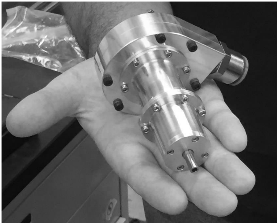
Figure 2 Assembled turbo-spindle
