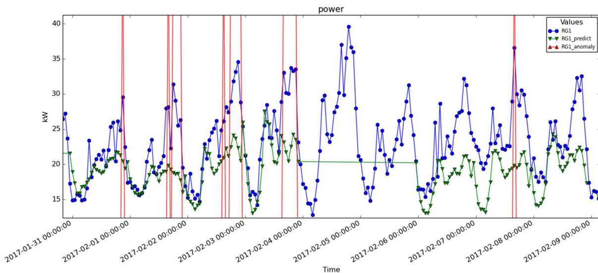
Figure 15 – Example of gap detection between predicted and actual values
