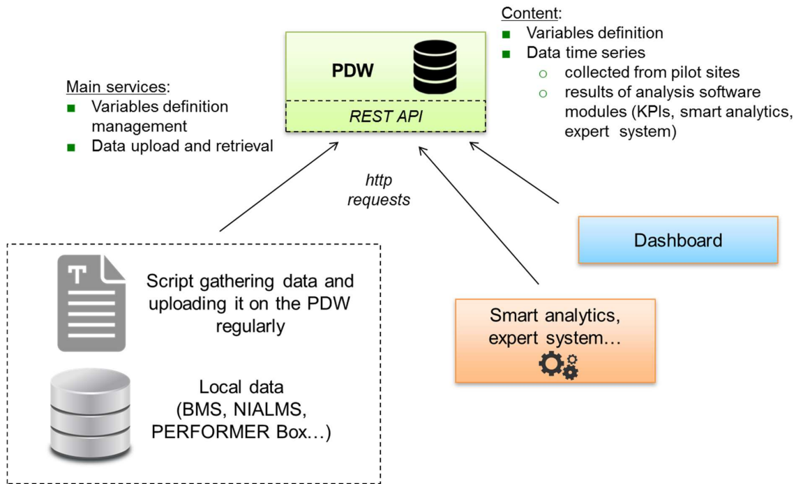
Figure 14 - Interoperability with the PERFORMER Data Warehouse
