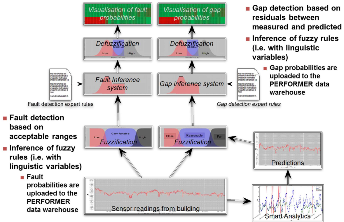
Figure 16 - Architecture of the expert system module
