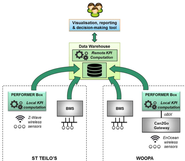
Figure 18 - Technical integration of a PERFORMER Box
