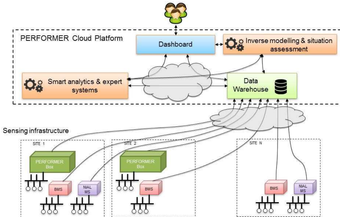
Figure 4 – ICT architecture of the PERFORMER solution
