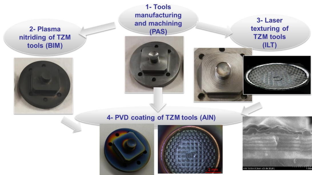
Fig. 10: Tool innovative production chain
