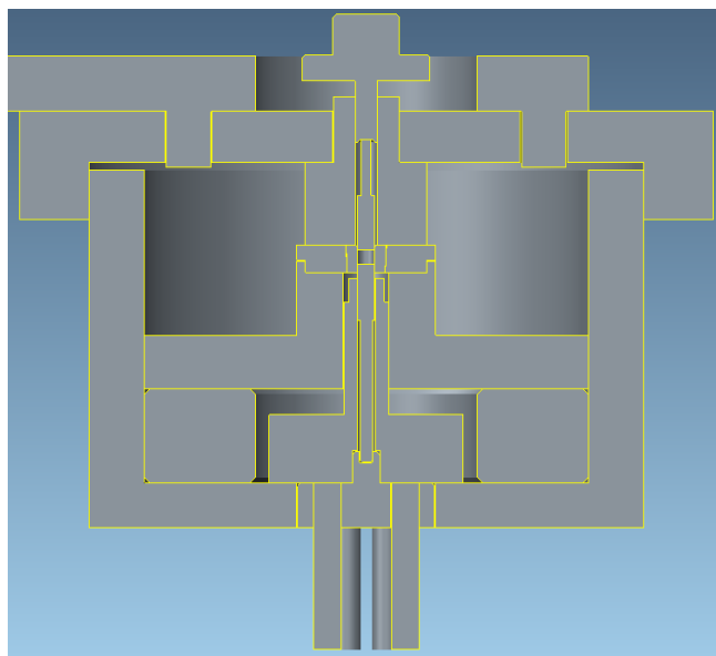
Fig. 27: Cross section of CAD model of the tool for compression and expanding the sintering die
