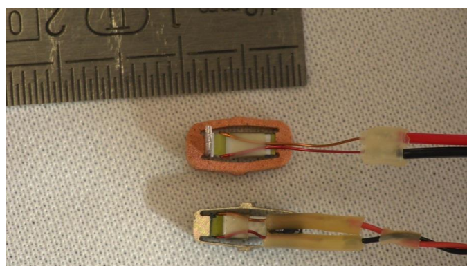
Fig. 24: Comparison between Micro-FAST actuator (top) and standard actuator (bottom)
