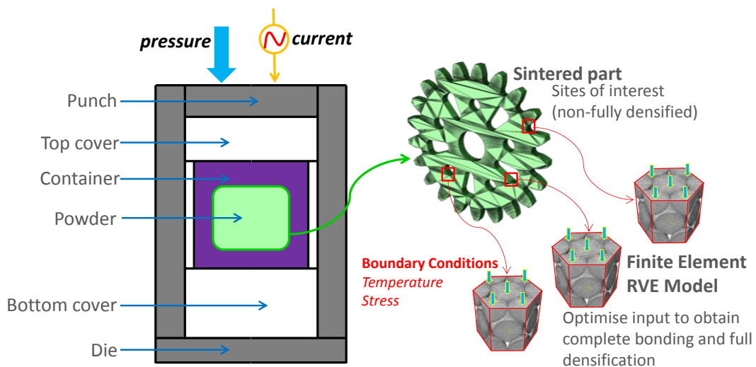
Fig. 8: Schematic of the multi-scale modelling of the sintering process
