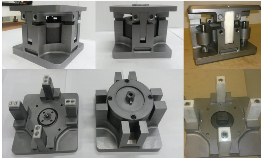
Fig. 9: Micro-FAST Forming Tools
