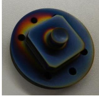
Fig. 13: TzM punch with plasma nitriding + PVD coating.
