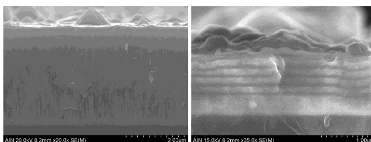
Fig. 12: Cross-section view of a CrAlSiN monolayer (left) and a CrAlOxN/CrAlN multilayer (right) coatings.
