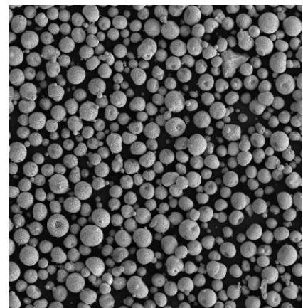
Fig. 6: Electron microscope image of the spraydried MSZ powder used in the micro-FAST trials.
