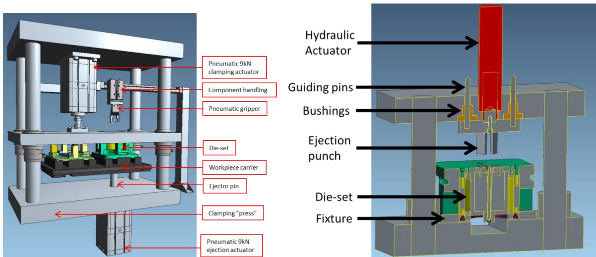
Fig. 19: CAD design for first automated system (left) and final manual concept (right)
