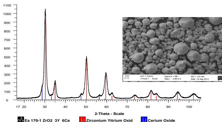
Fig. 7: Ce-YSZ nanopowders main characteristics (left), XRD and SEM of C-YSZ nanopowders (right)
