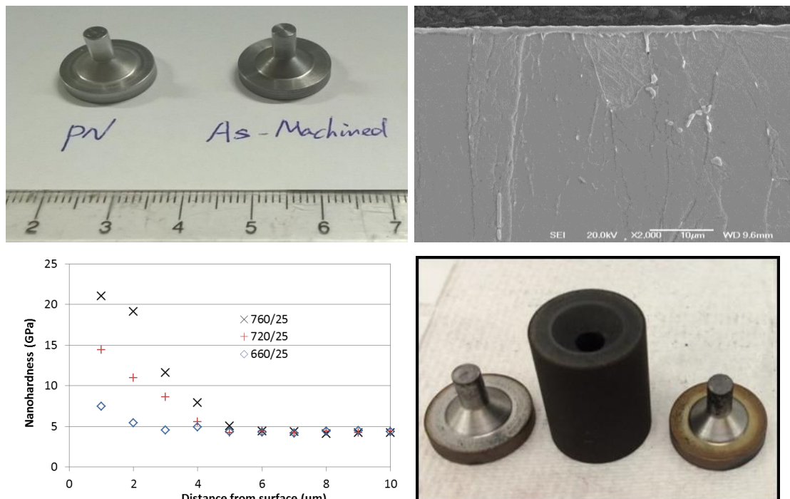
Fig. 11 (a) Comparison of as-machined and plasma nitriding treated TZM punches, (b) A cross-sectional view of plasma nitriding treated TZM sample (c) hardness profile under the nitride layer (d) Plasma nitrided punches after field test.
