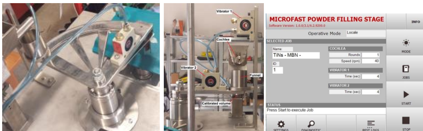
Fig. 17: Feeding system (left, middle) and software control (right).
