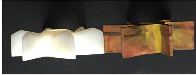
Fig. 21: Product to process adaptation: conventional geometry vs simplified design
