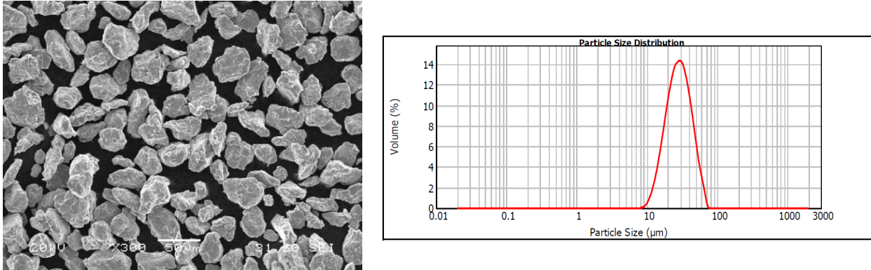
Fig.5 SEM morphology (left) and PSD (right) of Ti-alloy powder produced by HEBM
