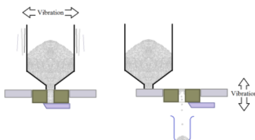
Fig. 16: Working principle of powder feeding
