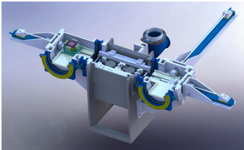
Fig. 2 Sectional view of design of handling system
