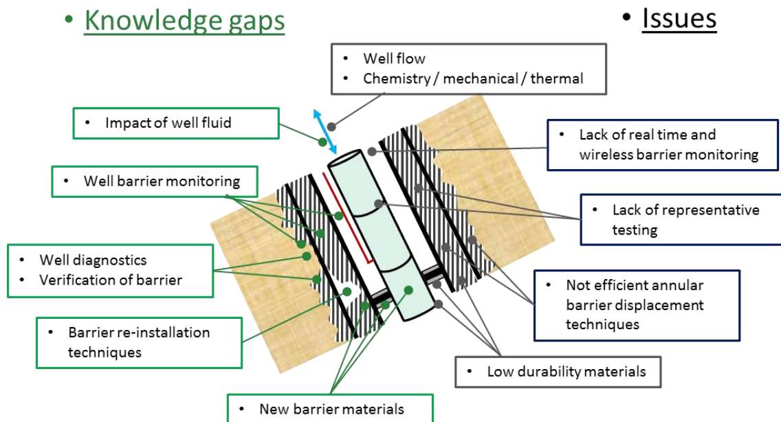
Figure 15: Schematics of an operating CO 2 well showing knowledge gaps and issues.
