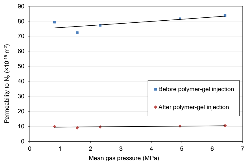
Figure 13: Changes in wellbore cement fracture permeability to N 2 , with mean gas pressure, before and after polymer-gel treatment.
