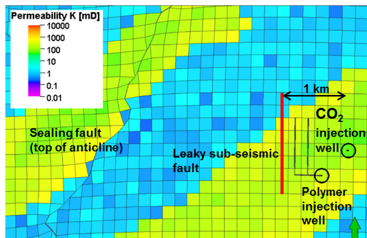
Figure 7: Location of polymer injection well, sub-seismic fault and CO 2 injection well.
