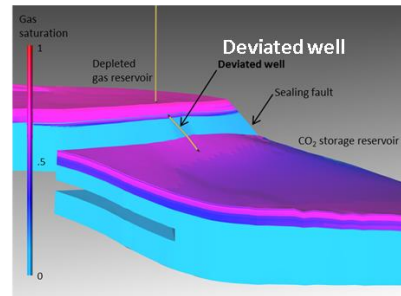
Figure 5. Breaching of fault seal by hydraulic fracturing (left) and drilling a deviated well (right) to enable lateral migration of fluids between the two adjacent reservoirs separated by a sealing fault.
