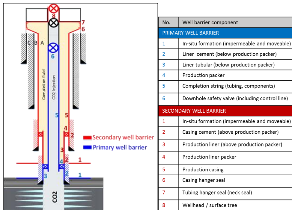
Figure 10: Well barrier elements for a typical CO 2 injection well.
