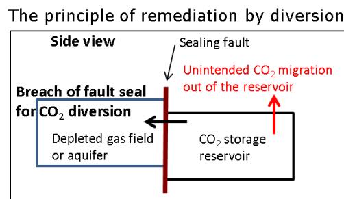
Figure 4. The principle of remediation by flow diversion from the CO 2 storage reservoir to the adjacent unconnected reservoir. Hydraulic connection between the two reservoirs separated by a sealing fault could be achieved by drilling a deviated well or by creating hydraulic fractures through the fault seal.
