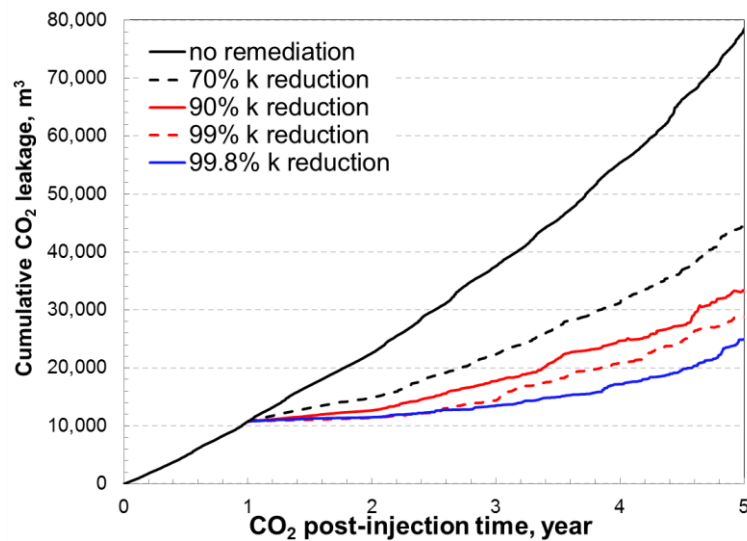
Figure 14: Simulated leakage profiles with and without polymer-gel treatment, and for varying effective fracture permeability reduction.
