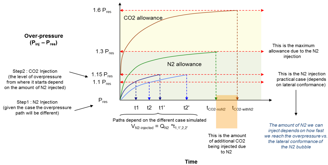
Figure 9: Conceptual design of an N 2 injection prior to a CO 2 injection.
