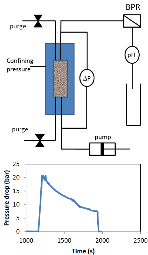
Figure 11. Simplified schematic of the experimental set-up for testing strength of reactive solution in porous media. As shown in the lower panel, a differential pressure of 20 bar was needed to displace brine through the sample, which in this case was 3 cm long.
