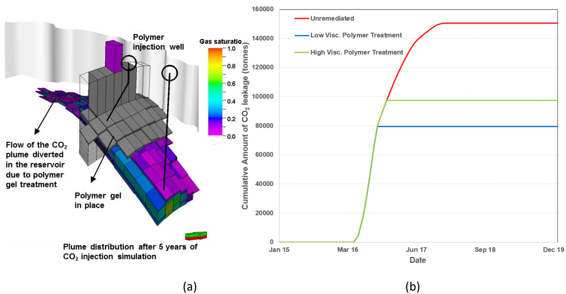
Figure 8: The results of numerical simulations for Scenario 1 in Table 1 (a) CO 2 plume distribution after 5 years of post-remediation CO 2 injections, (b) performance comparison of remediation measures for cases of unremediated leakage, low and high viscosity polymer-gel treatments.
