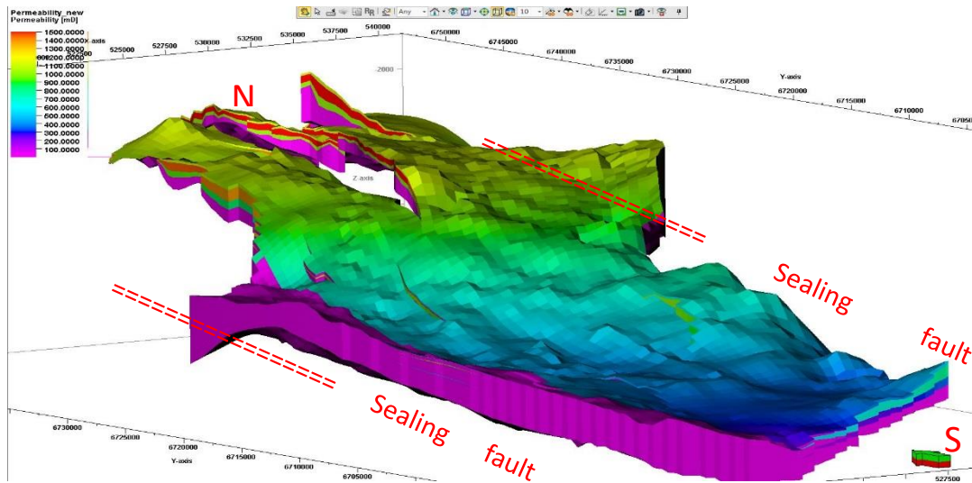
Figure 1: The Johansen model used in SINTEF's part of the study. A ridge-structure in the north-western part of this model was used to represent the undesired CO 2 migration path.
