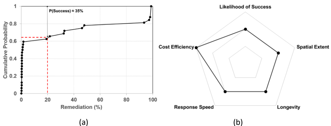
Figure 16: Brine/water injection technique: (a) success probability; (b) spider chart
