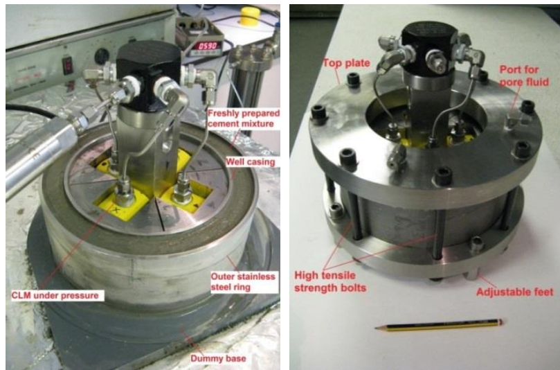
Figure 12: The wellbore cell of Imperial College. A central loading mechanism is used to generate varying mechanical load on the inner cylinder and induce fractures after cement curing.
