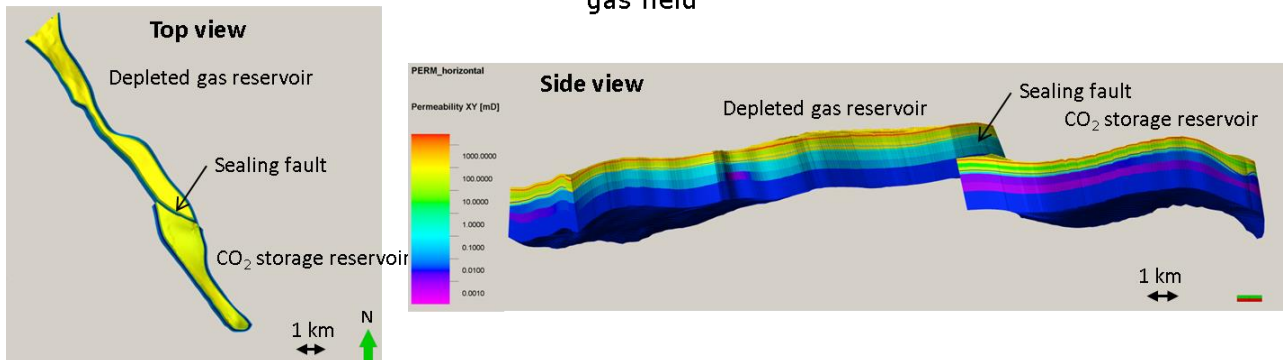
Figure 6. Top view (left) and side view (right) of the real case model used to simulate remediation by flow diversion from the CO 2 storage reservoir to the adjacent depleted gas reservoir.
