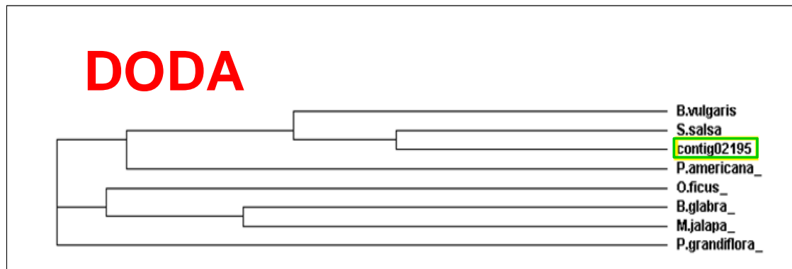
Figure 1.5.3. Phylogenetic analysis of the partial cDNA sequence of DOPA-4, 5-dioxygenase (DODA) obtained from the partial transcriptome sequencing of A. hypochondriacus cv. Revancha (contig 02195) as compared to sequences of known DODA genes in related species such as: Beta vulgaris , Suaeda salsa , Portulaca americana , Opuntia ficus-indica , Beta vulgaris var. glabra , Mirabilis jalapa and Portulaca grandiflora .
