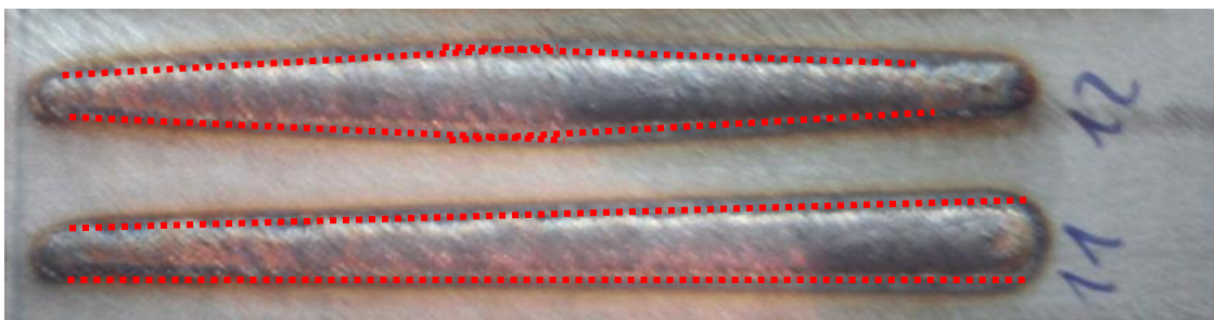
Figure 19. Different variable cladding tracks defined for the laboratory validation of the ALAS prototype.
