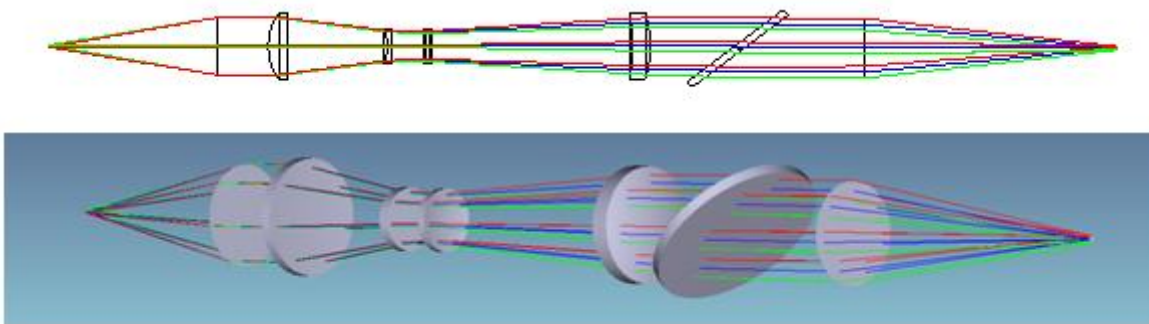
Figure 5. Simulation of optical system
