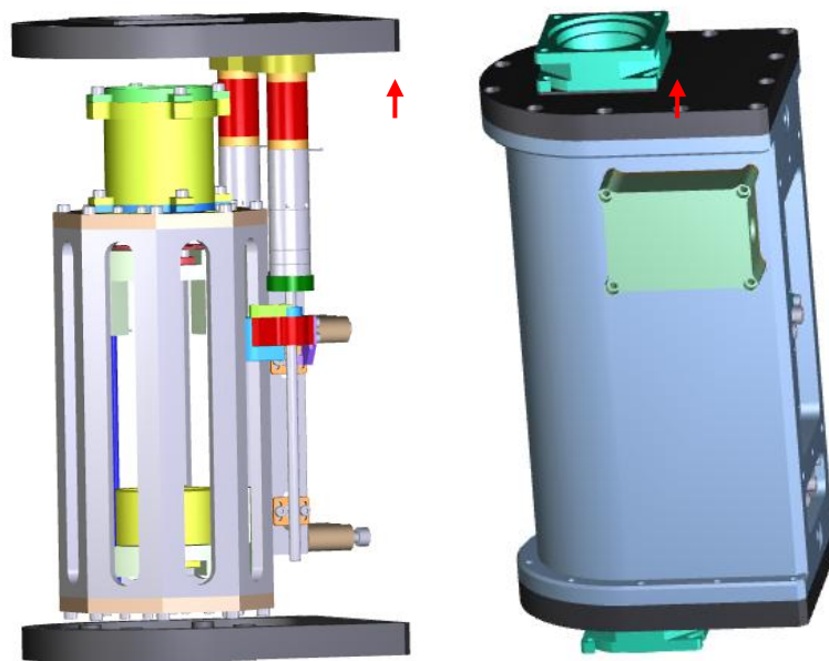
Figure 13. Scheme 3D of the ALAS prototype, interior and exterior of it.
