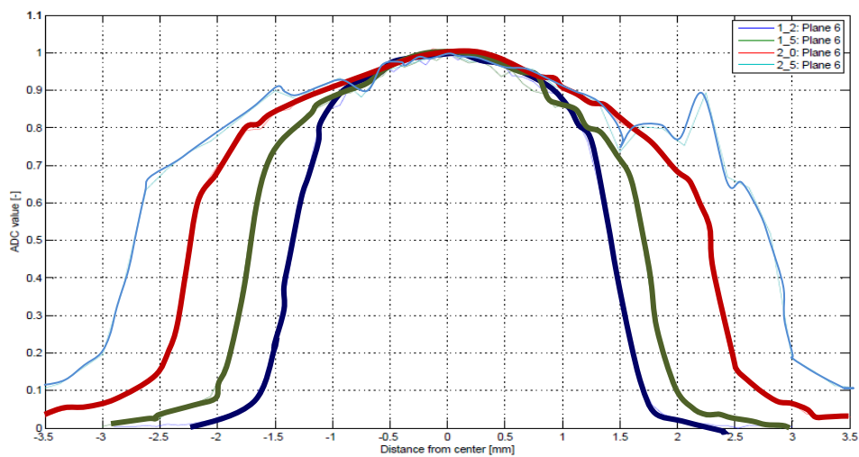
Figure 17. Cross-section of the beam size in all the magnification range.
