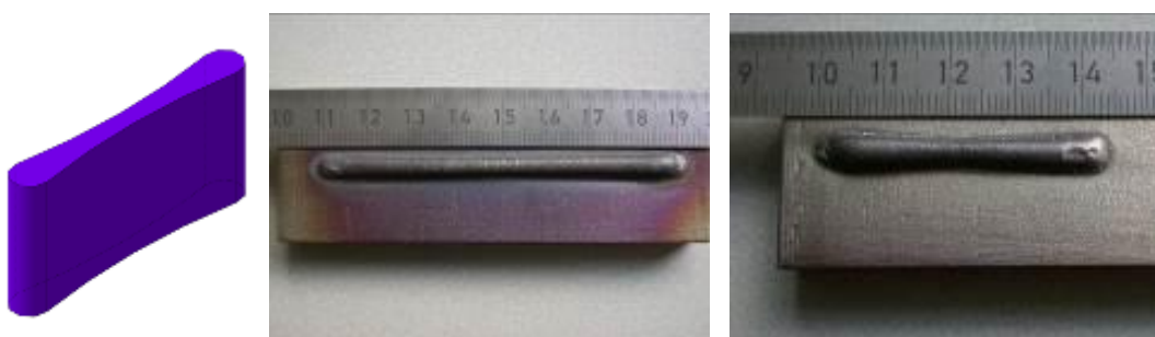
Figure 25. Left: digital drawing of hourglass shape. Middle: produced hourglass sample 2 of 80mm length, Right: produced hourglass sample 3 of 40mm length shape.
