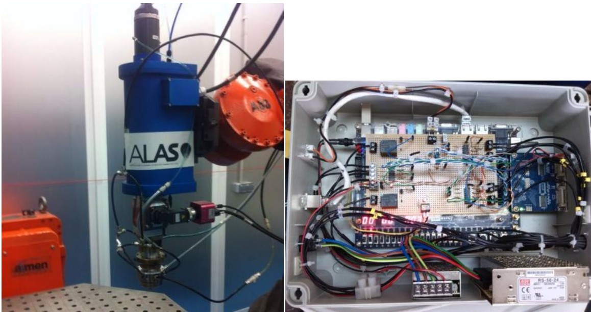
Figure 14. Final ALAS head prototype.
