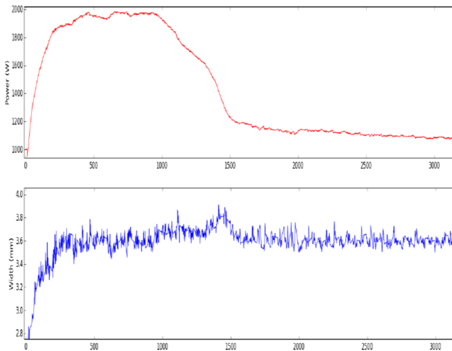
Figure 23. View on measured melt pool sizes during laser cladding process and their relation to the target width. Upon progress of the laser cladding process, a constant melt pool size is generated due to decrease of laser power.
