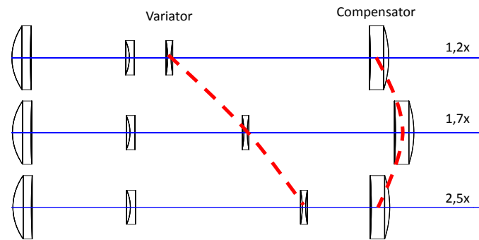
Figure 12. Synchronization of the movement of the movable lens.
