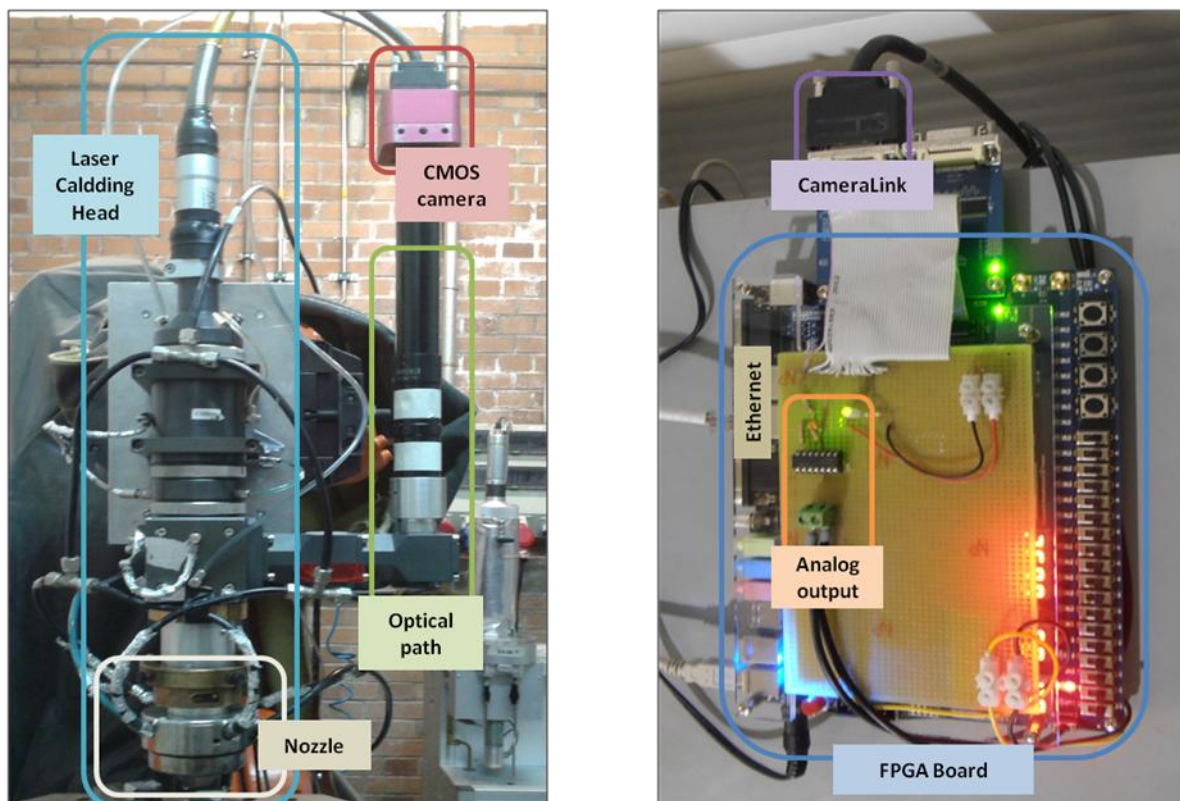
Figure 11 Testing laser cladding head and prototype of ALAS controller , b) FPGA hardware prototype of the ALAS controller.
