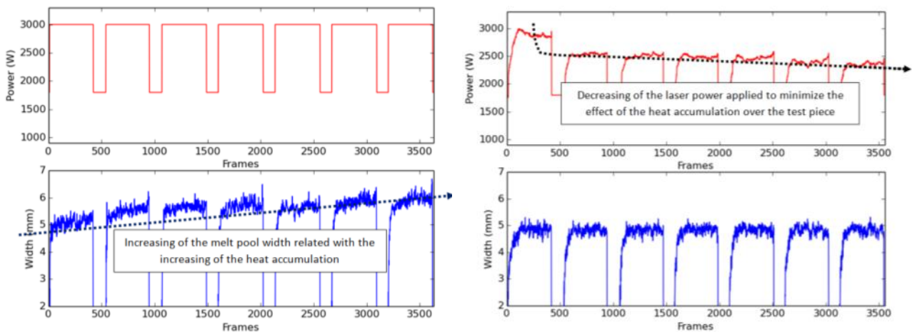
Figure 20. Comparison of applying a constant laser power value and a power control strategy to deal with the heat accumulation effect.
