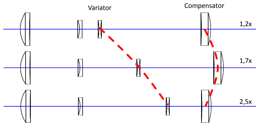
Figure 6. Scheme of lenses path on optical zoom system.
