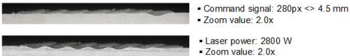
Figure 21. Metallographic comparison between close-loop control and a fixed laser power command.
