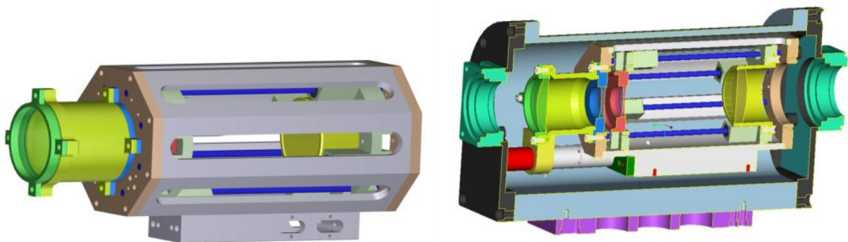
Figure 7. Octagonal monoblock. Sectional view of the Zoom Module.
