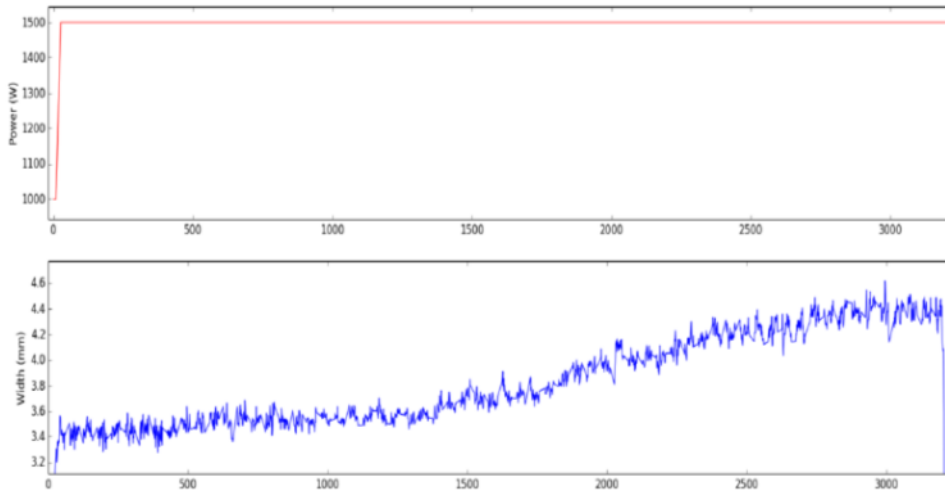
Figure 22. View on measured melt pool sizes during laser cladding process and their relation to the target width. Upon progress of the laser cladding process, a higher melt pool size is generated due to heat accumulation in the steel sample.
