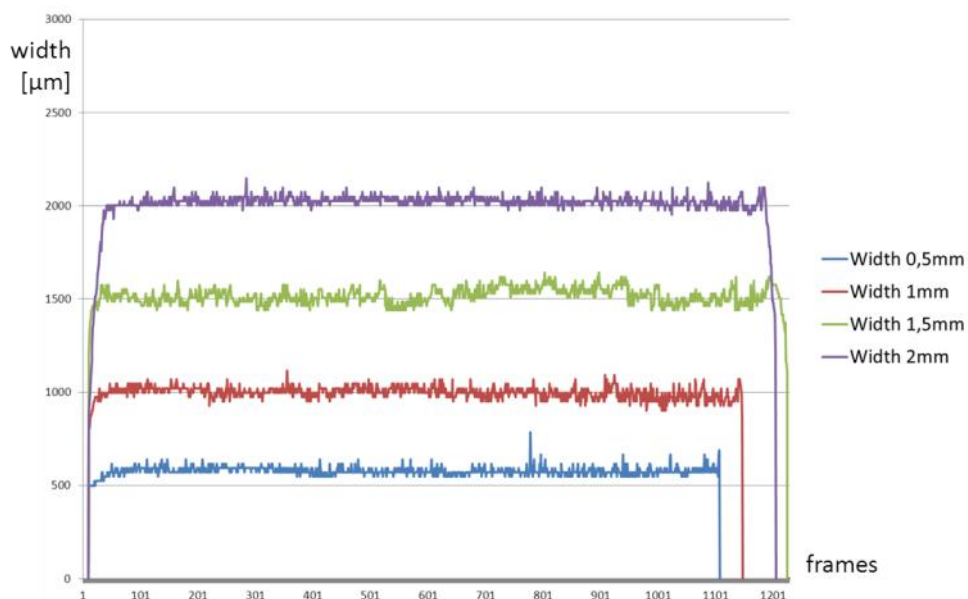
Figure 10 Signals of melt pool width.
