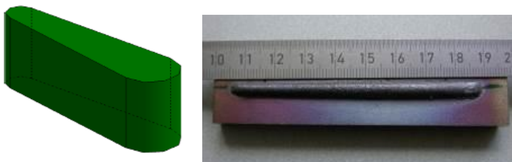
Figure 24. Left: digital drawing of right samples. Right: Picture of complex shape of sample 1, so-called big-small shape.
