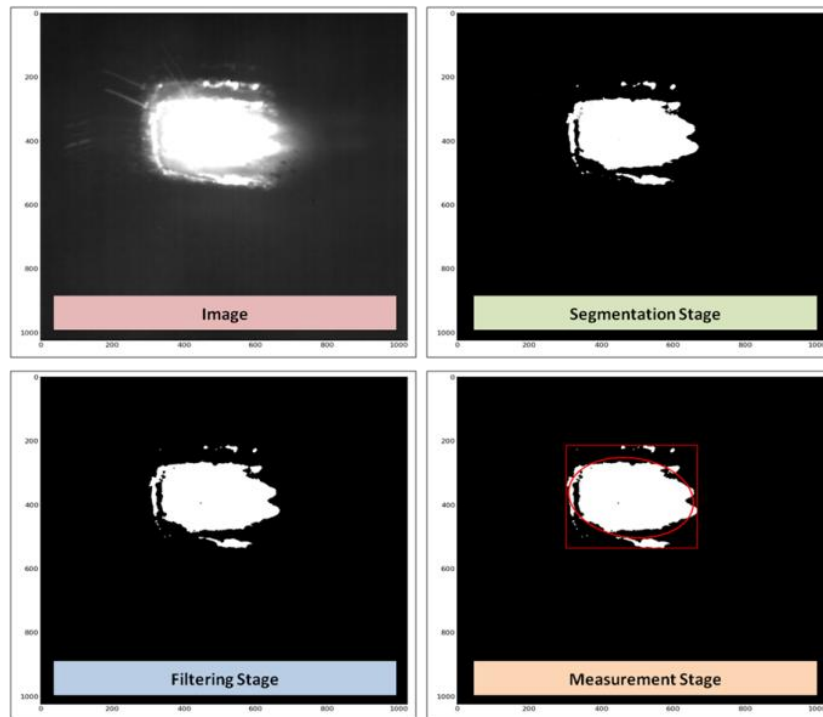
Figure 9. Image processing algorithm implemented in the FPGA controller.
