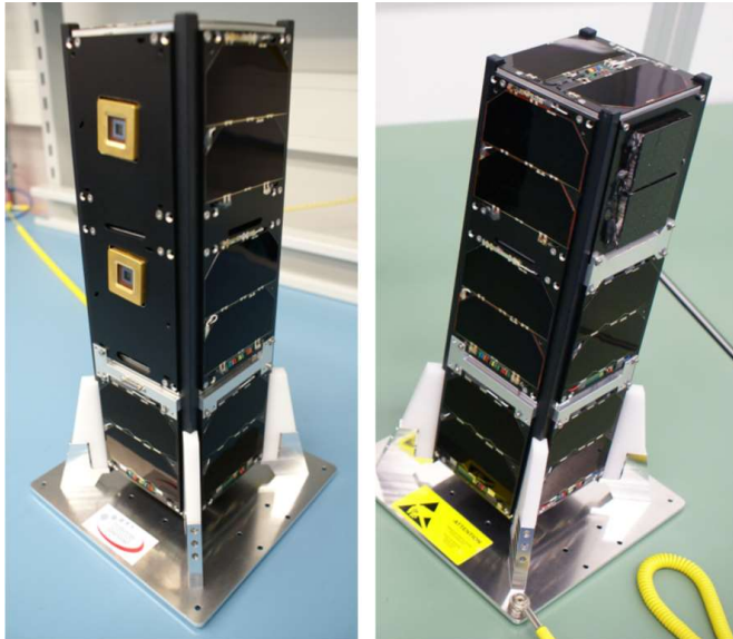
Figure 5, flight ready PEASSS satellite with visible in the left picture the 2 sun-sensors and in the right picture the 2 black pyro power generator elements
