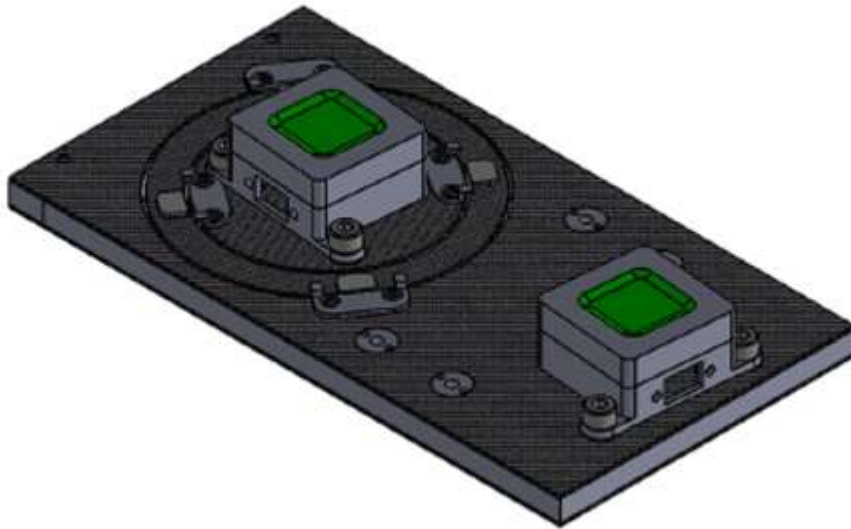
Figure 1, Design drawing of the Smart Structure with a fixed sun-sensor and a second sun-sensor mounted on a gimballed structure that can be tilted by means of 2 piezo bimorph actuators located at the back side of the panel
