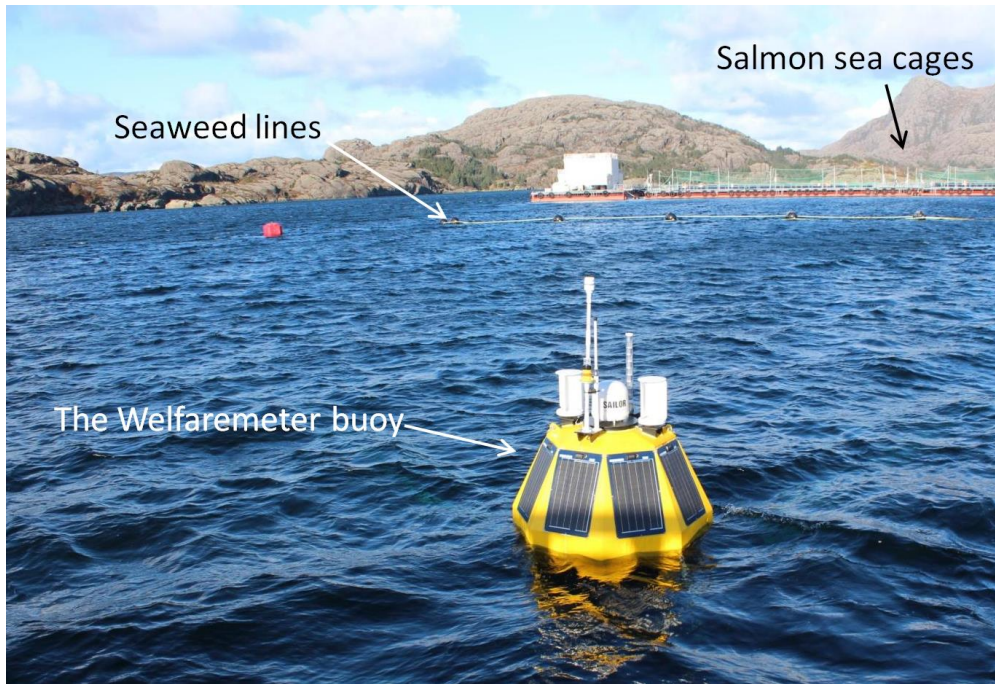
Figure 2: The Welfaremeter buoy deployed at a salmon and seaweed aquaculture site.
