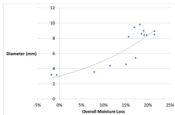
Figure 4.6 Stem diameter vs moisture loss
