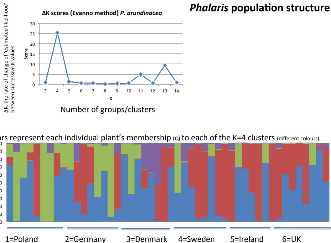
Figure 2.2: Population genetic structure in European Phalaris samples genotyped using plastid SNPs of near complete genomes.
