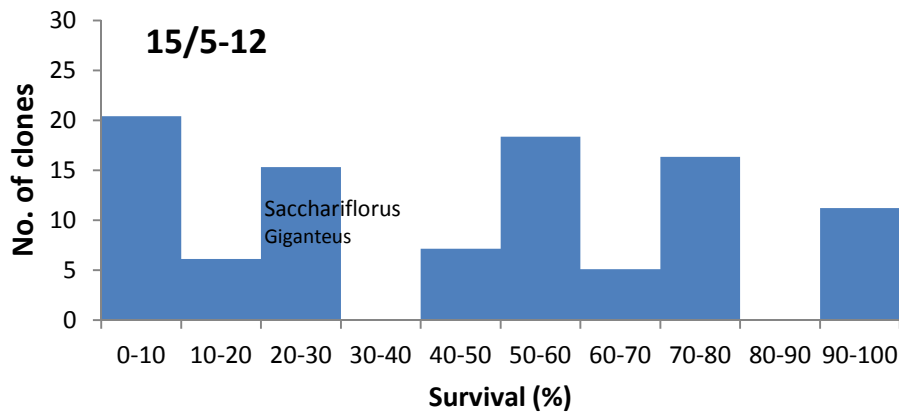
Figure 3.10. Shoot survival after severe frost on May 6-8 th .
