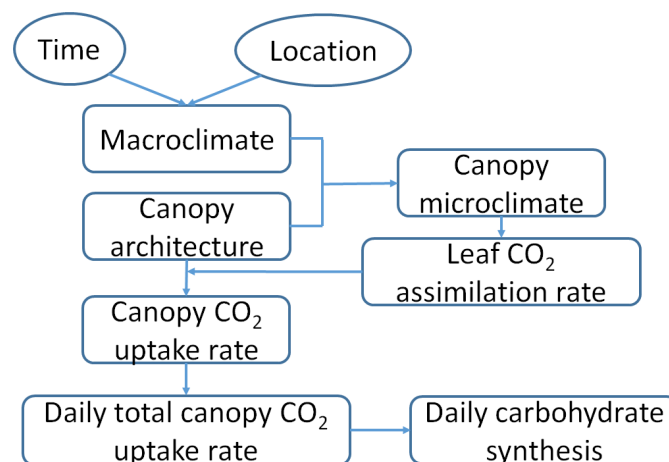
Figure 1.2. The major processes incorporated into this new Java version WIMOVAC.
