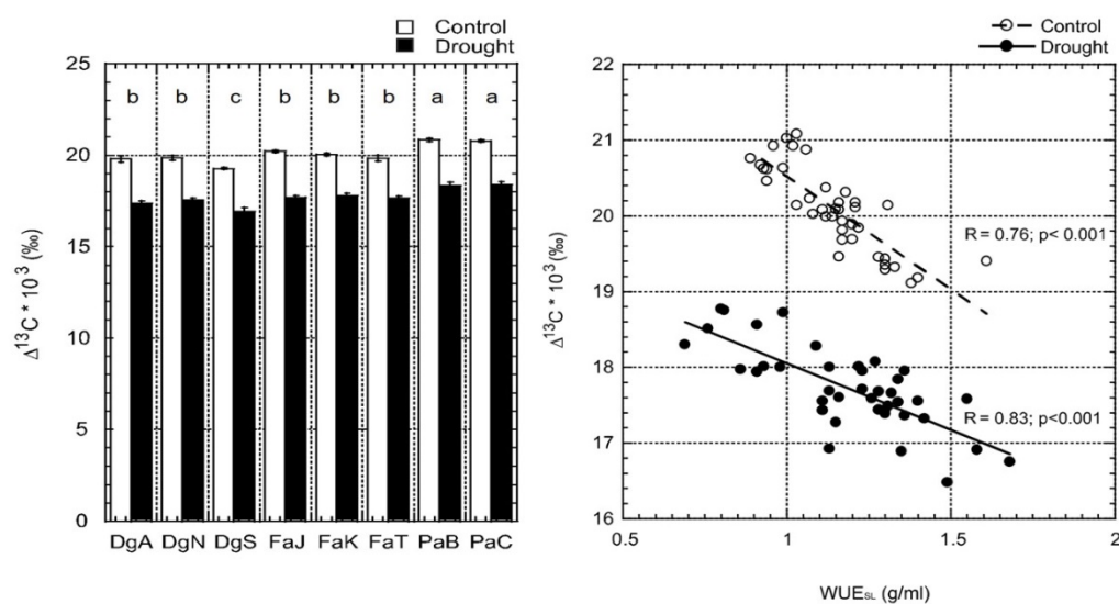
Figure 3.4. Discrimination of ^{13}\text{C} (‰) in shoot material of species and varieties under control (white bars) and drought treatment (black bars) – LEFT. Relationship between \Delta^{13}\text{C} discrimination (‰) and \text{WUE}_{\text{SL}} (g/ml) - RIGHT.
