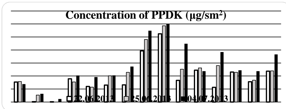
Figure 3.9. PPDK content in Miscanthus at 24C (22.06) and after increasing time at 14C (25.06 and 04.07).
