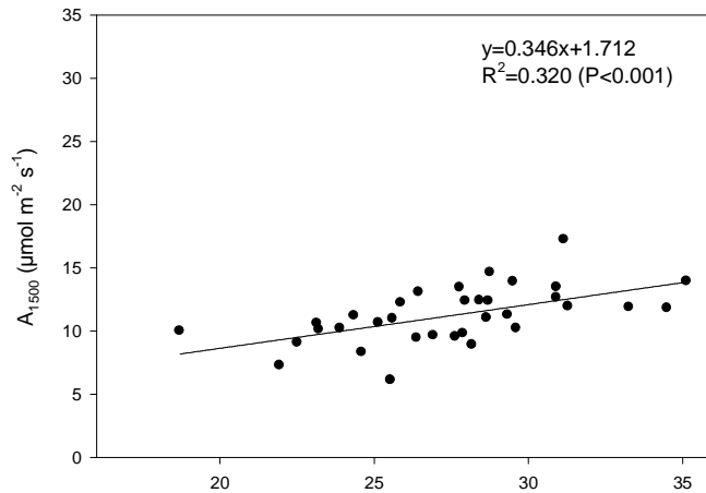
Figure 3.8. Relationship between specific leaf area and photosynthetic rate under cold conditions in miscanthus genotypes.
