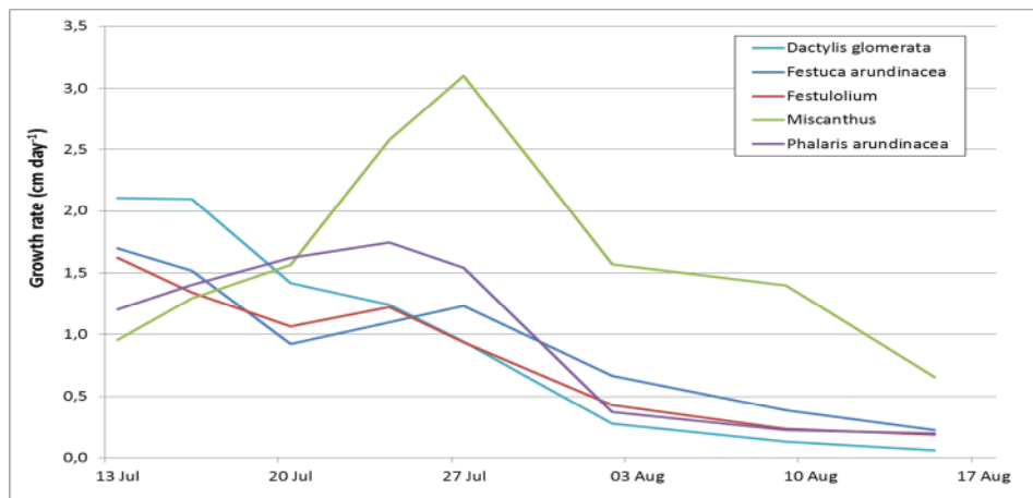
Figure 3.6. Daily shoot growth rates before onset of increased water table (from July 15 th ) until full flooding (from July 28 th ).
