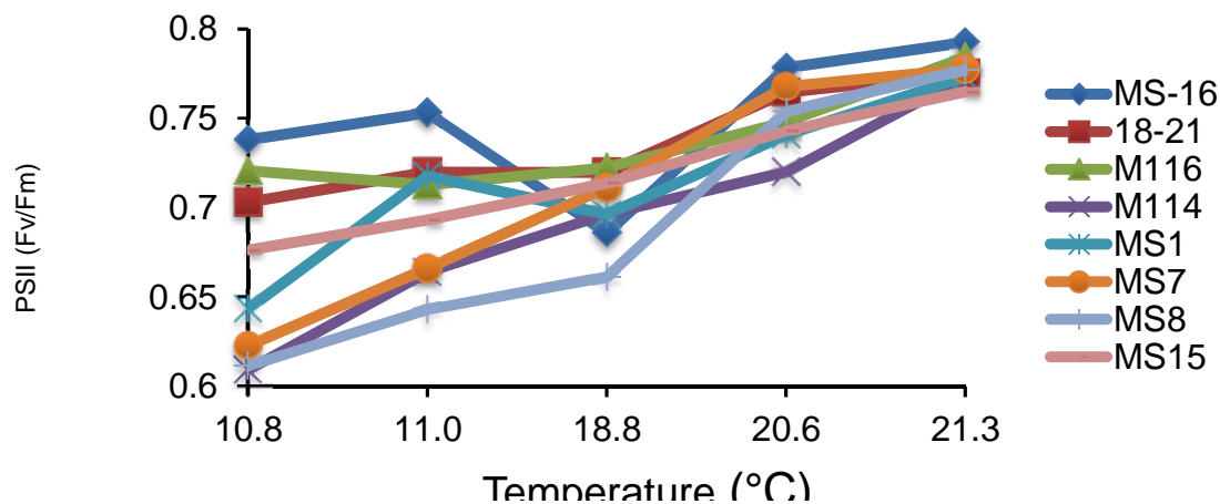
Figure 3.7. Maximum quantum yield of PSII (Fv/Fm) of miscanthus at cold and warm temperatures in the field.
