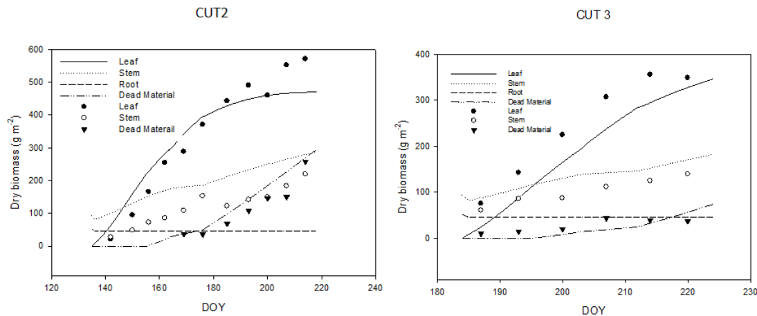
Figure 1.3. The predicted and measured biomass of different organs in Festulolium after the second and third cut. The lines represent the simulation results. The dotted symbols represents the measured values.
