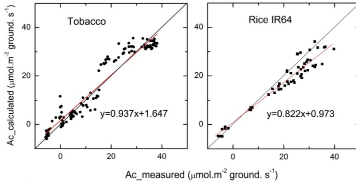
Figure 1.1. The correlation between measured and predicted canopy photosynthesis. These results show that our canopy photosynthesis model can accurately predict canopy photosynthetic CO 2 uptake rates.
