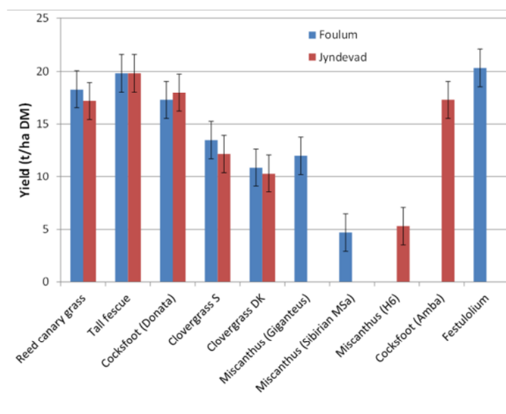
Figure 4.4: Yields (ton/ha DM) in 2014 of grasses and grass-legume mixtures at a coarse sandy soil (Jynde vad) and a loamy sand (Foulum).
