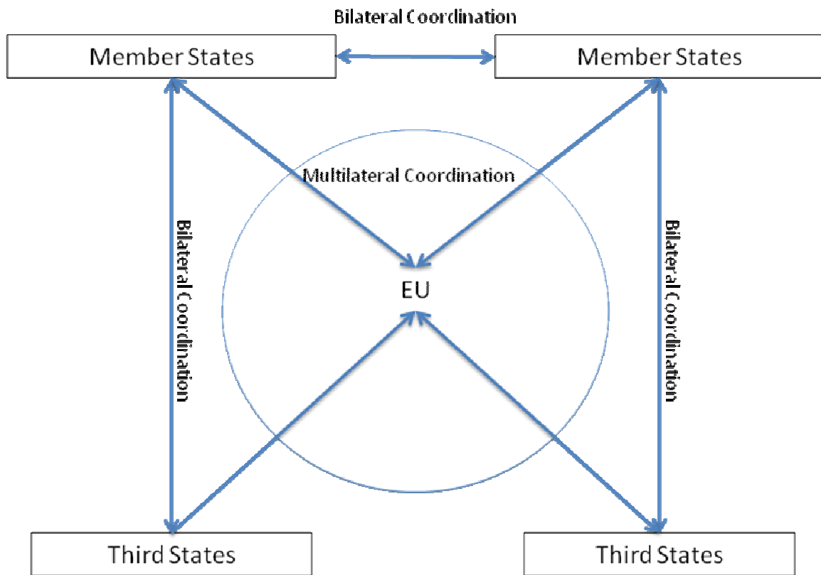
Figure 1: Diagrammatic Depiction of a simple coordination game
