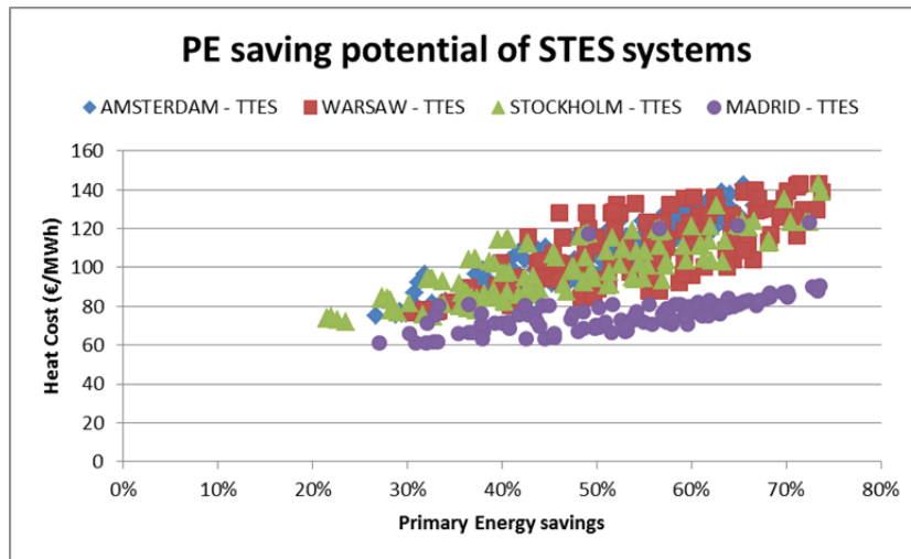
Figure 14: PE saving potential of STES systems
