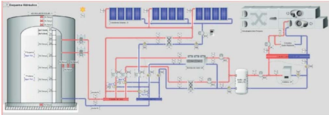
Figure 8. Layout of the Bilbao demo
