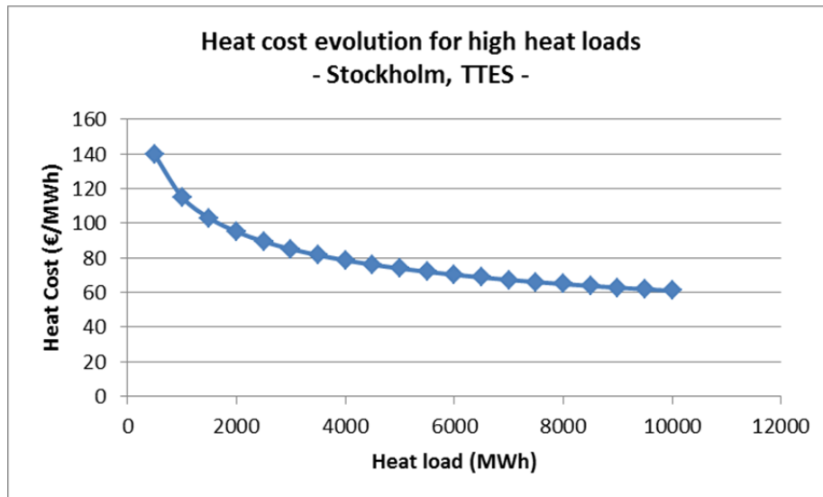
Figure 16: Heat cost of STES plants depending on the heat load to be delivered
