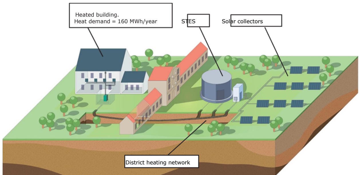
Figure 3. Concept of the heating system
