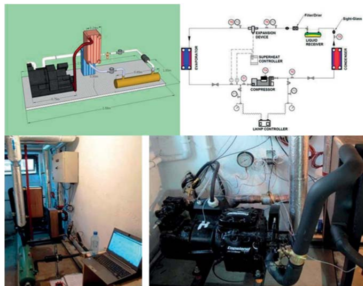
Figure 9. Schematic Sensor Positions and Images of the Heat Pump on site
