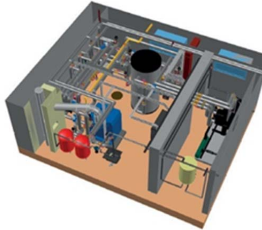
Figure 5. The 3d layout of the boiler in the Polish Pilot Plant
