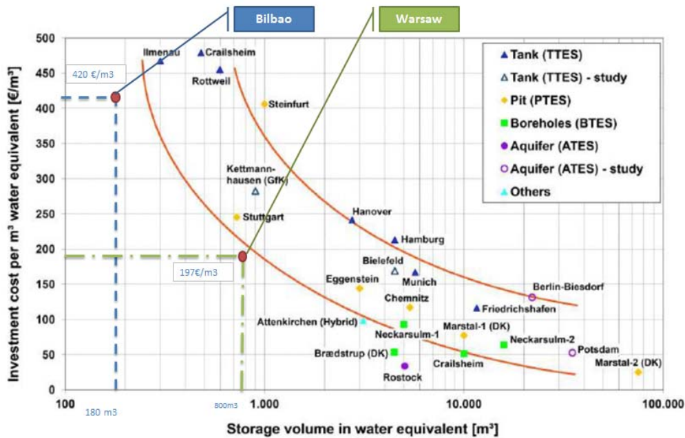
Figure 15: Specific investment cost of different STES typologies of real plants
