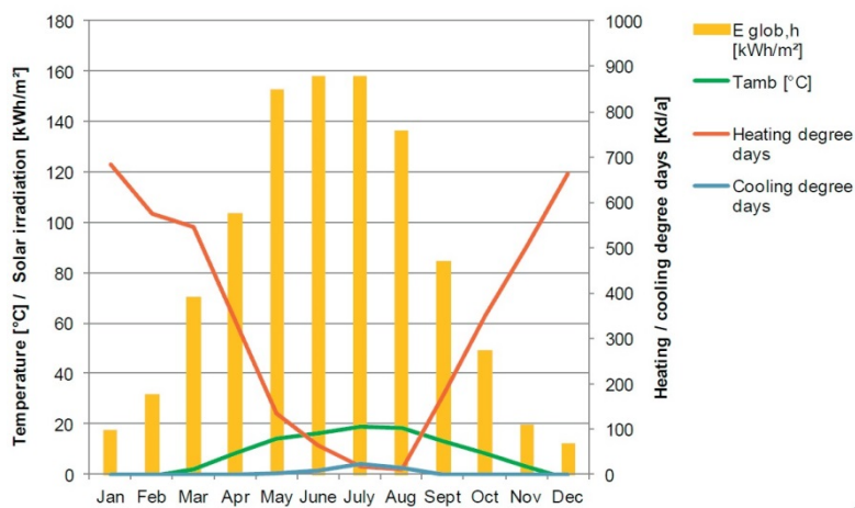
Figure 2. Monthly values for solar irradiation ( E_{glob,h} ), ambient temperature ( T_{amb} ), heating and cooling degree days for Warsaw according to Meteonorm
