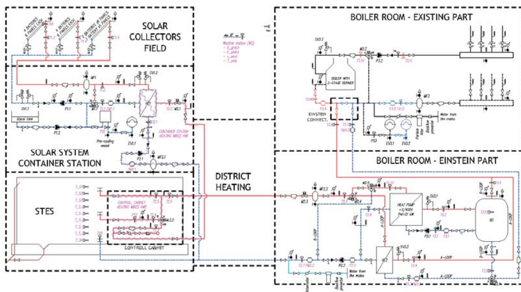
Figure 4. Final design of the EINSTEIN Polish Pilot Plant
