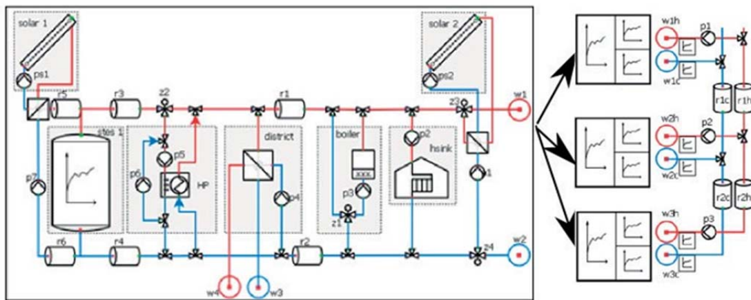
Figure 10 . Simulation of solar collectors and thermal energy storage coupled with district heating.
