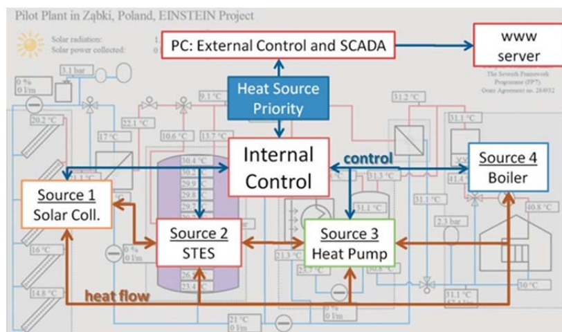
Figure 11. Control approach at the Polish pilot plant. The multi-source heating system with
