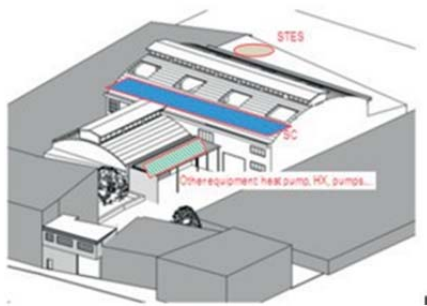
Figure 6. Main equipment of the Bilbao Einstein demo
