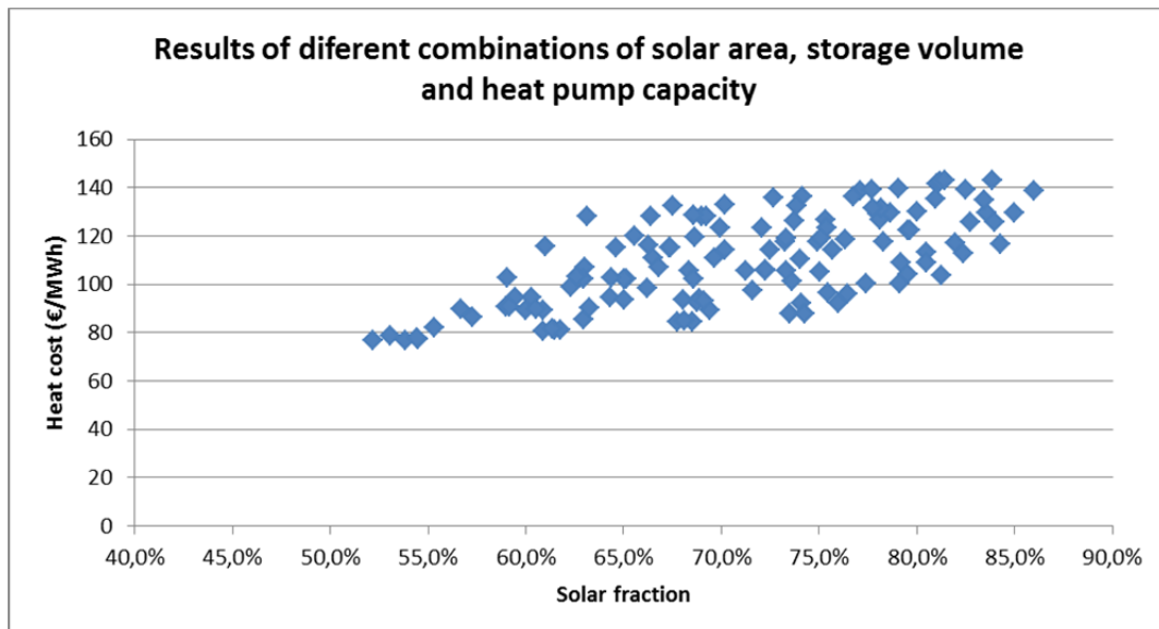
Figure 17: heat cost VS solar fraction of different combinations of solar area, STES volume and HP capacity
