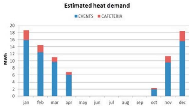
Figure 7. Estimated heat demand at Bilbao demo
