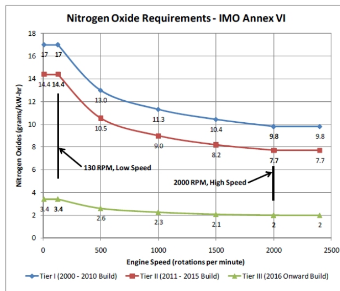
Figure 4 NO x Tier limits from IMO Annex VI 2
