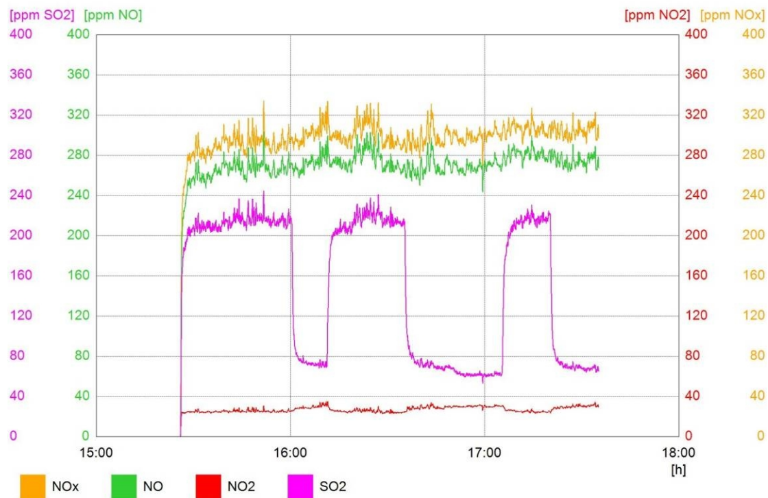
Figure 11 SO x reduction with NTPR
