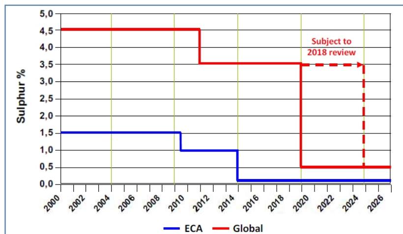
Figure 2: IMO timeline for reduction in fuel sulphur content
