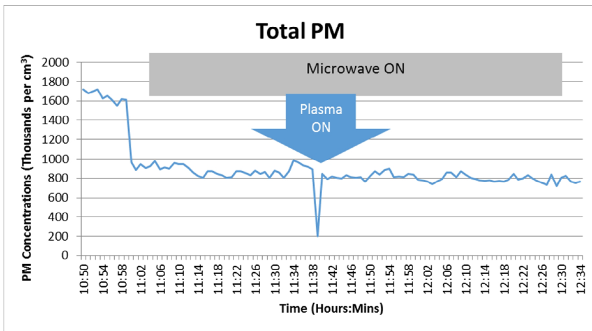
Figure 10 PM reduction with non-thermal plasma
