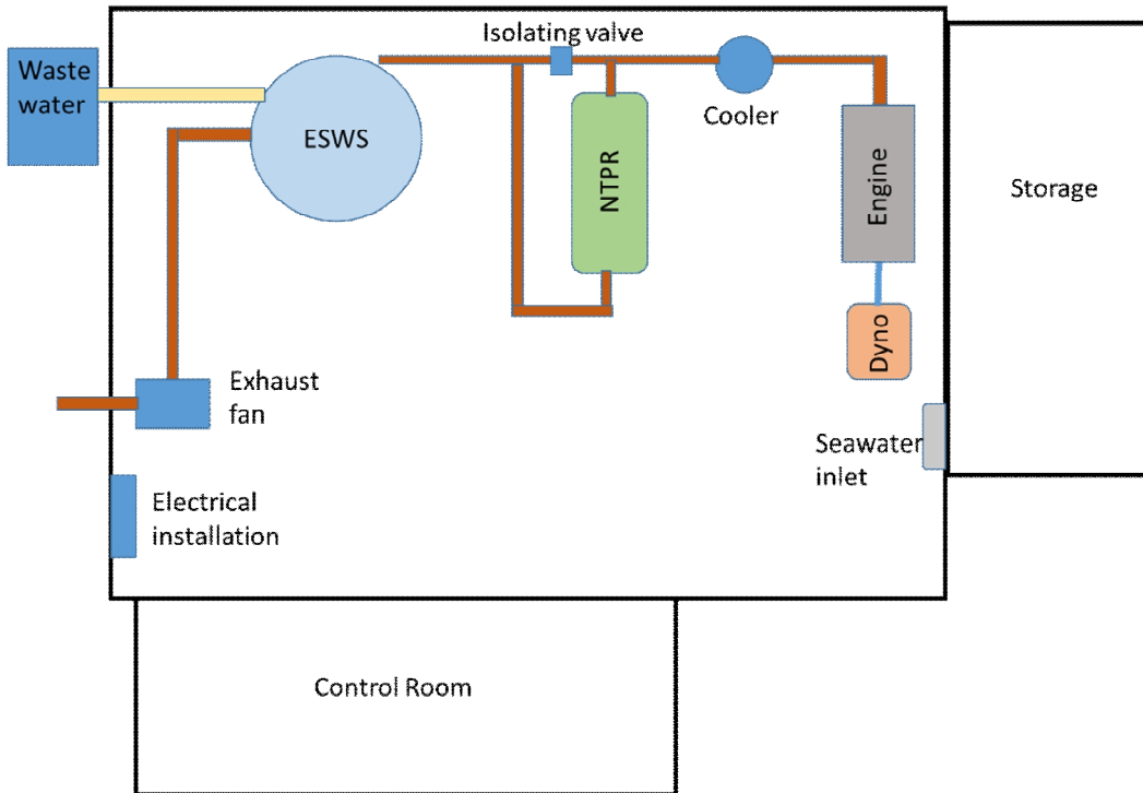
Figure 5 Layout of DEECON Pilot Scale System
