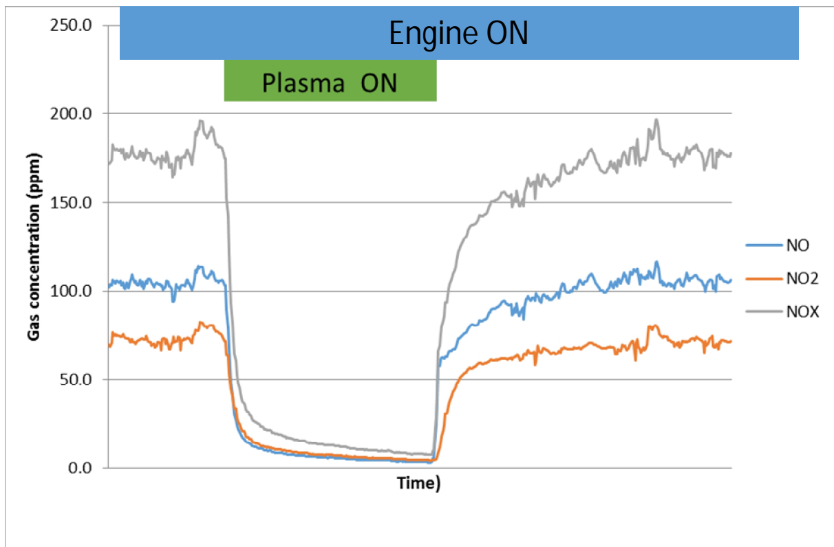
Figure 7 NO, NO 2 and NO x reductions with NTPR
