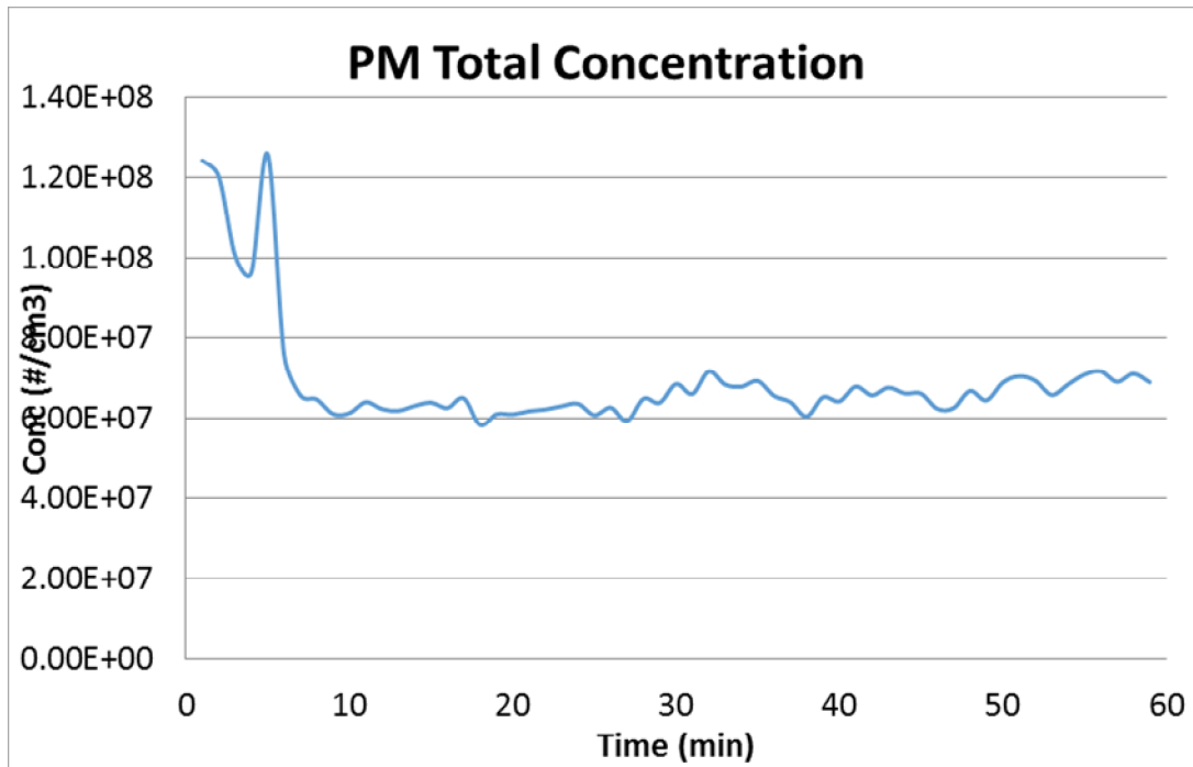
Figure 9 PM reduction with microwave only
