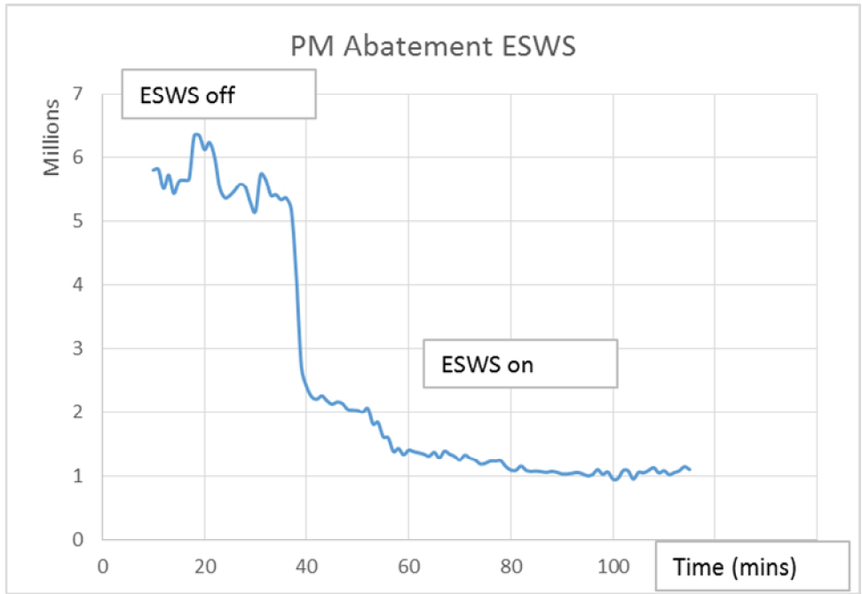
Figure 12 reduction of PM with ESWS
