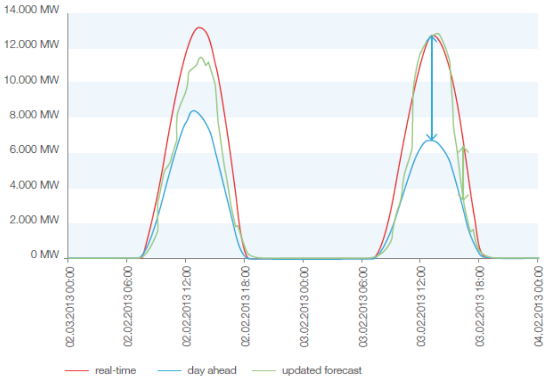
Figure 3: TenneT Germany, PV forecast deviation: fog forecasted, but not occurred (deviation 6000 MW to DACF; 3000 MW to updated forecast)
