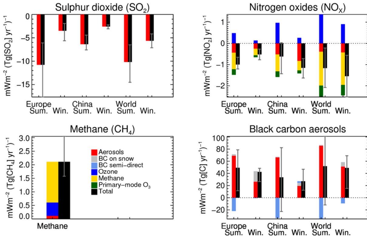
Figure 7: The ECLIPSE estimates of specific radiative forcing (SRF, mWm^{-2} per Tg\ yr^{-1} of emission rate change) for reductions in the emissions of SO_2 , NO_x , CH_4 , and BC aerosols in Europe, China and the global average, separately for NH summer (Sum., May-October) and NH winter (Win., November-April). Shown are values averaged over all five models, with the error bars indicating the full range of the model estimates. Colours indicate the contribution of different forcing mechanisms. Notice that for CH_4 regionality was not accounted for because, due to its longer lifetime, forcing does not depend on the emission region.
