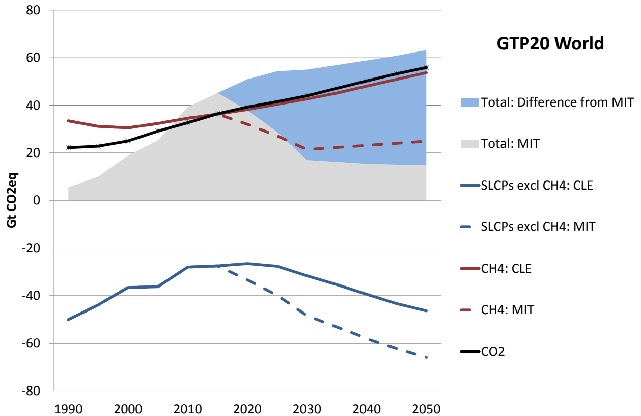
Figure 9: CO 2 -equivalent emissions (Gt) determined with the GTP 20 metric, as a function of time, for global emissions of the current legislation (CLE) and SLCP mitigation (MIT) scenarios. Lines show the values for individual forcing components (black CO 2 , red CH 4 , blue other SLCPs), while the shaded areas show the total CO 2 equivalent emissions from all SLCPs and CO 2 . The blue shading indicates the mitigation potential of MIT, compared to CLE.
