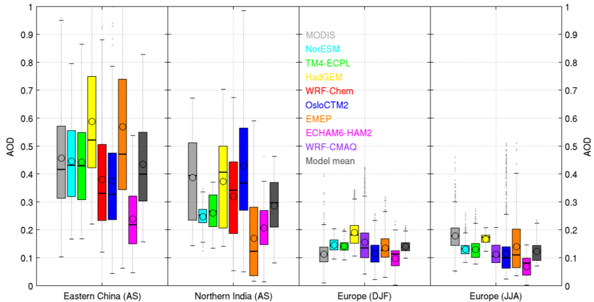
Figure 4: Comparison of satellite-derived (MODIS) and modelled aerosol optical depth (AOD) at wavelengths of 550 nm over Eastern China and Northern India (for area definition, see Quennehen et al., 2015) in August-September 2008, and Europe (14.5°W-34.5°E, 35.5°-74.5°N) in winter (December-February, DJF) and summer (June-August, JJA) of 2008. Mean values (circles), medians (central lines), 25 th and 75 th percentiles (boxes) and range of other data excluding outliers (whiskers) are shown.
