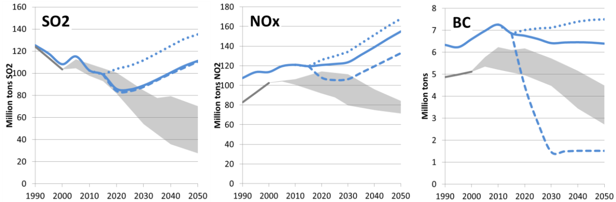
Figure 2. Global anthropogenic emissions of CO_2 , CH_4 and key air pollutants ( SO_2 , NO_x and BC ) for the current legislation (CLE), no further controls (NFC) and ECLIPSE SLCP mitigation scenario. Units are Gt for CO_2 and Mt for the SLCPs. Also shown for comparison is the range of the RCP emission scenarios (grey shading).
