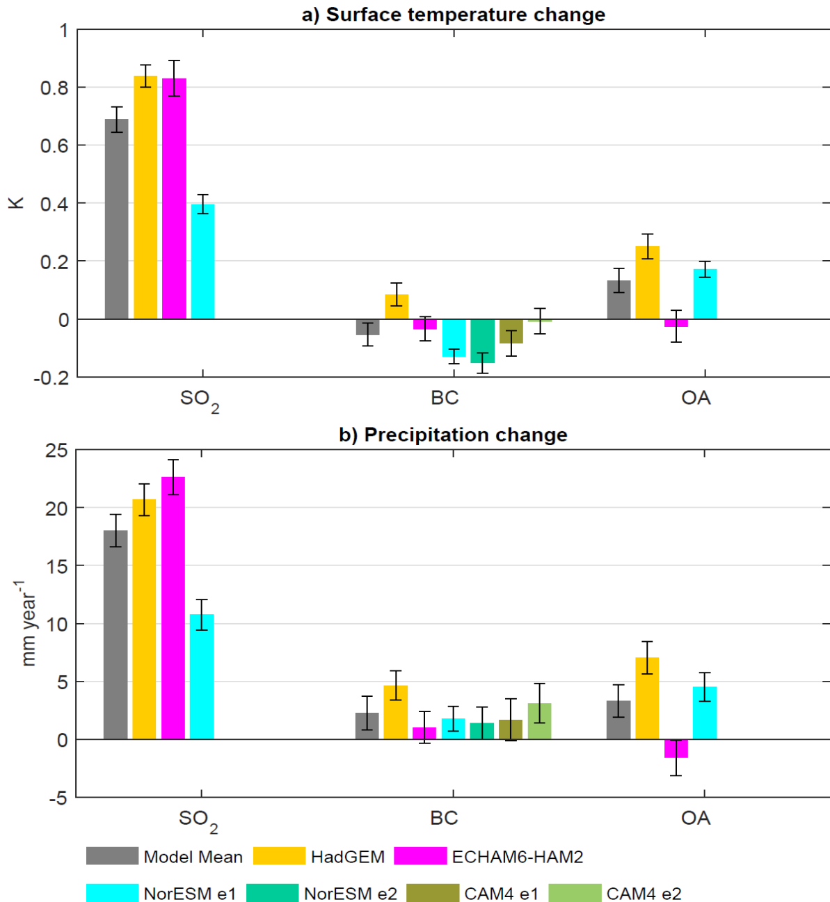
Figure 12: Global mean annual average changes in (a) surface temperature and (b) precipitation averaged over all land areas excluding ice sheets, from the four ESMs (one was run only for BC), for a complete removal of all land-based emissions of a particular species, compared to the ECLIPSE version 4 baseline emissions for the year 2008 (CESM-CAM4 used the year
