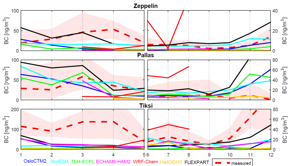
Figure 5. Monthly (month is displayed on the abscissa) median observed and modelled BC concentrations for the stations Zeppelin on Svalbard (11.9°E, 78.9°N, top), Pallas in Finland (24.12°E, 67.97°N, middle) and Tiksi in Siberia (128.9° E, 71.6°N, bottom), for late winter/spring (left column) and summer/autumn (right column) for the years 2008-2009 (for Tiksi, measured values were available only from July 2009 to June 2010). The red dashed lines connect the observed median values, the light red shaded areas span from the 25 th to the 75 th percentile of the observations. Modelled median values are shown with lines of different colour
