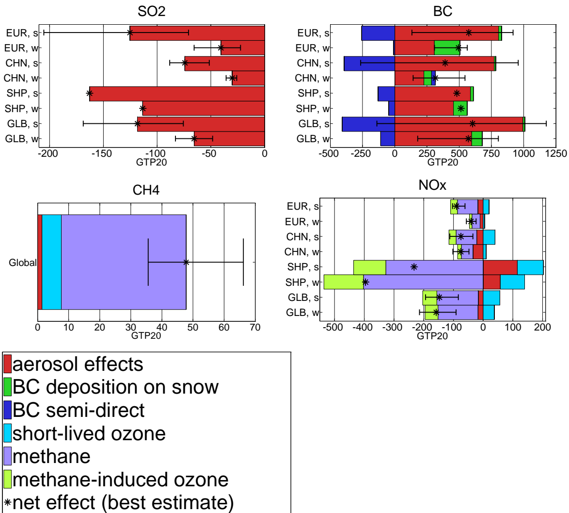
Figure 8: GTP_{20} values for SLCPs, relative to an equal mass emission of CO_2 , for all regions and seasons, decomposed by processes and based on the RF values shown in Fig. 7. The regions included are Europe (EUR), China (CHN), global (GLB), and the shipping sector considered separately (SHP), all for both NH summer (s, May-October) and NH winter (w, November-April). Uncertainty bars reflect model spread. Only two models calculated effects of emissions from shipping and there no uncertainty range is given.
