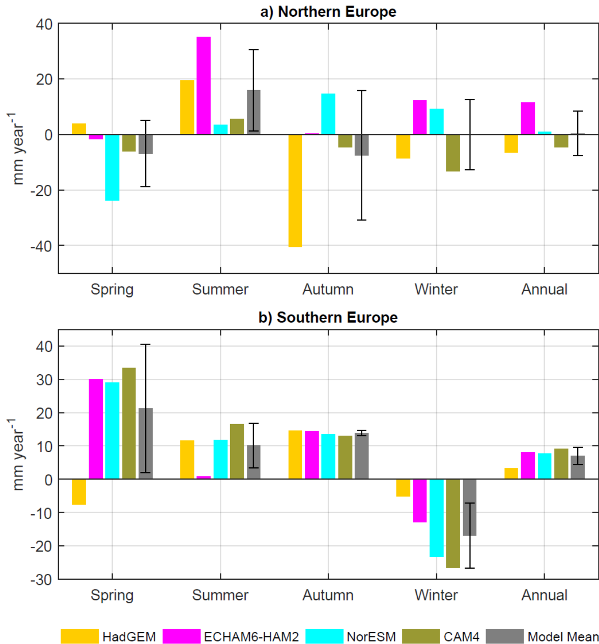
Figure 17: Seasonal and annual mean differences in precipitation (in \text{mm y}^{-1} ) over Northern (a) and Southern (b) Europe between transient simulations of the mitigation (MIT) scenario and the current legislation (CLE) scenario, averaged over the last 10 years of the simulations (2041-2050). Regions are defined as for Figure 15 (a, b). Results are shown for the four ECLIPSE models individually and for the multi-model mean. Positive values mean that MIT
