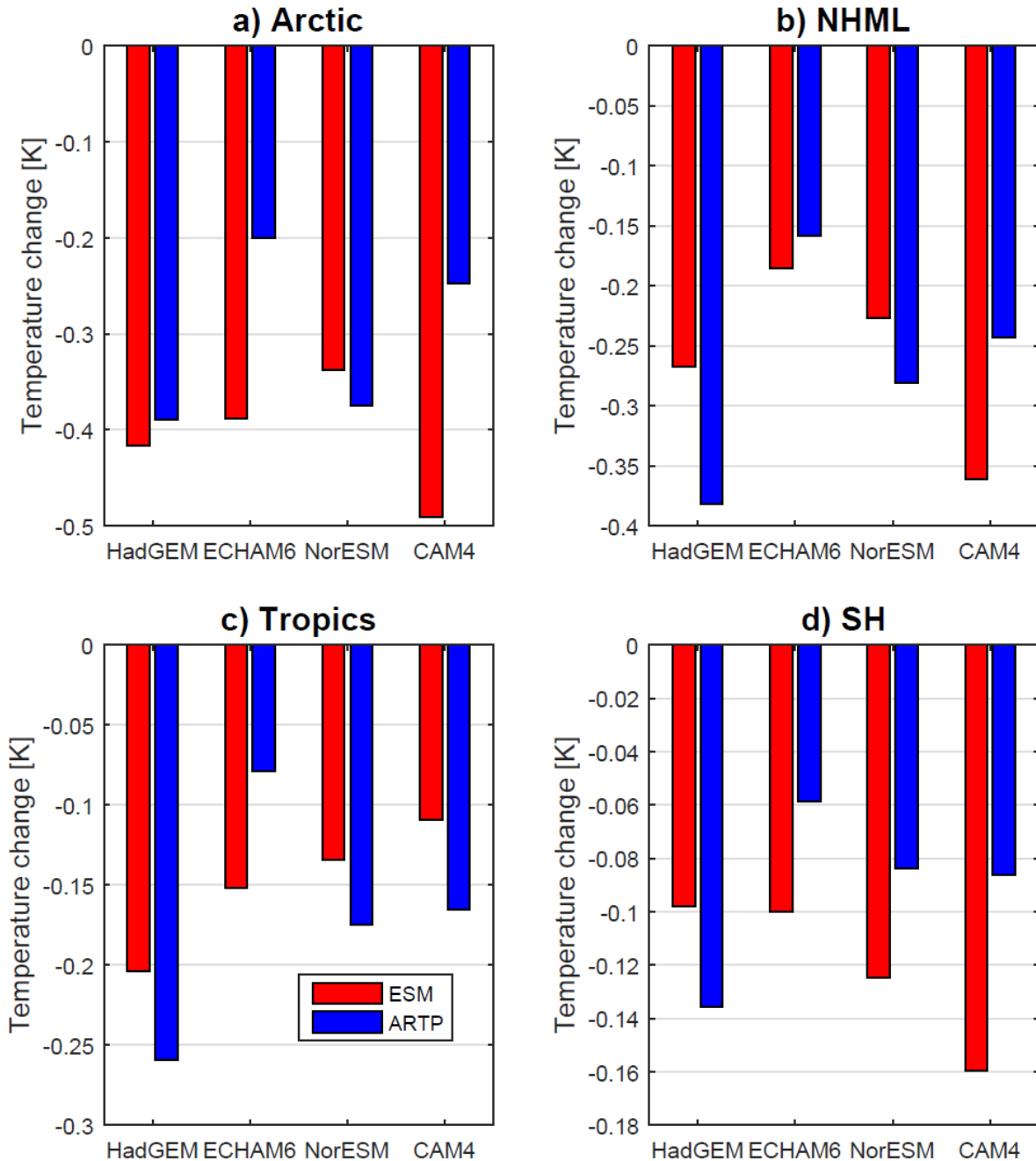
Figure 20: Temperature changes (MIT-CLE) in four latitude bands (Arctic, Northern Hemisphere Mid-Latitudes (NHML), Tropics and Southern Hemisphere) calculated with the ESMs and ARTP-based method. Mean changes over the 2031-2050 period are shown. Notice the different temperature scales.
