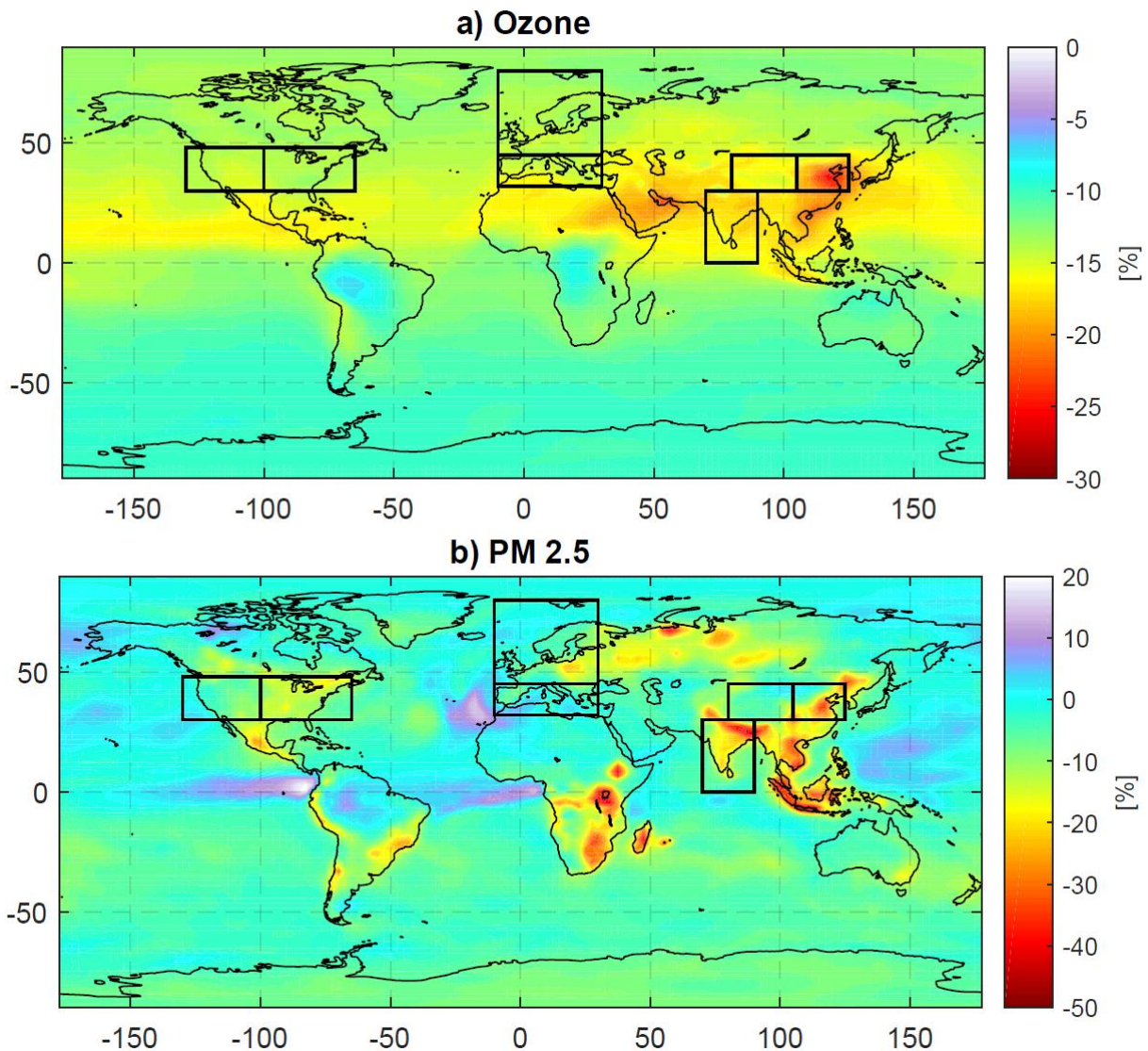
Figure 10: Relative difference maps (in %) for the surface concentrations of O 3 and PM 2.5 , as obtained from simulations based on the emission mitigation (MIT) scenario and the current legislation (CLE) scenario, i.e. (100 \times (\text{MIT}-\text{CLE})/\text{CLE}) . Shown are mean concentration differences for the period 2041-2050 and averaged over model results from OsloCTM2, NorESM and HadGEM.
