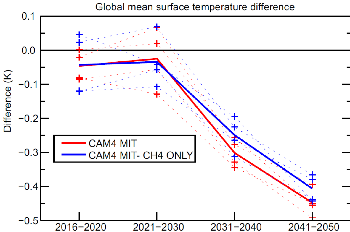
Figure 18: Time evolution of differences in global mean surface temperature between transient simulations following the mitigation (MIT) and the current legislation (CLE) scenario (i.e., MIT-CLE), as simulated by the CESM-CAM4 model with a slab-ocean representation. One experiment (red lines) included all emission reductions of the MIT scenario, whereas another experiment (blue lines) included only the CH 4 emission reductions of the MIT scenario. Ensemble mean results are shown with thick lines, individual ensemble members with thin lines.
