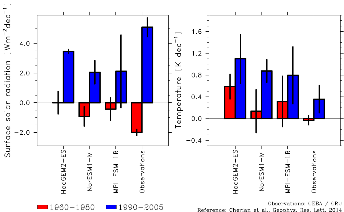
Figure 6. Linear trends in (left) surface solar radiation and (right) near-surface temperature increase per decade over continental Europe from the „historical“ simulations in the CMIP5 archive contributed by previous versions of three ECLIPSE ESMS. The period 1960 – 1980 is shown in red, the period 1990 – 2005 in blue.
