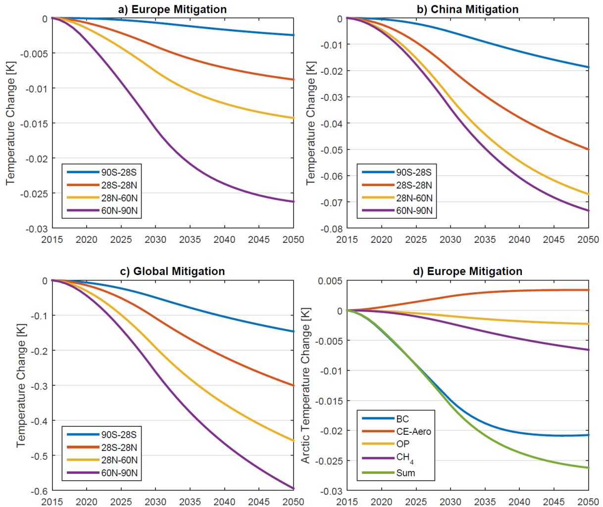
Figure 21: Annual mean surface temperature changes estimated by the ARTP method. Panels a-c: Changes in four latitude bands due to ECLIPSE mitigation scenario (MIT-CLE) for mitigation in Europe (a), China (b) and globally (c). Panel d: Arctic temperature changes due to mitigation of individual components from Europe. CE-Aero: Co-emitted aerosol (precursor) species (OA, SO 2 and NH 3 ), OP: Ozone precursors (NO x , CO and NMVOCs). Note the different scales on the vertical axes.
