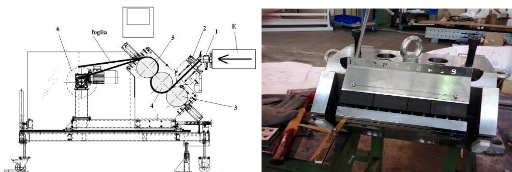
Figure 8. Flat die applied to the Comac extruder for sheets production.
