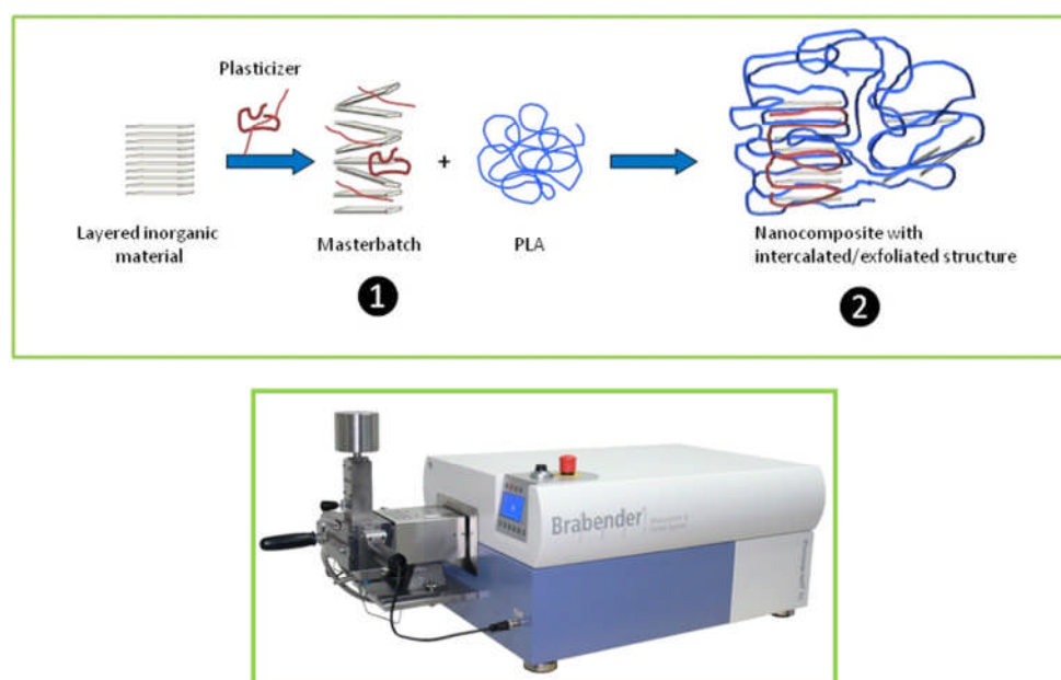
Figure 3. Two step procedure for the preparation of PLA/clay nanocomposites and machine used
