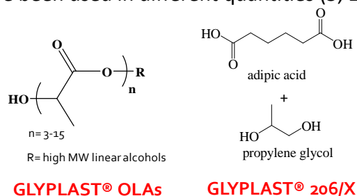
Figure 1: chemical structures of employed plasticizers provided by CQSA
