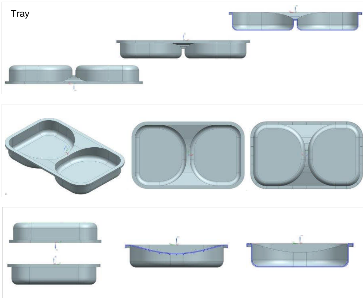
Figure 17. CAD parts of the tray.
