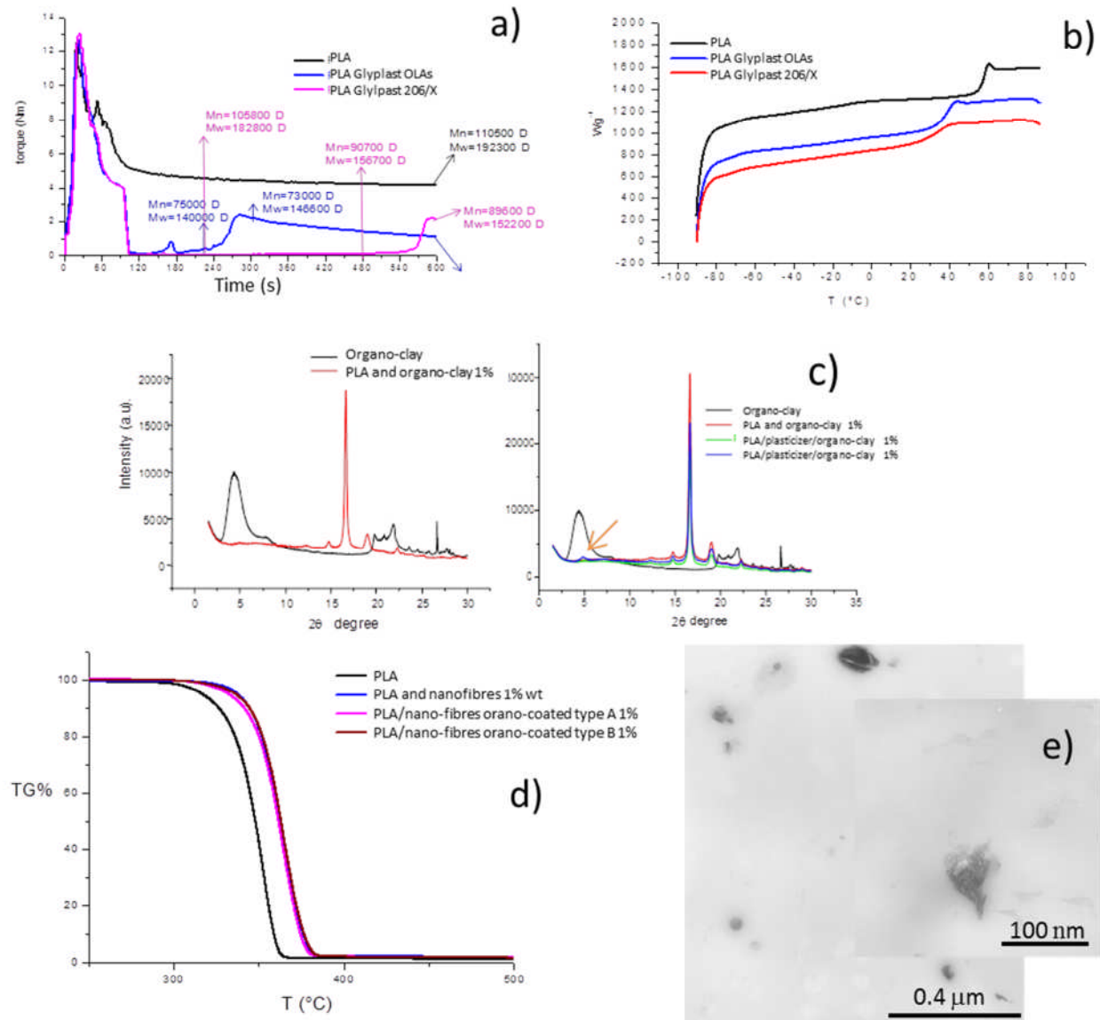
Figure 4: Examples of PLA-based composites testing: a) Torque and Mn/Mw evolution during the melt mixing of PLA with plasticizers of both families investigated; b) DSC analysis showing the exerted plasticizing effects; c) XRD paths of organoclay and different composites suggesting exfoliated or intercalated/exfoliated morphologies; d) TGA of composites obtained with fibres showing the improved thermal stability of collected materials; e) TEM images of nanocomposites obtained by dispersing LDH-modified by ionic exchange with a functional plasticizer (OLA family derived).
