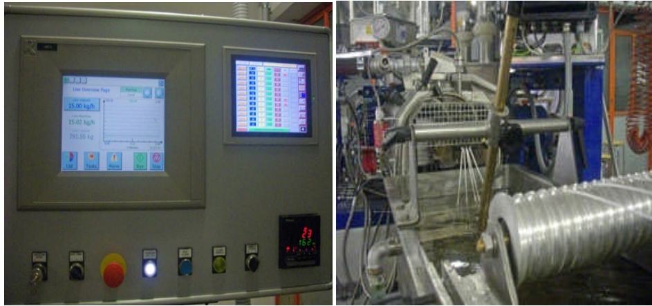
Figure 7. Image of the Comac EBC 25HT pilot-scale co-rotating twin-screw extruder, used for scale up production.
