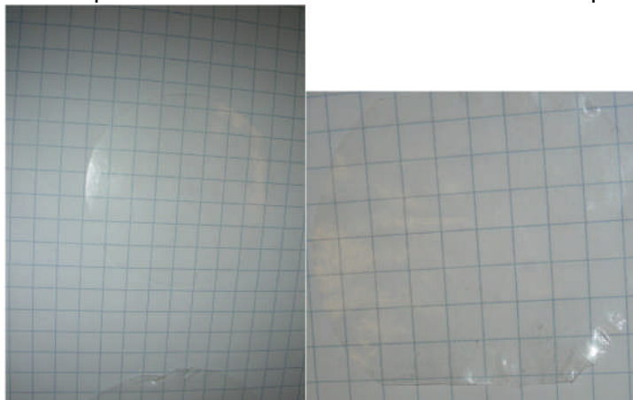
Figure 5. Films obtained by compression moulding of composites a) PLA/nanofibres 1%wt and b) PLA/plasticizer 15% wt/nanofibres 1%wt
