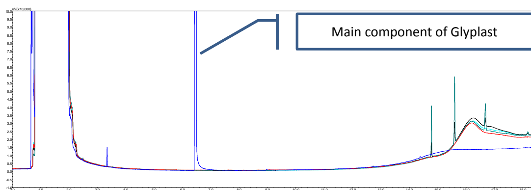
Figure 1. Chromatograms of the migration substances in Glyplast 206/3NL.
