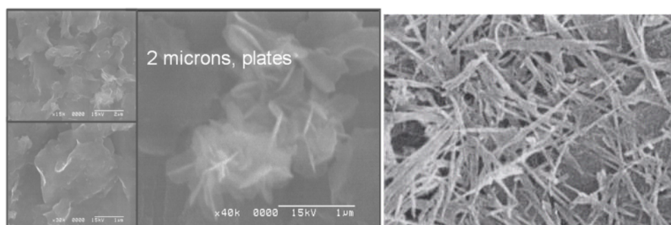
Figure 2: SEM images of organo-coated clay and fibre evidencing the different aspect ratios provided by AVANZARE
