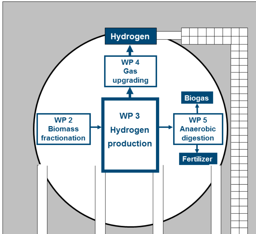
Production of hydrogen, biogas and fertilizer by integration of hydrogen fermentation and biogas production using biomass as feedstock in HyTIME
