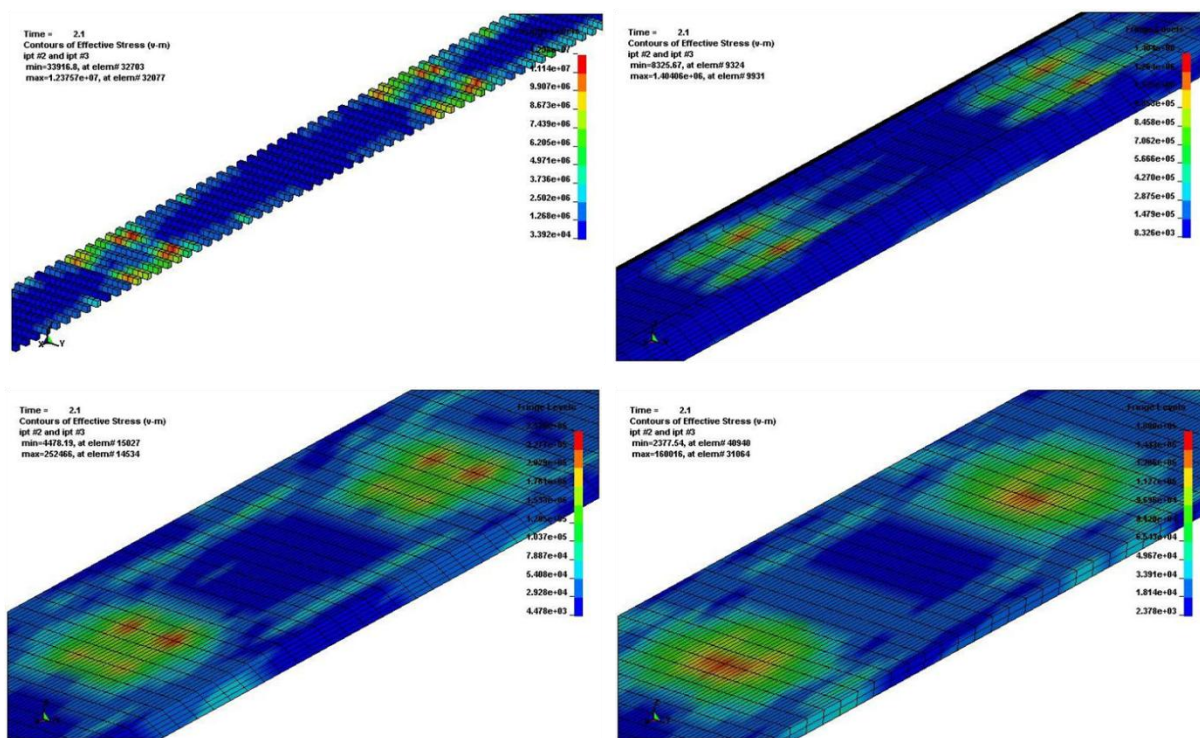
Figure 7: Dynamic FEM analysis of railway substructure showing the contours of effective stress in the different layers: sleepers (top left); ballast (top right); sub-ballast (bottom left) and substrate (bottom right)
