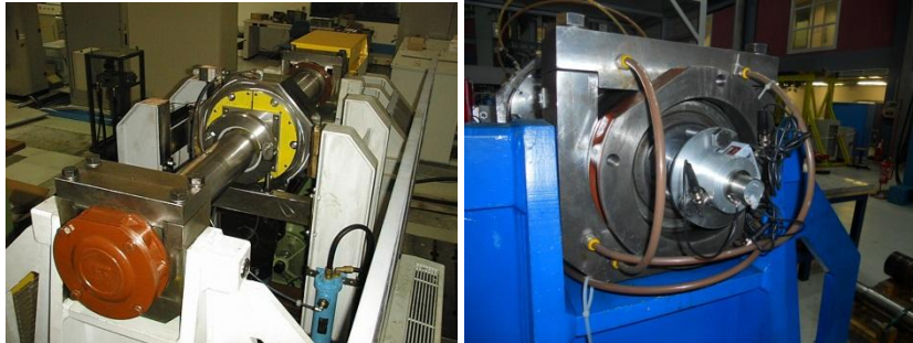
Figure 6: Experimental set-up for full-scale AE and LFV measurements
