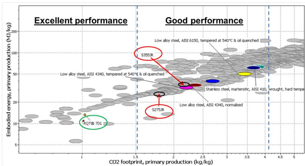
Figure 3: Analysis of Material Selection for the vehicle structure in terms of Embodied energy vs CO2 footprint
