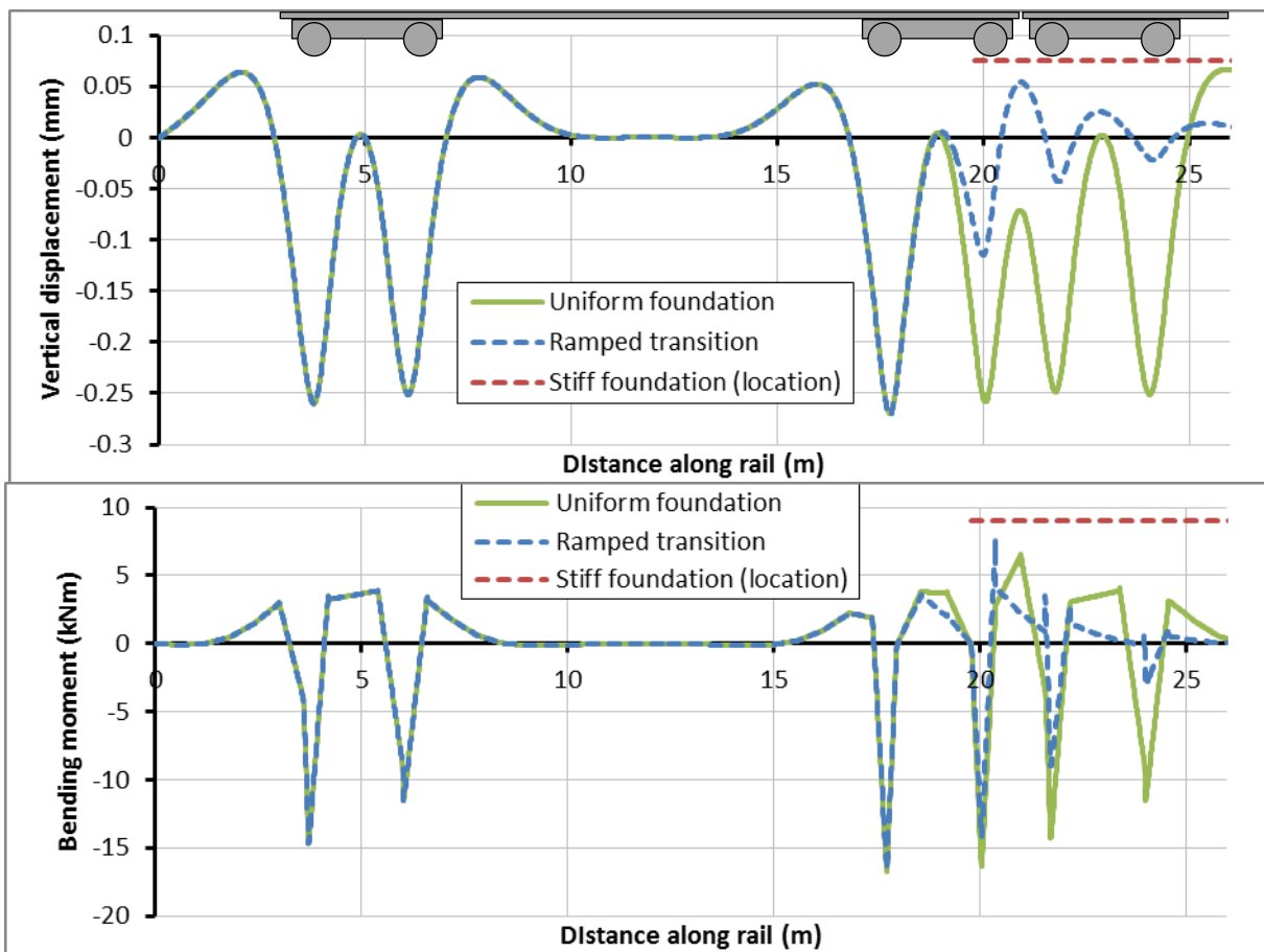
Figure 9: Vehicle passing over ramped transition to stiff support
