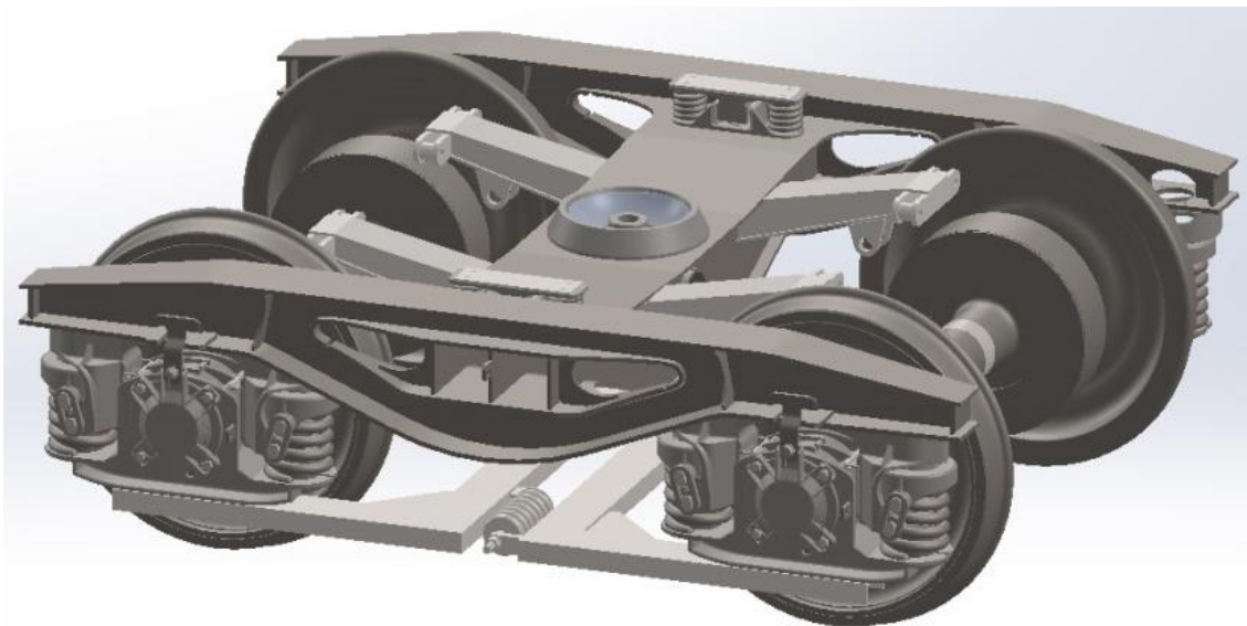
Figure 2: CAD model of the prototype SUSTRAIL freight bogie
