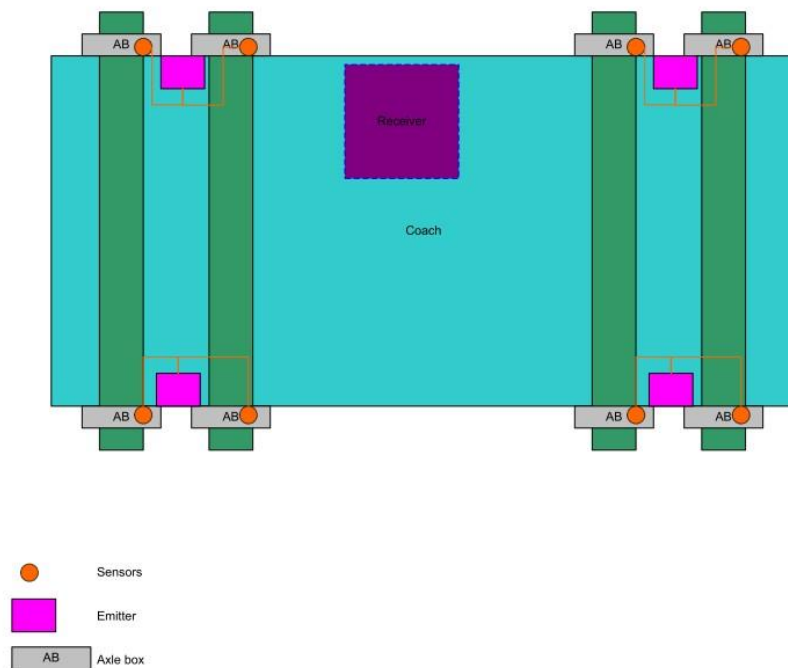
Figure 5: Schematics of SUSTRAIL Vehicle Measuring system
