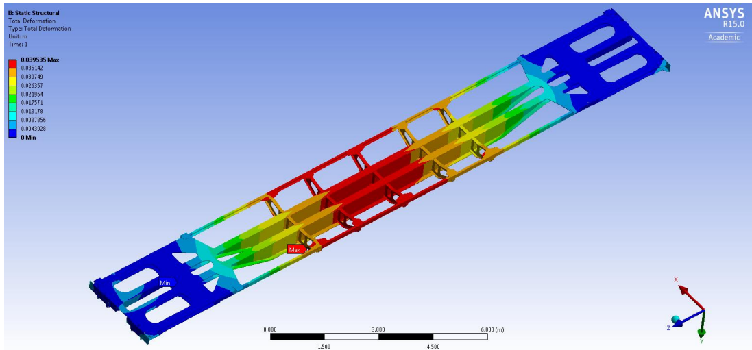
Figure 4: FEM analysis of the wagon frame (Total deformation under vertical and longitudinal service loads)
