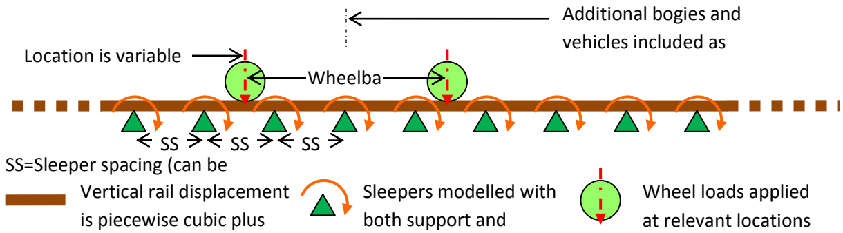
Figure 8: Beam model of rail
