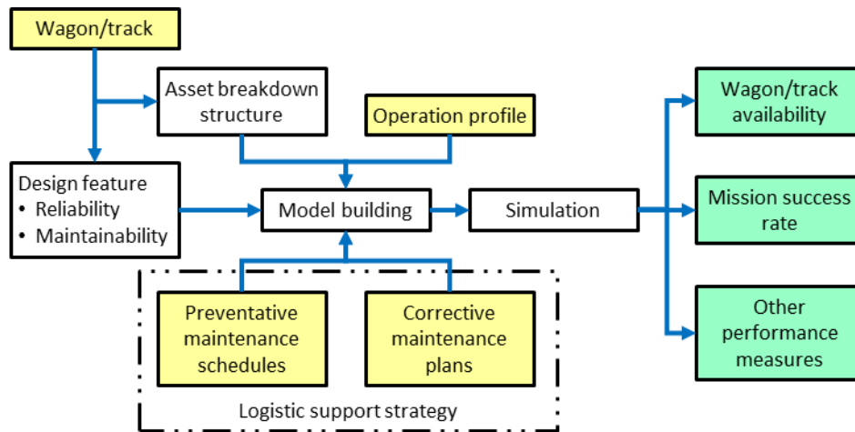
Figure 11: Description for RAMS simulation approach
