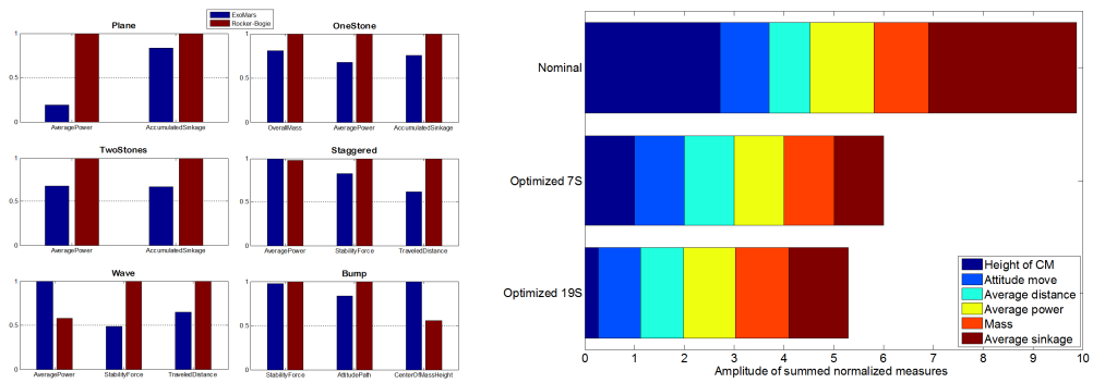
Figure 11: Comparison of performance for optimized ExoMars and Rocker-Bogie rover for 7S (left), and for nominal, optimized 7S and 19S ExoMars suspension (right)
