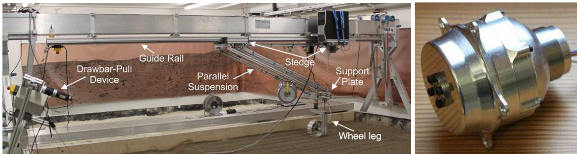
Figure 14: Single Wheel Testbed (left) and actuator unit (right)
