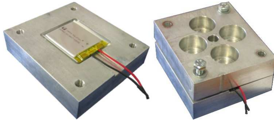
Figure 10: The random vibration battery jig and selected battery cell.
