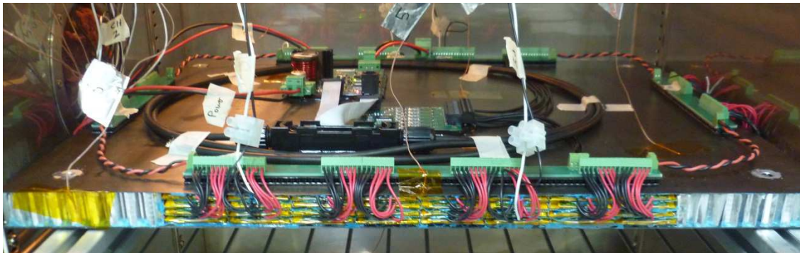
Figure 13: Views of the external prototype. a) detail of the power generator, b) electronics integrated in the inner skin; c) power storage integrated in the core of the panel.
