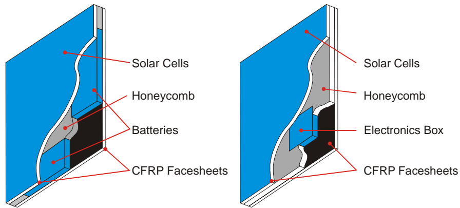
Figure 5: Illustration of the MFS applications
