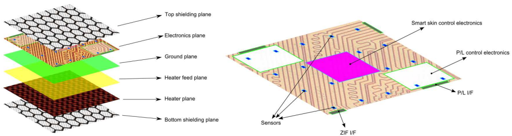
Figure 6: Schematics of the Smart skin.
