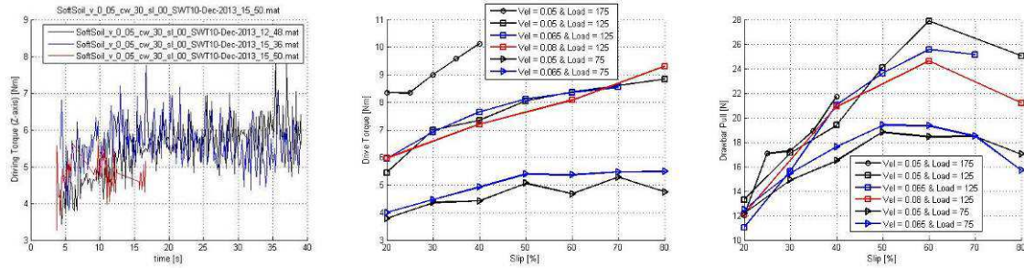
Figure 15: Actuator performance for various operating points on soil: Required drive torque (soft soil left) vs. time, required drive torque vs. slip (hard soil centre), and resulting available free pulling force (hard soil right) vs. slip
