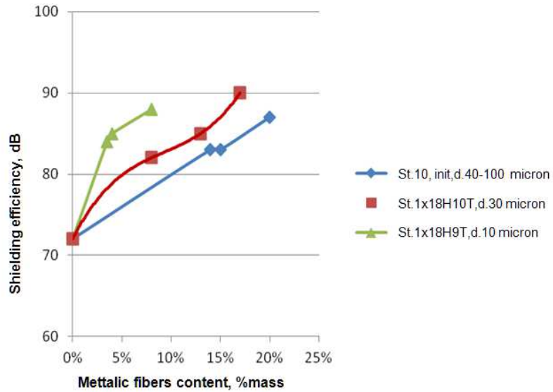
Figure 4: Shielding efficiency dependence of carbon-fiber plastic with the filler, formed from steel fibers, on the diameter of the fiber
