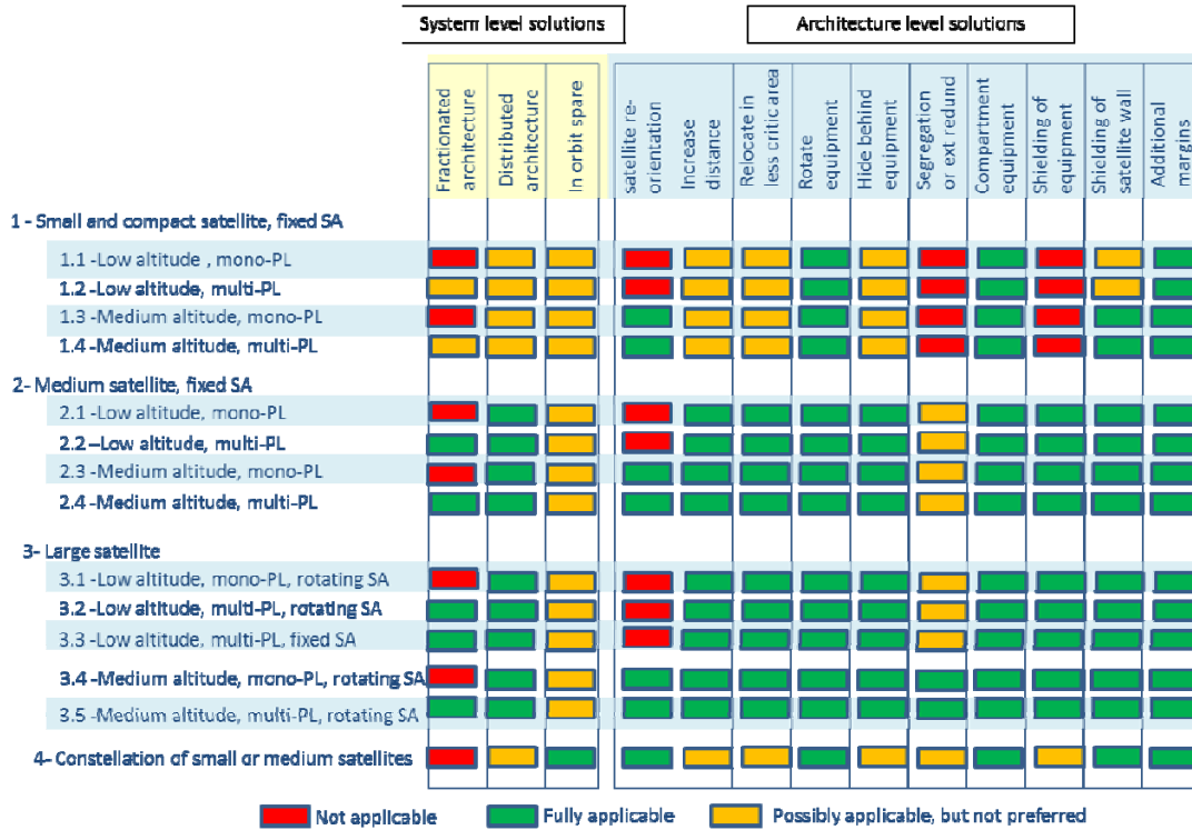
Figure 2-23: Applicability of solutions to satellites
