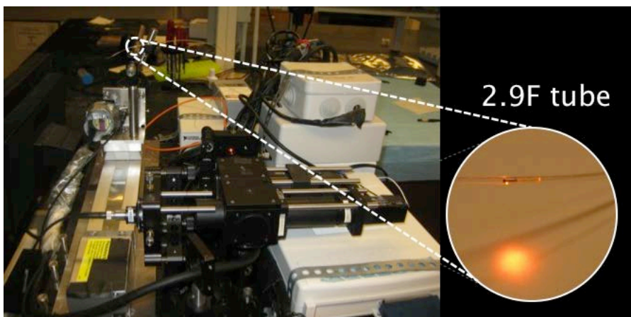
Figure 9. Experimental set-up of NIRF catheter
