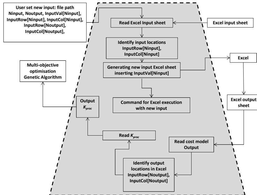
Figure 23: Structure of the interface between the cost model implemented in Microsoft Excel and the multi-objective optimisation GA.
