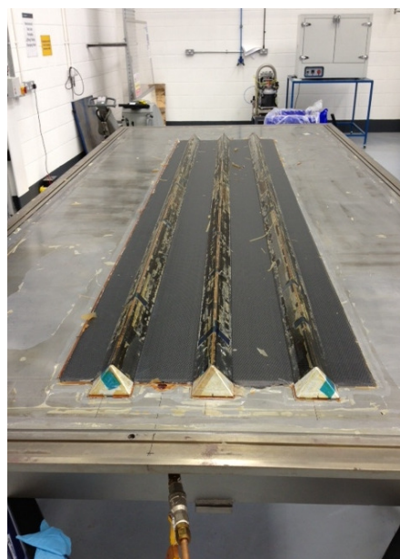
Figure 44: Cured Final demonstrator just after cure on the rigid bottom tool
