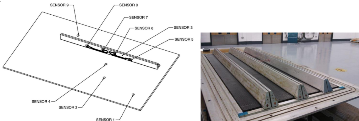
Figure 21: Sensor configuration for monitoring the infusion of a stiffened panel using INASCO flow sensors and DiAMON s/w.
