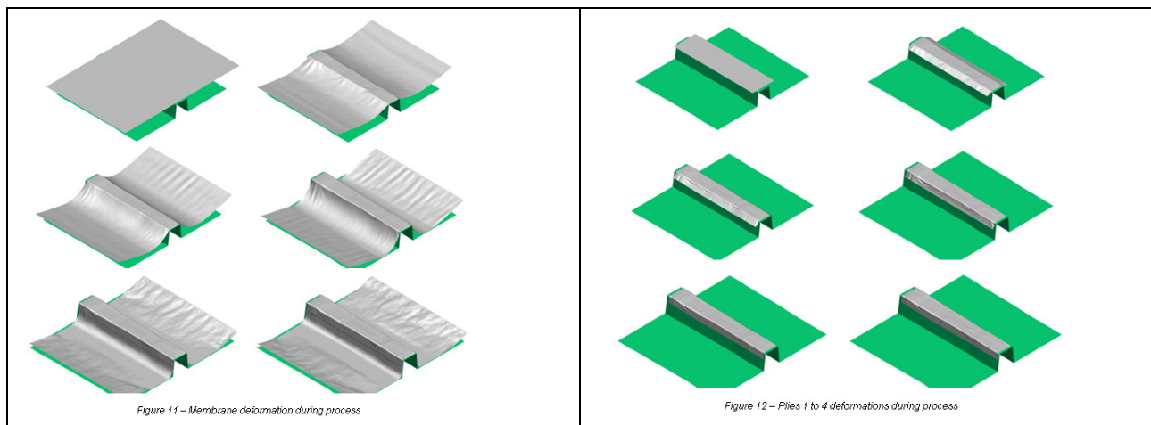
Figure 43: Bombardier preforming studies
