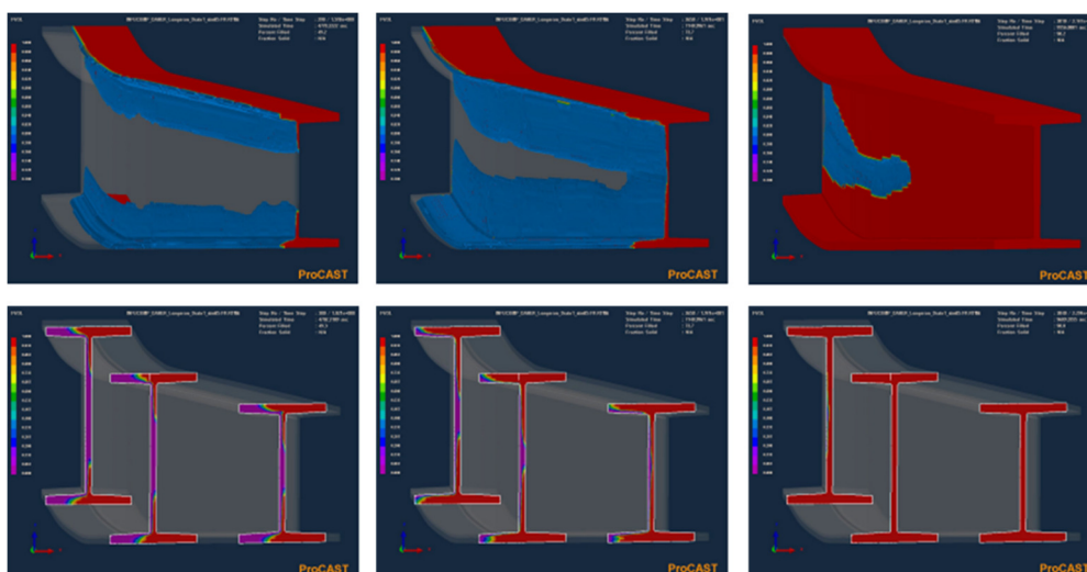
Figure 38: Example DAHER spar simulation results
