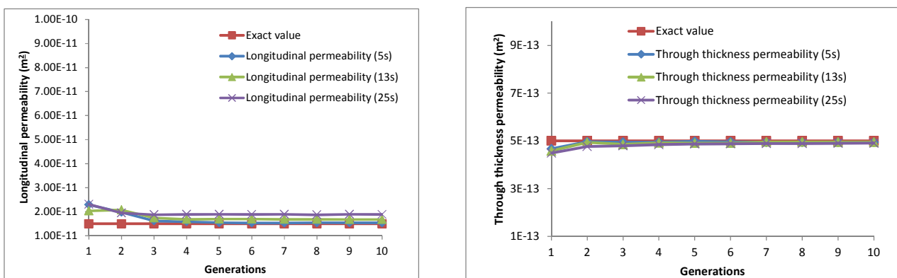
Figure 35: Average permeability convergence: (left) Longitudinal permeability; (right) Through thickness permeability.
