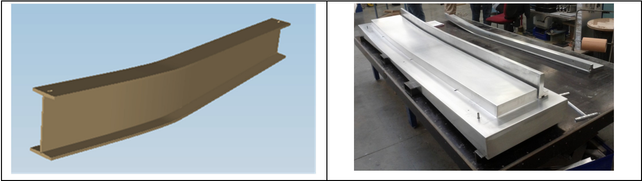
Figure 37: DAHER large scale demonstrator 3D CAD and tooling
