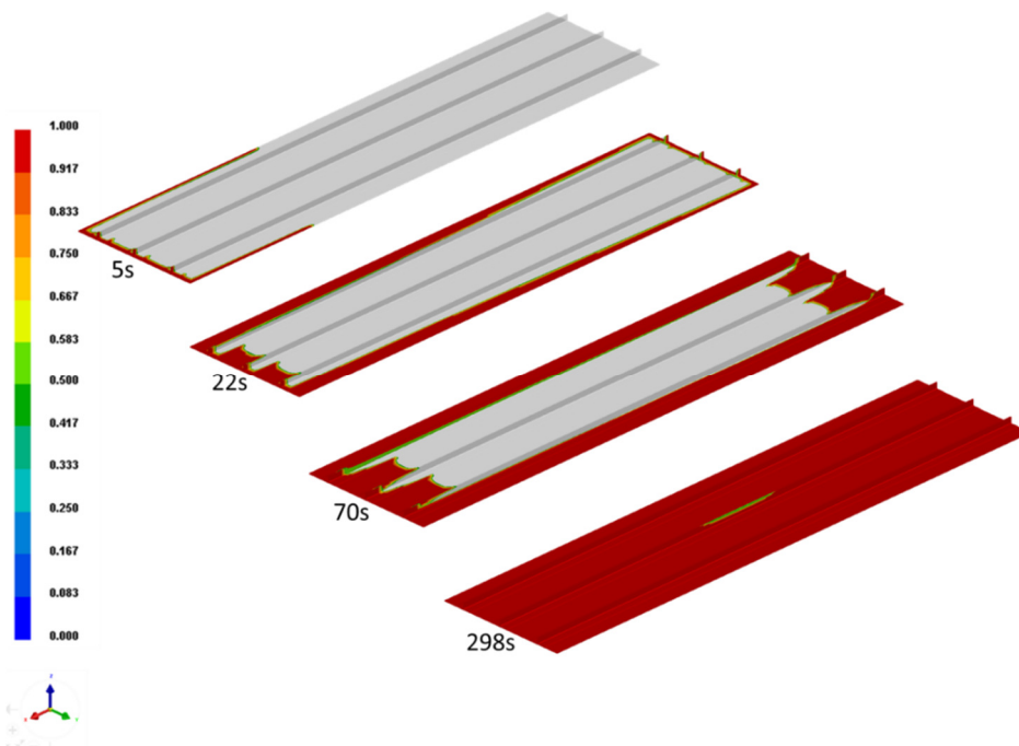
Figure 45: ESI Flow front simulation
