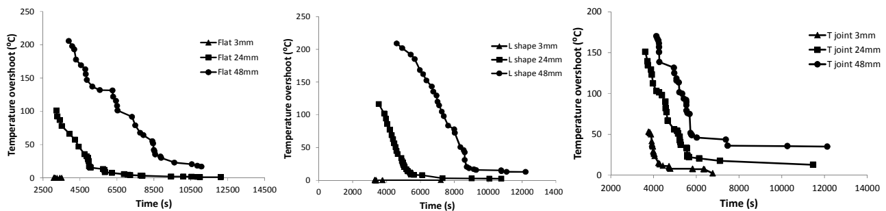
Figure 32: Temperature overshoot – cure time trade off surfaces identified by optimisation: (left) flat panel; (middle) L-profile; (right) T-joint.
