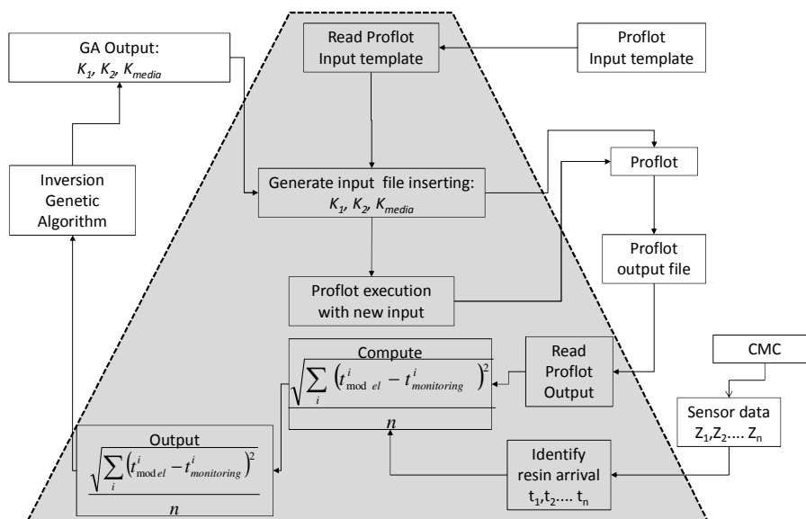
Figure 34: Structure of the interface between Proflot, the inversion GA and CMC
