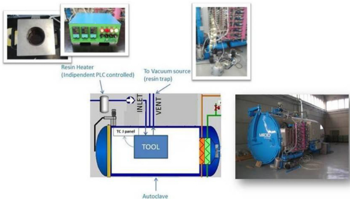
Figure 42: Piaggio infusion test setup
