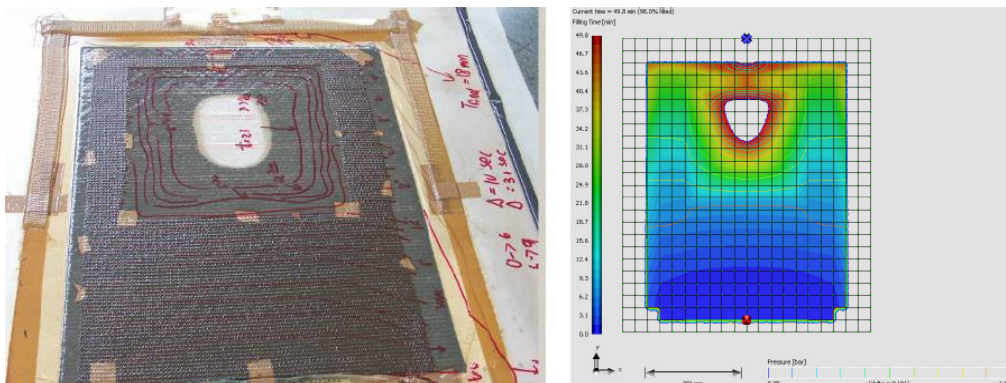
Figure 49: IAI Entrapment coupons and simulation
