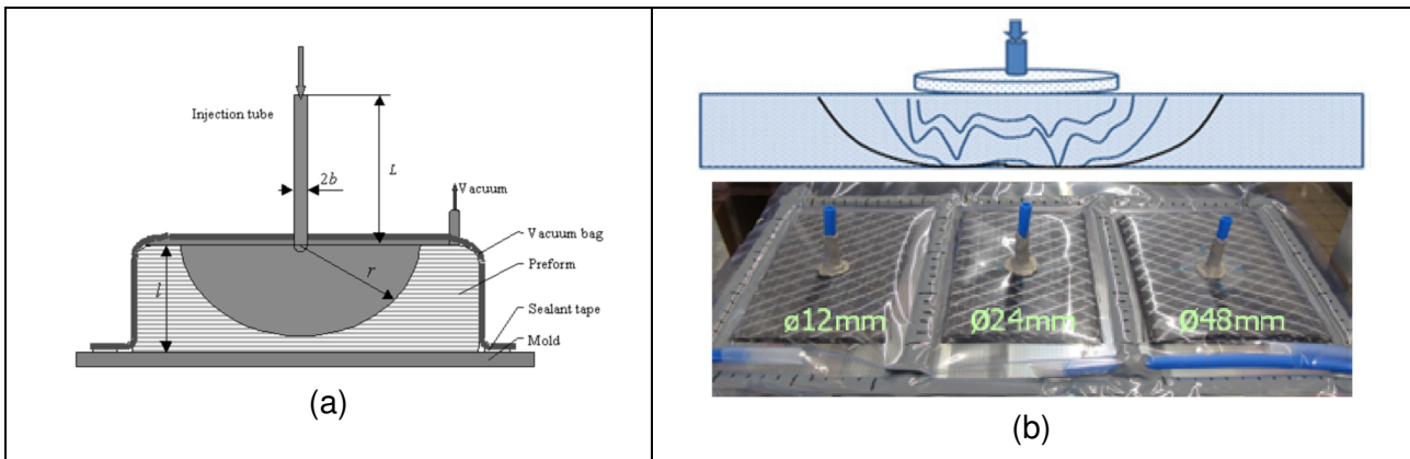
Figure 14: Point infusion test [Nedanov and Advani] (a) and a modified version of the test with distribution patch at the inlet (b)
