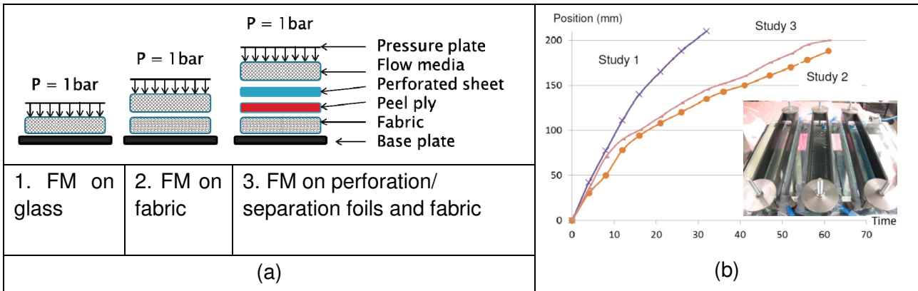
Figure 12: Flow media test configurations (a), flow fronts' propagation comparison (b)
