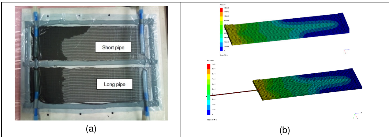
Figure 13: Flow fronts in preforms with different inlet pipes' lengths (a), pressure contour plots from the simulations without and with 1 m inlet pipe (b)
