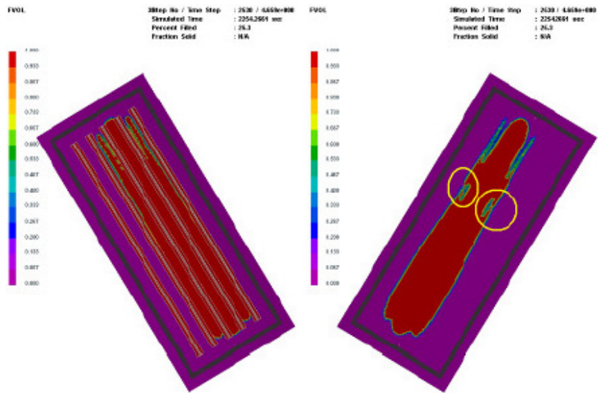
Figure 48 IAI demonstrator – entrapment phenomenon
