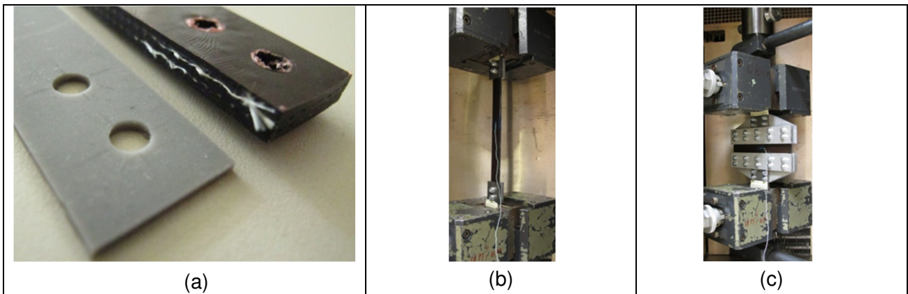
Figure 7: Thin cured elastomer and glass fibre reinforced membranes (a), uniaxial tension specimen (b) and pure shear specimen (c) in the testing machine
