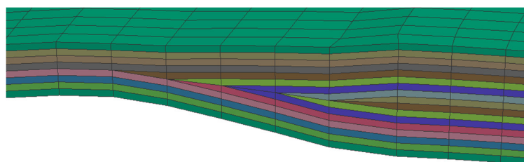
Figure 18: Thickness variation due to layer end (layers drop-off)
