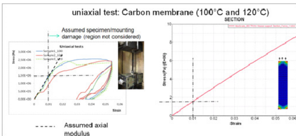
Figure 8: Membrane uniaxial tension test and simulation (orth. viscoelastic shell (Mat. model 140))
