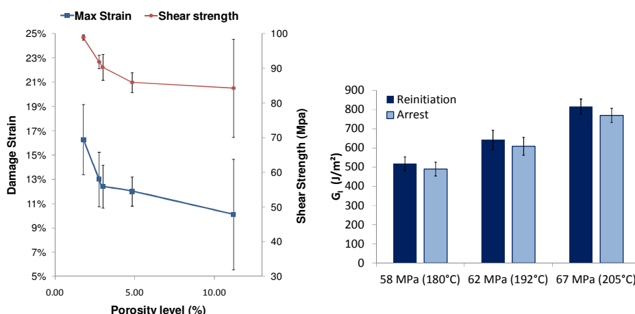
Figure 29: Effects of porosity on shear properties (left); effects of residual stress on delamination toughness (right).
