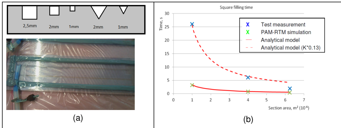
Figure 10: Tested race track geometries and view of the test (a), comparison of flow propagation from test and analytical/numerical models
