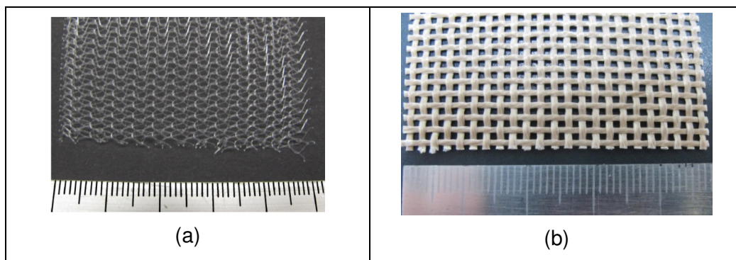
Figure 11: Two types of flow media tested: IFB (XS6262-003 „X60“X650FT) (a), Daher (Daher specification) (b)
