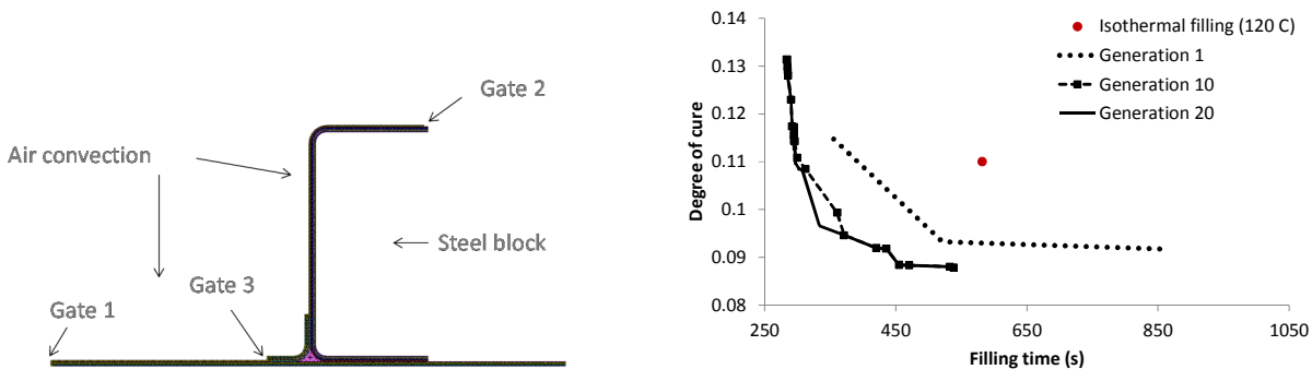
Figure 31: C-section model built in PAMRTM (left); evolution of the Pareto set (right).
