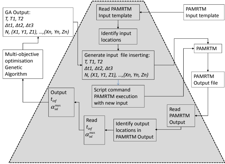
Figure 30: Structure of the interface between PAM-RTM and the multi-objective optimiser
