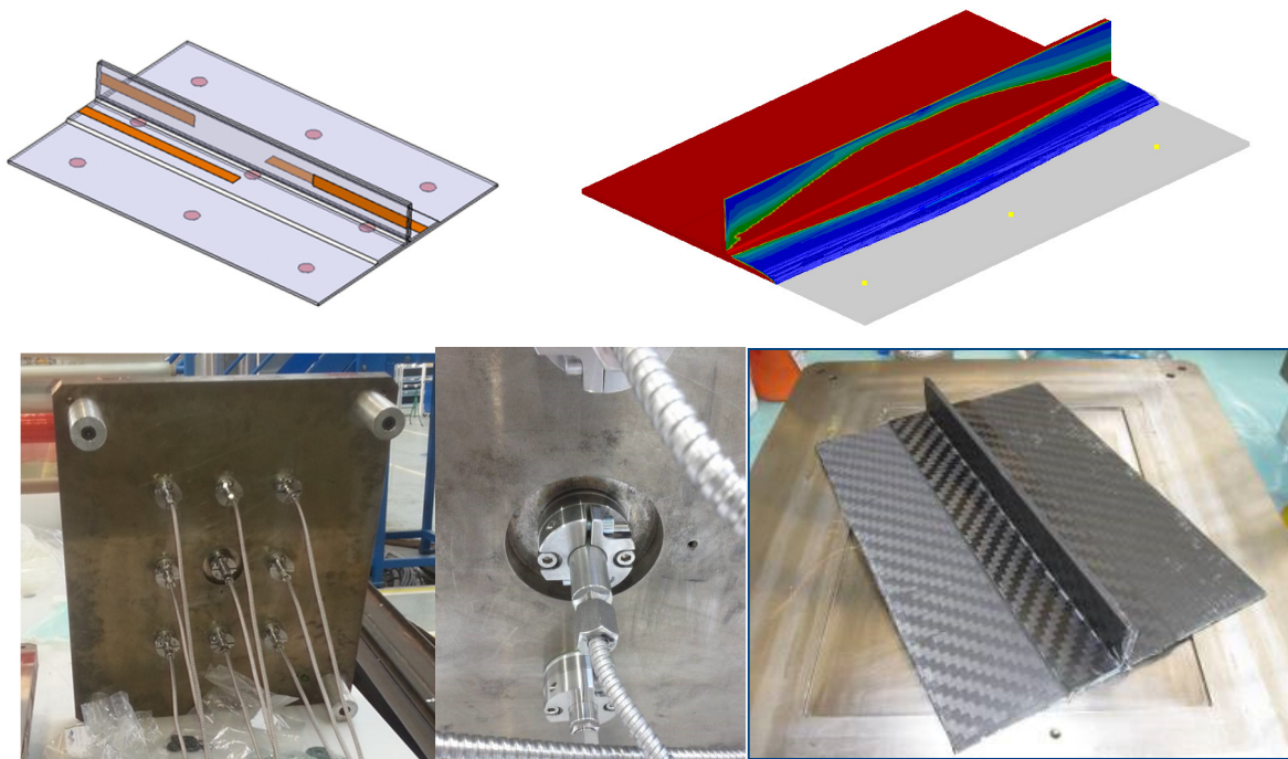
Figure 36: DAHER small scale singularity (panel with T stiffener)
