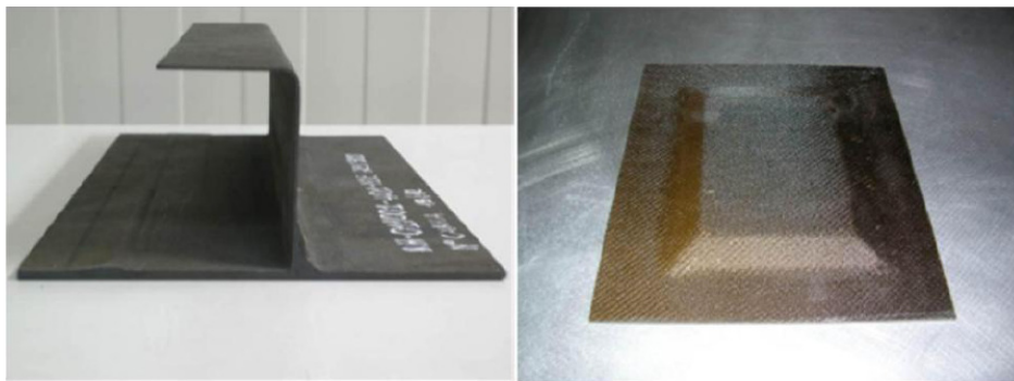
Figure 39: Piaggio small scale infusion demonstrators (C stiffener monolithic demonstrator and sandwich demonstrator)
