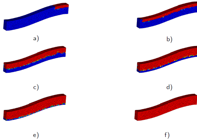
Figure 16: 3D simulation of the resin injection with draining filling, K=1e^{-9} \text{ m}^2
