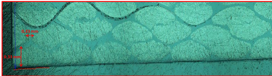
Figure 28: Typical micrograph of an intersection at the surface of the laminate.
