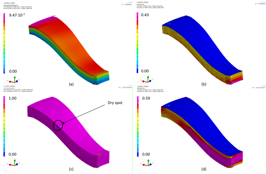
Figure 20: 3D complex shape simulation: (a) displacement field after initial compaction, (b) porosity (1-Vf) after initial compaction, (c) final filling factor, (d) final resin Vf
