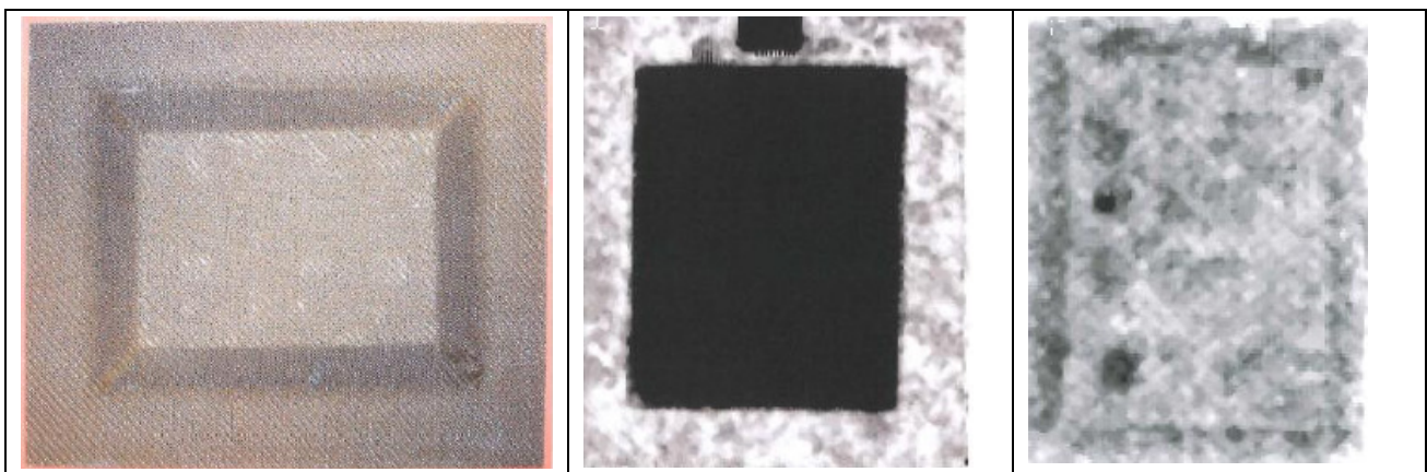
Figure 40: Sandwich small scale demonstrator (a) and artificial defect distribution, C-scan monolithic area (b) and sandwich area (c)
