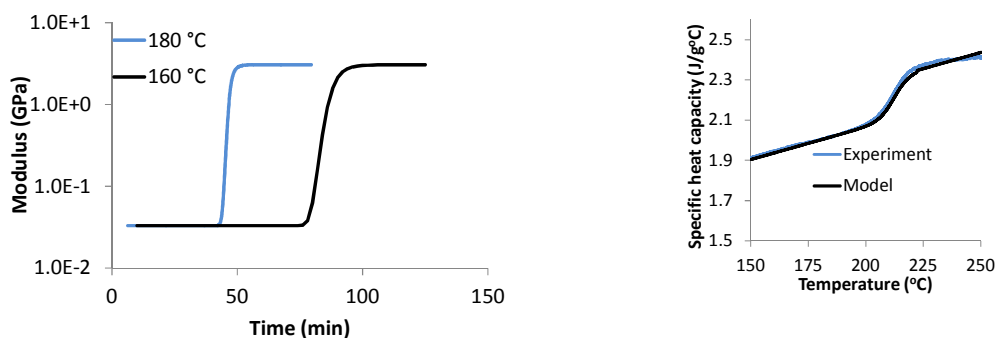
Figure 25: Examples of material sub-models: (left) development of modulus under isothermal conditions and (right) heat capacity as a function of temperature.
