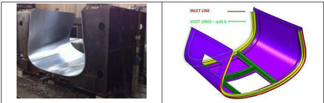
Figure 41: Belly fairing demonstrator
