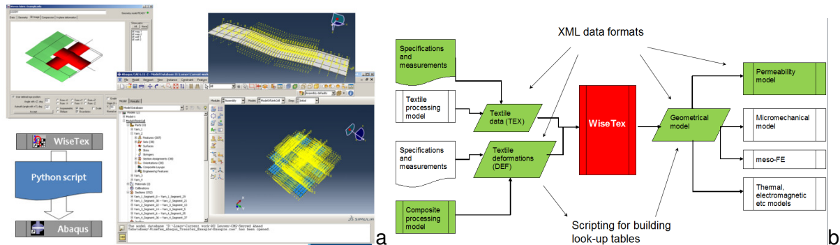
Figure 5: New meso-scope models developed in KU Leuven; (a) transformation of geometric WiseTex model in Abaqus; (b) data flow in the new version of WiseTex software
