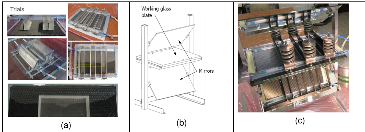
Figure 9: Infusion tests: Trials (a), schematic view of a test rig (b), test rig (c)
