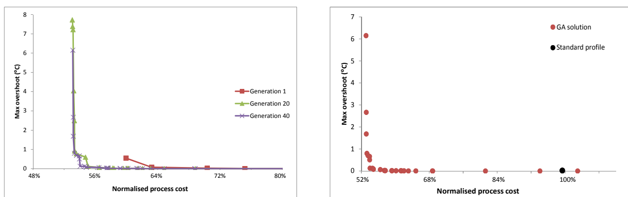
Figure 24: Evolution of the Pareto front in the cost/performance optimisation of an industrial component (left); comparison of the final Pareto front in the cost/performance optimisation and the standard profile (right).
