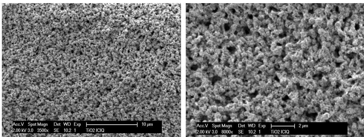
Figure 1.2. Scanning electron microscopy ( SEM) digital picture of a benchmark TiO 2 film. The film thickness was 7.1 μm + 4.7 μm scatter paste.
