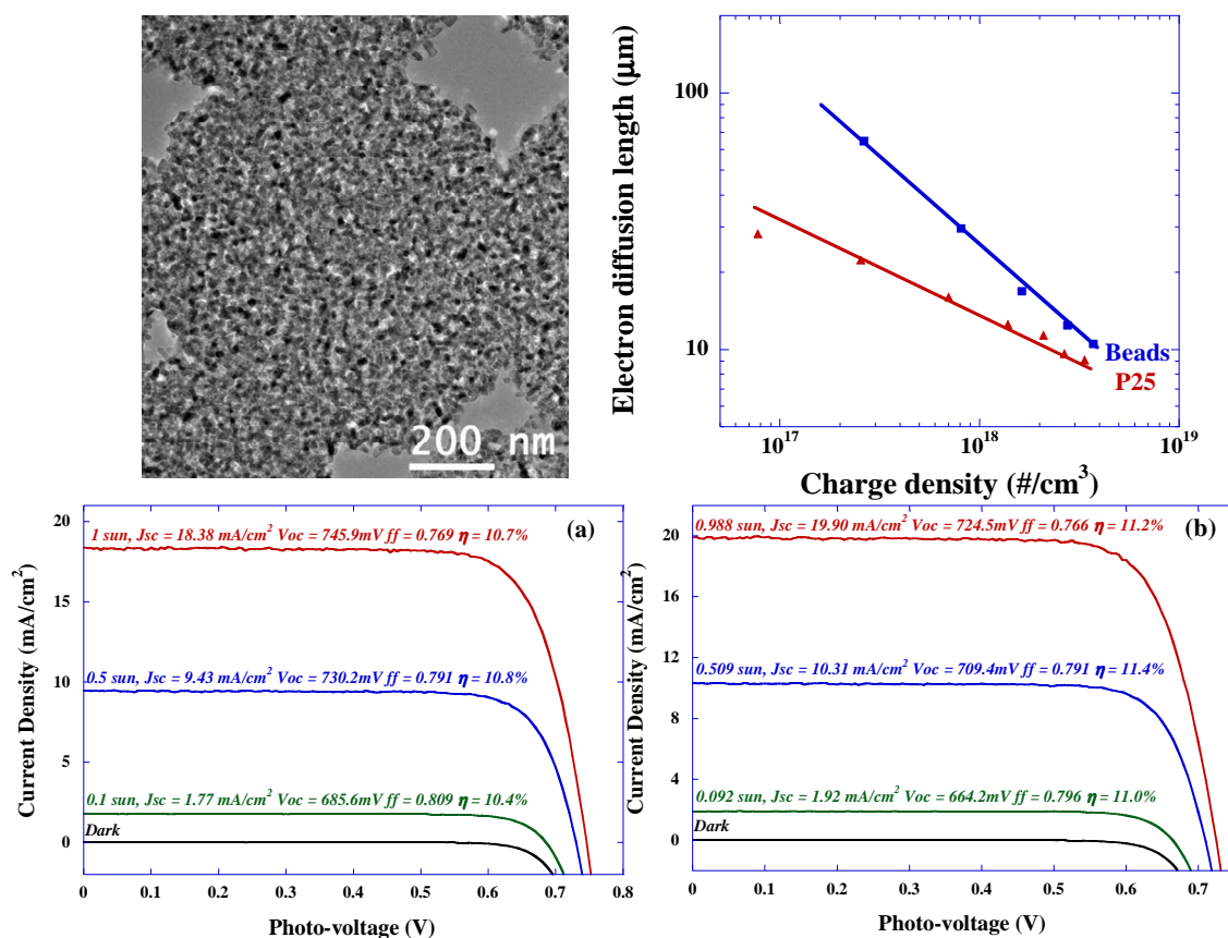
Figure 2.4. TEM micrograph of beads of \text{TiO}_2 , evolution of electron diffusion length as a function of charge density for the beads compared to the benchmark P25 particles, ( J - V ) characteristics of C106 dye in combination with a single type layer of beads (a) or using a triple layer configuration 20nm \text{TiO}_2 nanoparticles / Beads / 400 nm sized \text{TiO}_2 scattering particles.
