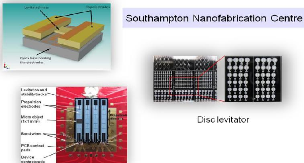
Figure 34: Micro-component levitators
