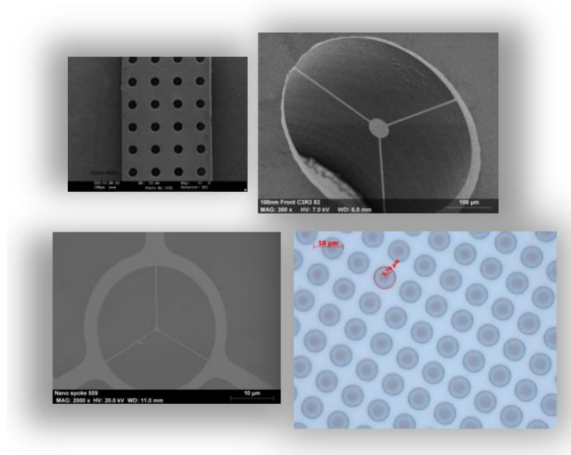
Figure 29: 2D wafer based micro-fabrication
