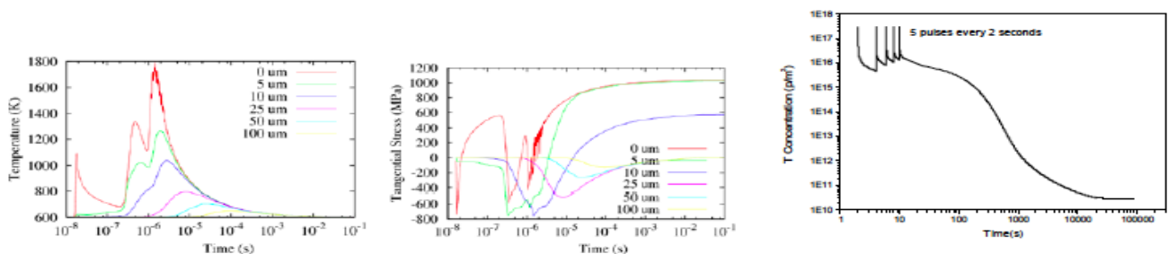
Figure 50: Temperature, Stress and Tritium retention in a Burst Mode operation
