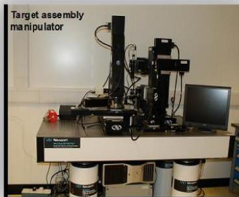
16-axis micromanipulator
