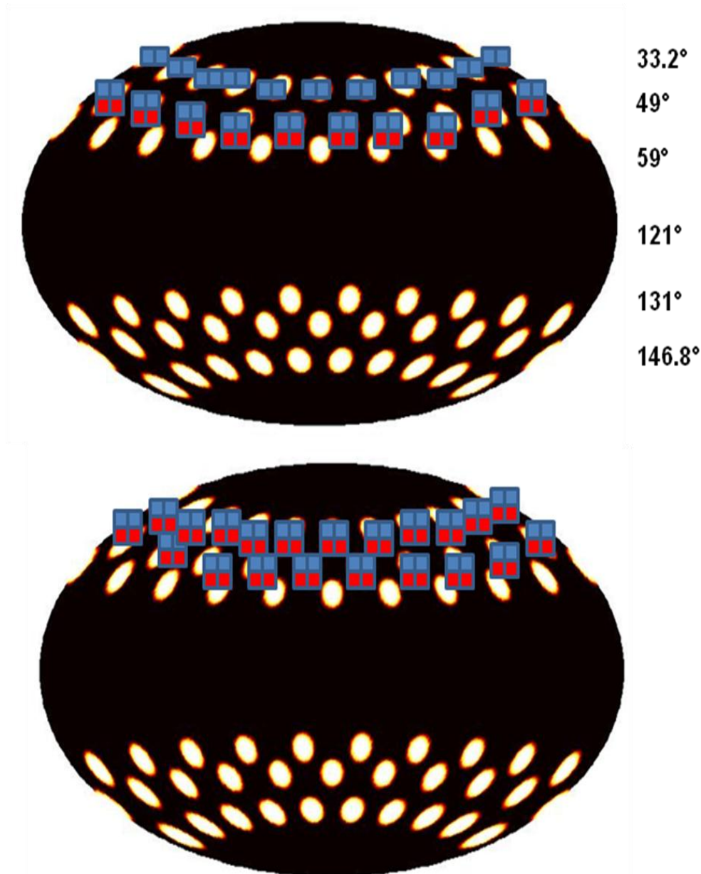
Figure 15: Polar drive irradiation on 160 beams LMJ. Compression will use half of the 33° beams (lower beams – 33a) and all 49° beams, splitted into 2 rings (49°a &b). All beams are repointed and defocused. The shock will be driven by all beams.
