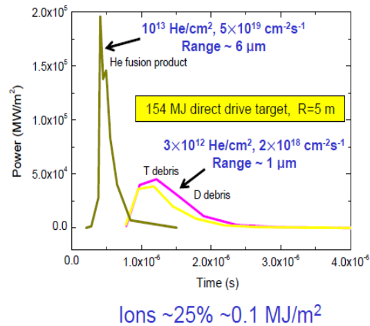
Figure 49: Power from Ion species in the wall at 5 m radius
