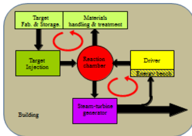
Figure 36: Laser Energy Reactor Global Structure
