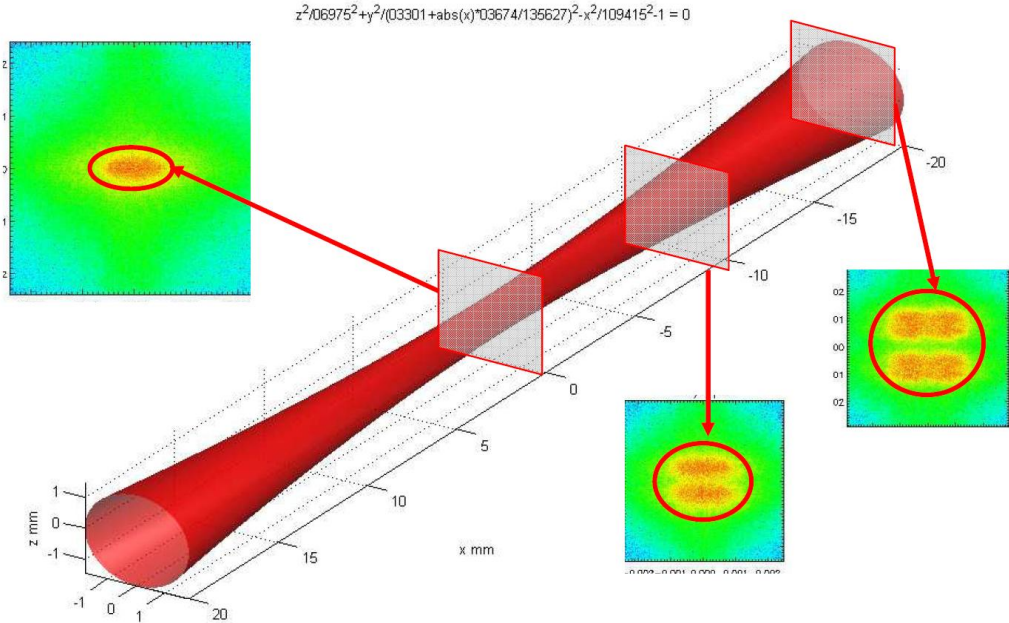
Figure 17: Distribution of intensity at different distances from best focus for a LMJ quad
