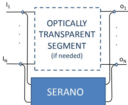
Figure 17: BV-OXC with SERANO bypassing architecture (high level).
