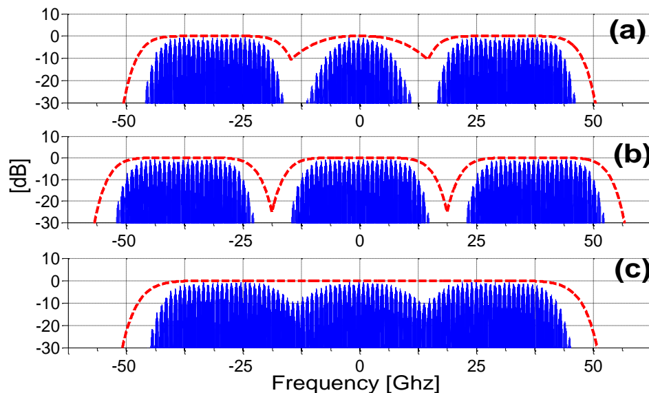
Figure 4: DP-QPSK signals and actual LCoS filter shapes.
