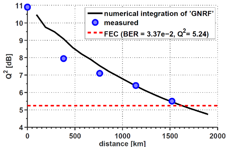
Figure 8: Squared Q-factor as a function of the transmission distance. The blue dots show the experimentally obtained results, while the black curve shows the predicted results by the Gaussian noise model. Graph from [Rahman-PhSw15].
