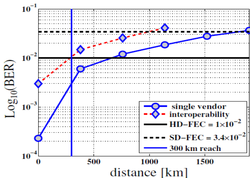
Figure 5: BER vs. distance for single vendor and inter-operability assuming HD or SD-FEC.
