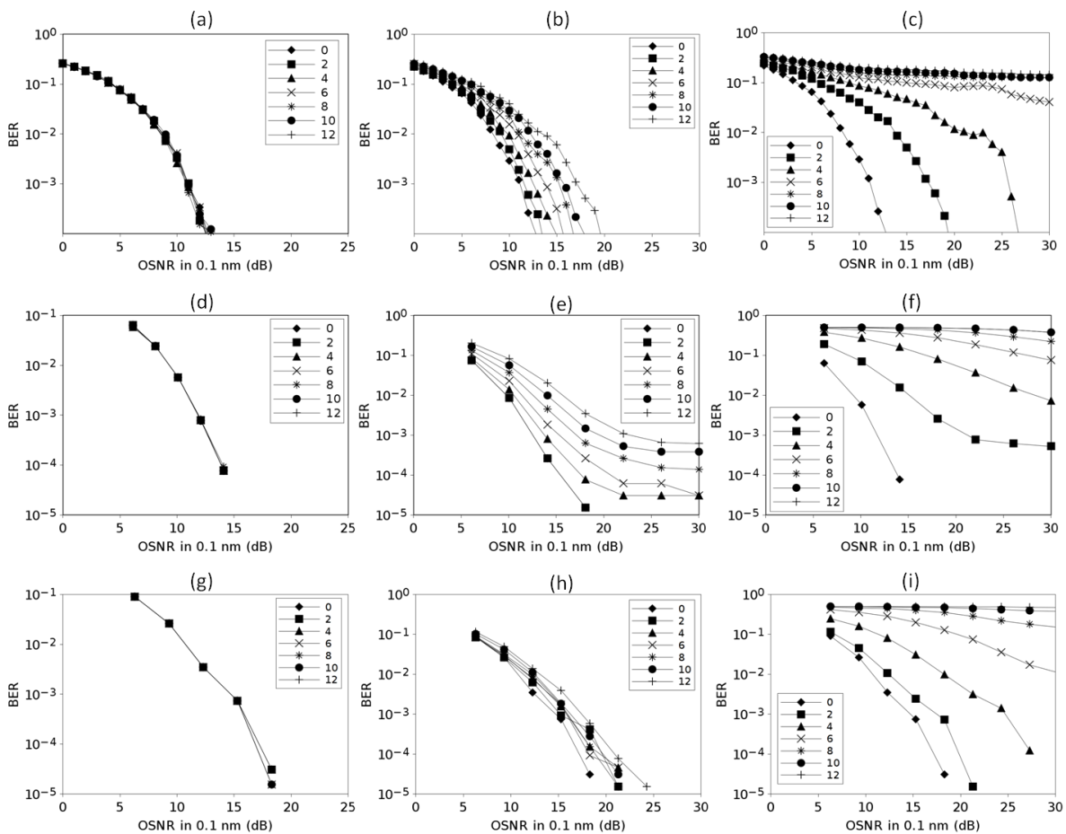
Figure 27: Simulation results for a standard IM/DD system (a, b, c), the OFDM SSB transceiver without bit loading (d, e, f) and with bit loading (g, h, i) after concatenation of different filters featuring bandwidths of 50 GHz (a, d, g), 25 GHz (b, e, h) and 12.5 GHz (c, f, i).
