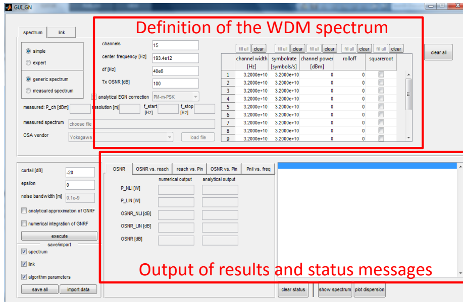
Figure 7: Screenshot of the implemented GUI which acts as an input frontend for the Gaussian noise model.
