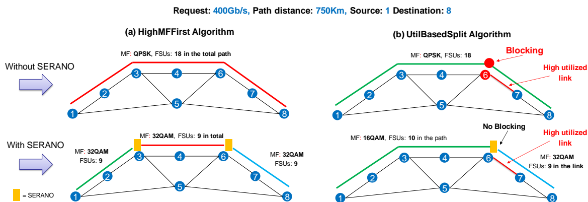
Figure 19: Example of HighMFFirst and UtilBasedSplit algorithms.
