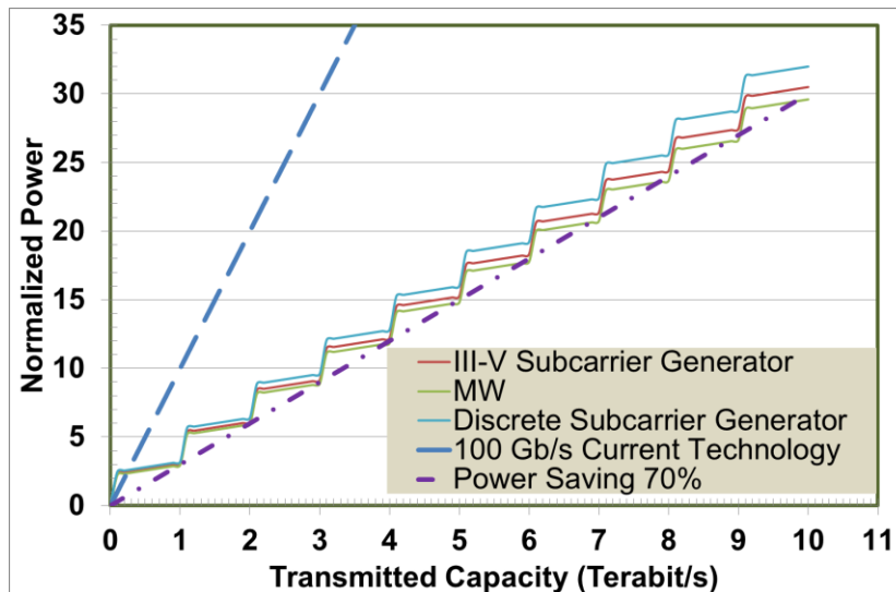
Figure 26: Power Consumption curves for three design options of the subcarrier generation module: discrete lasers on board of the line card, i.e. DFB lasers; monolithically integrated lasers in III-V material, i.e. Indium-phosphide; multi-wavelength, MW, source realized starting from a single laser as in [Sambo-JOCN2014].
