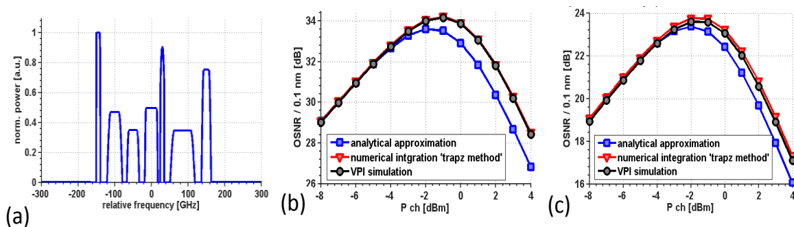
Figure 6: Spectra of investigated WDM signals and resulting simulation results. (a) shows the WDM spectrum for an arbitrarily chosen spectral shape. (b) and (c) show the effective OSNR (including linear ASE noise and nonlinear interference noise) as a function of the fibre input power per channel. Each graph shows a comparison between the different investigated numerical methods. (b) shows the results for a single span, while (c) shows the results for a 10 span transmission. Figure from Deliverable D2.3.
