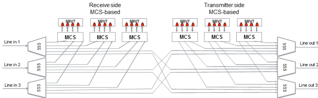
Figure 2: ROADM with Add&Drop modules based on multicast switches.
