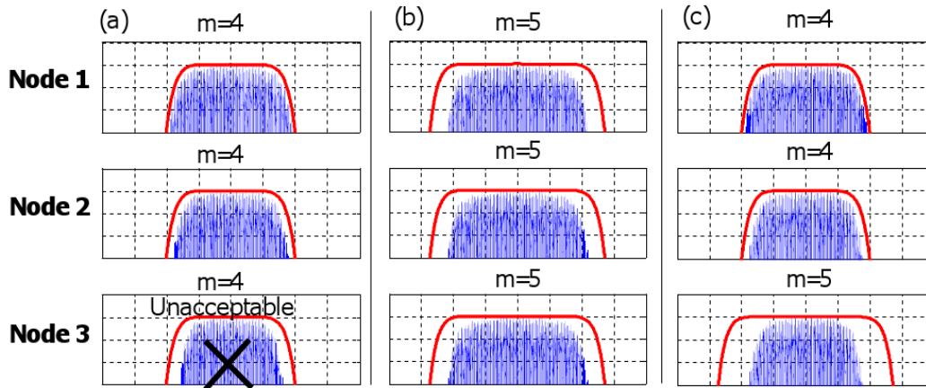
Figure 3: Traditional cascaded filtering with m=4 (50GHz, unacceptable filtering effects) (a); or m=5 (62.5GHz, acceptable filtering effects) (b); and Differentiated Filter Configuration (spectrum saving and acceptable filtering effects) (c).
