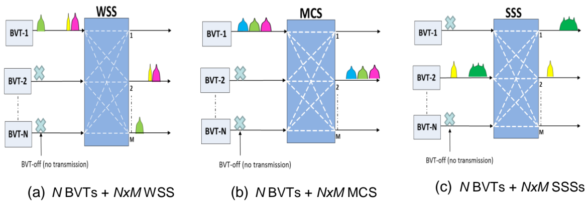
Figure 13: Different add/drop network subsystem with BVT designs.
