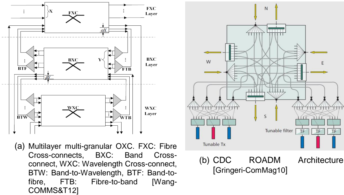
Figure 15: Traditional OXC and ROADM Architectures.
