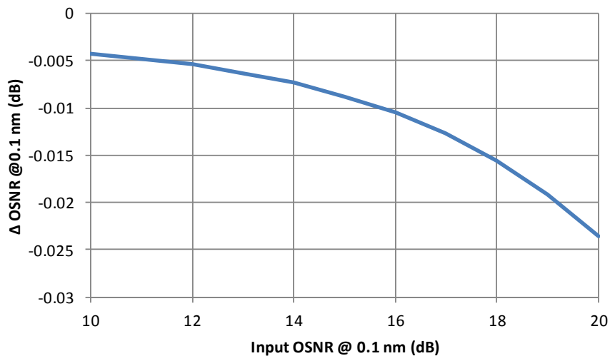
Figure 24: \Delta OSNR as a function of input OSNR.
