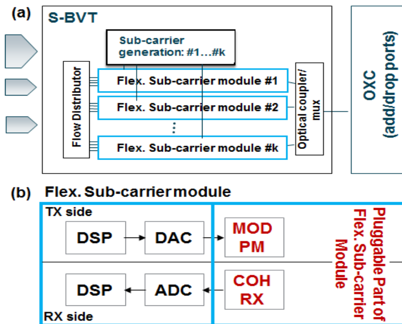
Figure 9: S-BVT architecture (a); Sub-carrier module (b).
