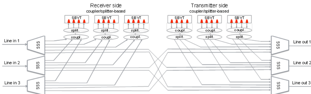
Figure 1: ROADM with Add&Drop modules based on coupler and splitter.
