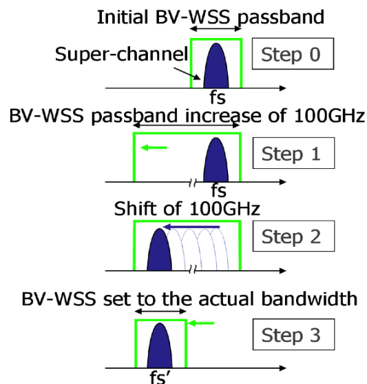
Figure 25: Filters enabling push-pull.
