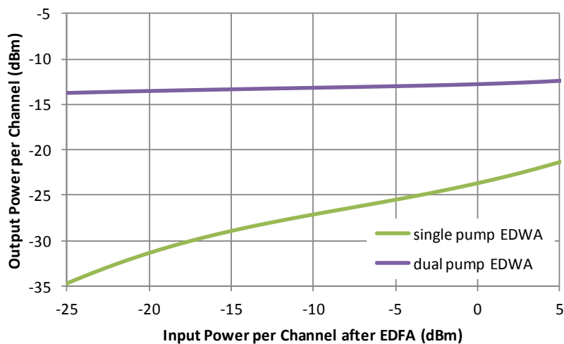
Figure 22: Output power per channel as a function of the input power per channel using 2 EDWA stages (1:8 splitters).
