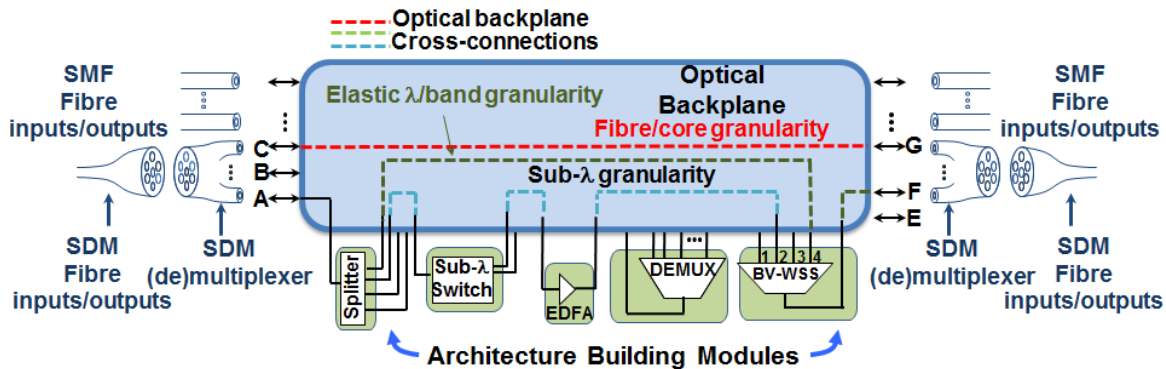
Figure 16: Architecture-on-Demand Node.
