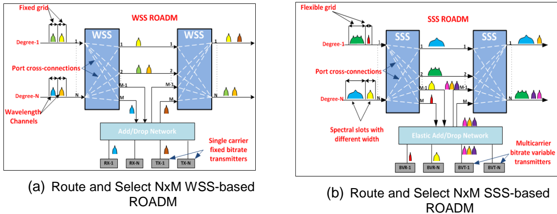
Figure 12: ROADM architectures for flexibility measurement. Route and Select NxM (a) WSS-based ROADM and (b) SSS-based ROADM.
