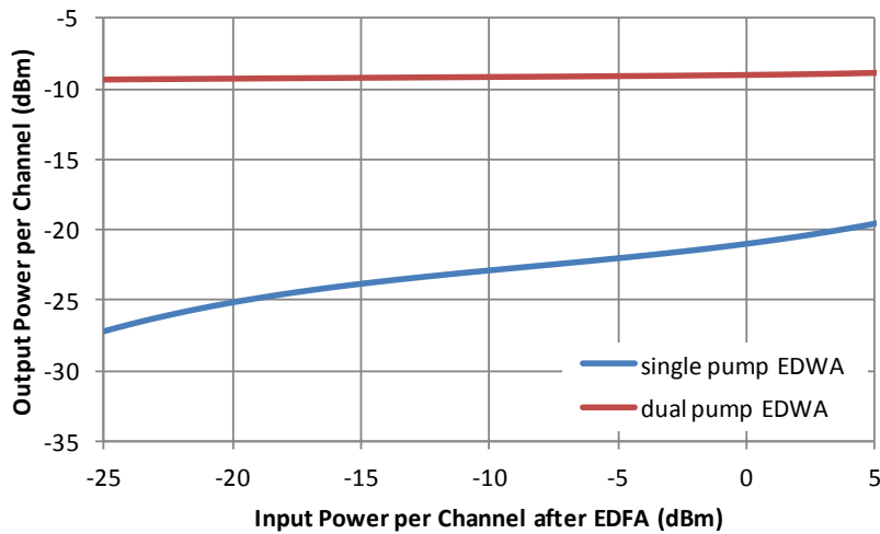
Figure 23: Output power per channel as a function of the input power per channel using 2 EDWA stages (1:4 splitters).
