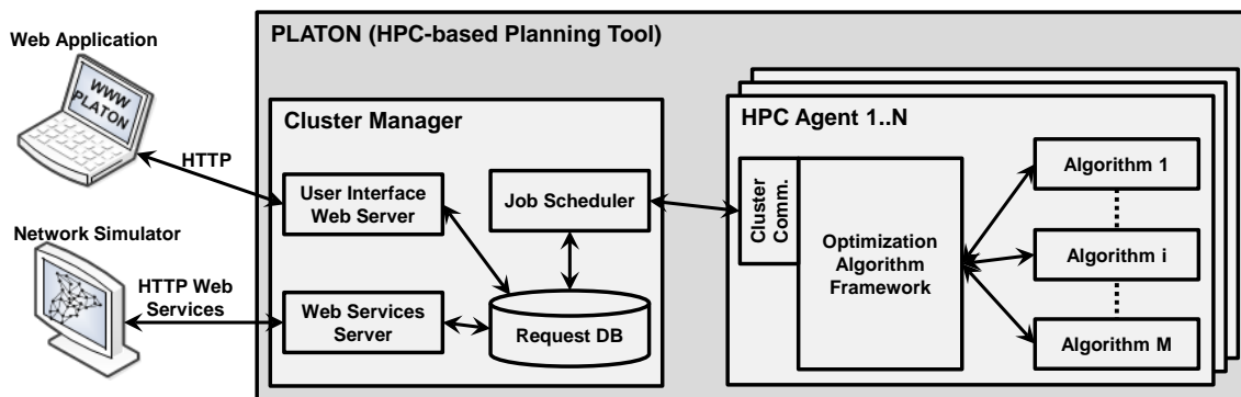
Figure 28. PLATON Architecture – Off-line planning scenario
