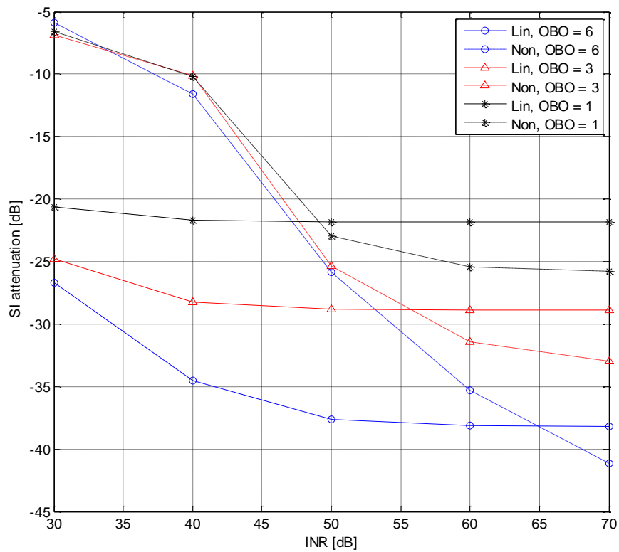
Fig. 2.8. Performances of linear and two-step method self-interference cancellation for a frequency selective self-interference channel.
