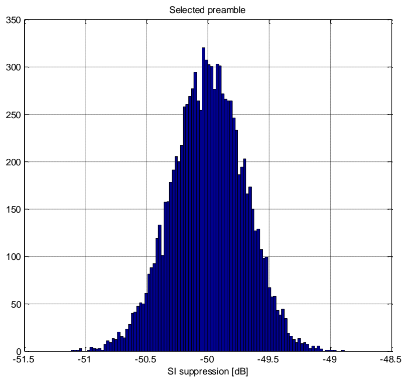
Fig.2.12. Hammerstein based self-interference cancellation with preselected preamble, 5th order nonlinearity, OBO=6 dB, INR=50 dB.
