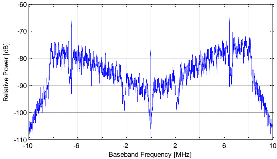
Fig. 5.3. Spectrum of the received signal (self-interference).
