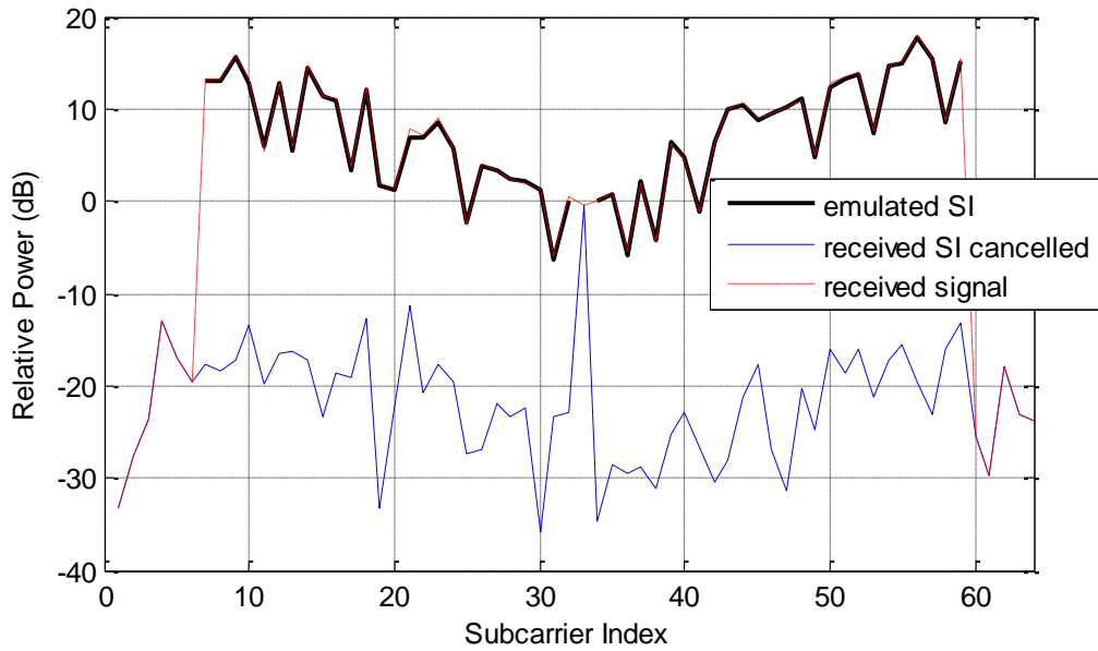
Fig. 5.6. SI cancellation at subcarrier domain.
