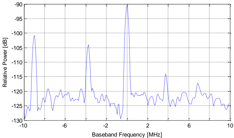
Fig. 5.4. Spectrum of the noise-only received samples.
