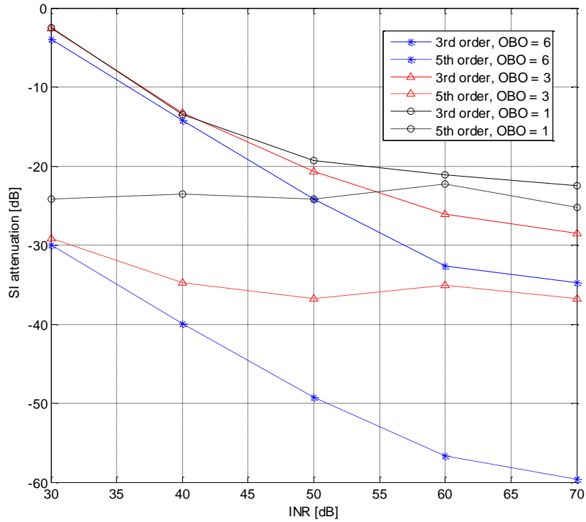
Fig.2.9. Hammerstein model based self-interference cancellation with random preamble.
