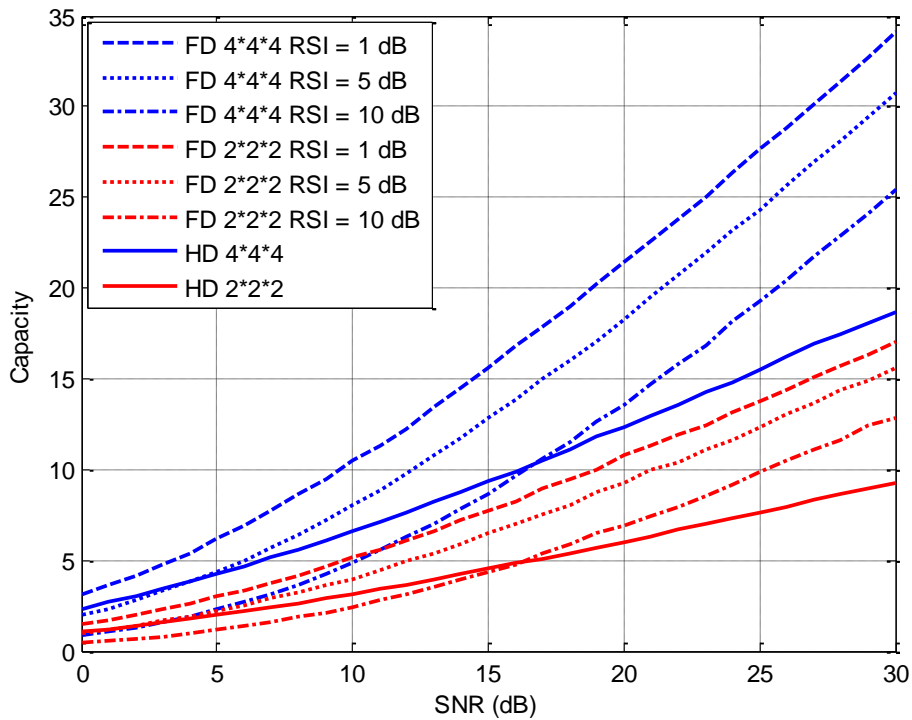
Figure 4.12. Capacity of full-duplex relay link with imperfect self-interference cancellation and those of the half-duplex relay link.
