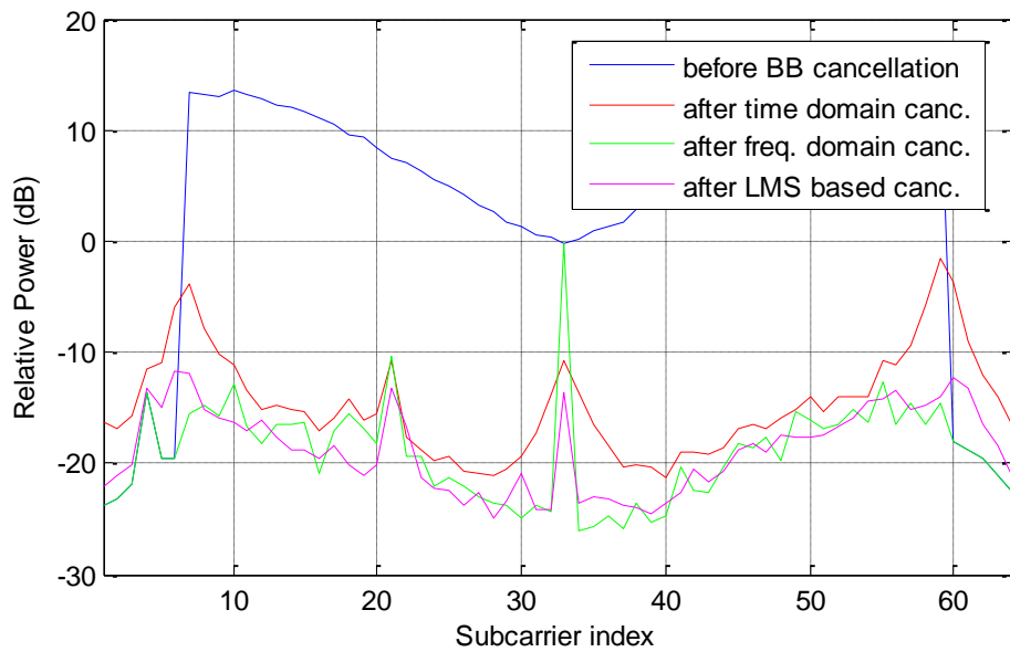
Fig. 5.9. Average SI cancellation per subcarrier.
