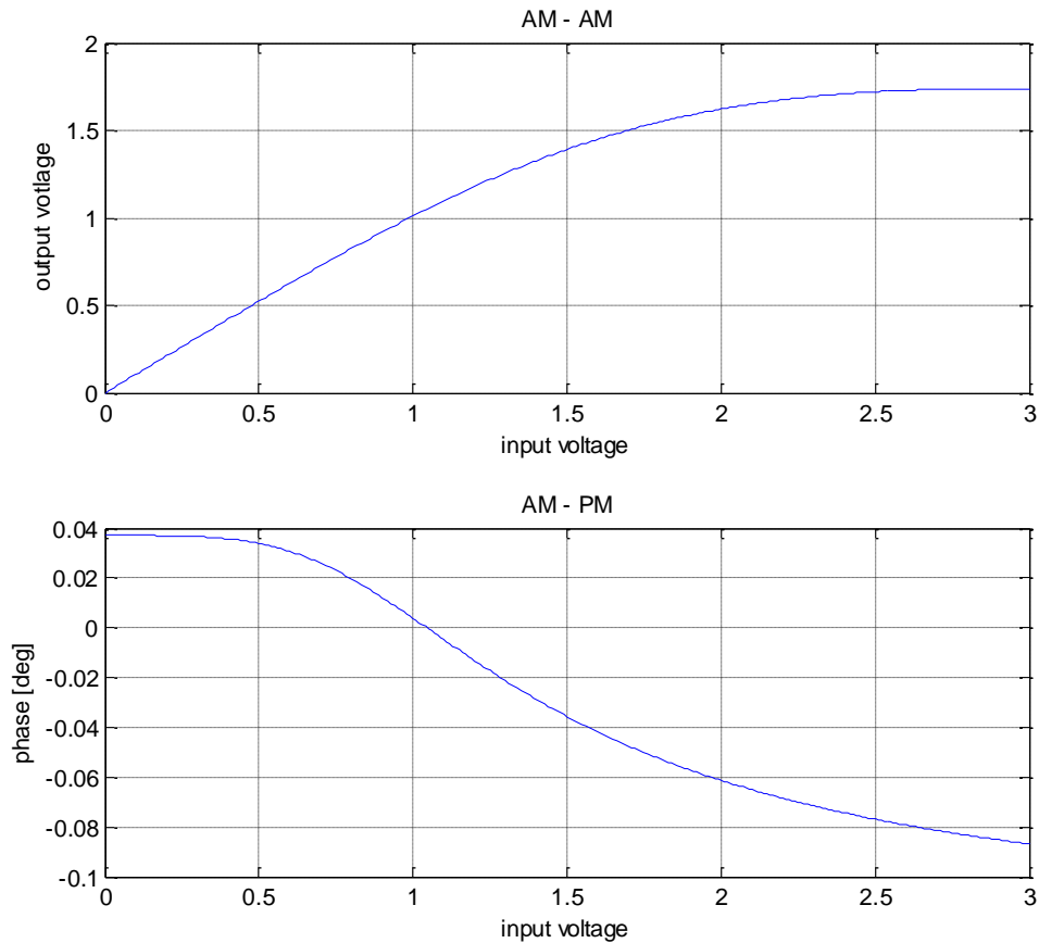
Fig. 2.3. Power amplifier model's amplitude and phase response.
