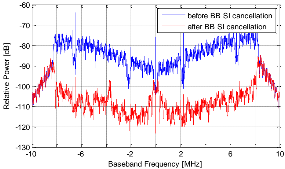
Fig. 5.7. Self-interference spectrum before and after time-domain self-interference cancellation.
