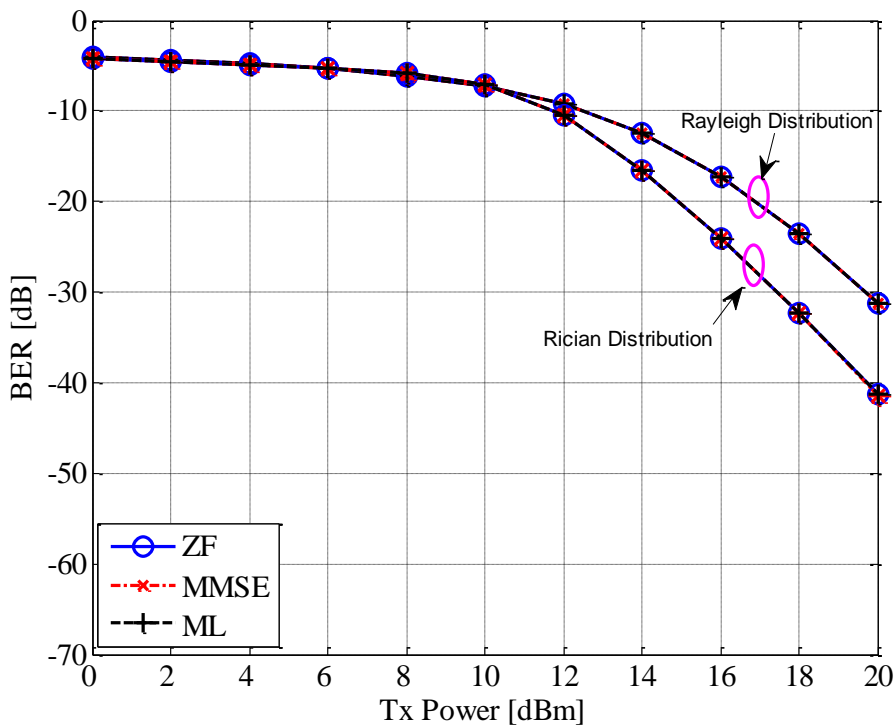
Fig. 3.5 The comparison BER performance between the different detection schemes with the Rayleigh and Rician distributed residual self-interference in OFDMA system.
