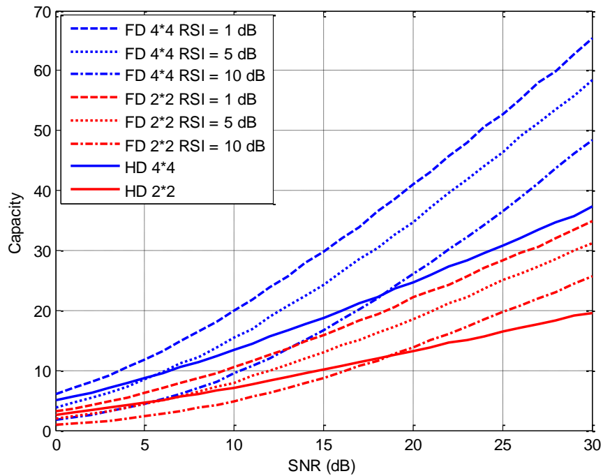
Figure 4.9. Capacity of full-duplex point-to-point MIMO system with imperfect self-interference cancellation and those of the half-duplex MIMO system.
