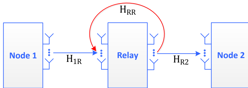
Figure 4.10. Block diagram of the full-duplex relay link.
