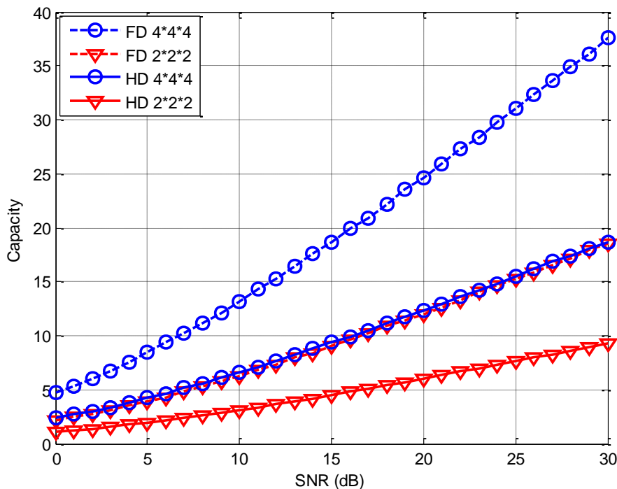
Figure 4.11. Capacity of full-duplex relay link with perfect self-interference cancellation and those of the half-duplex relay link.
