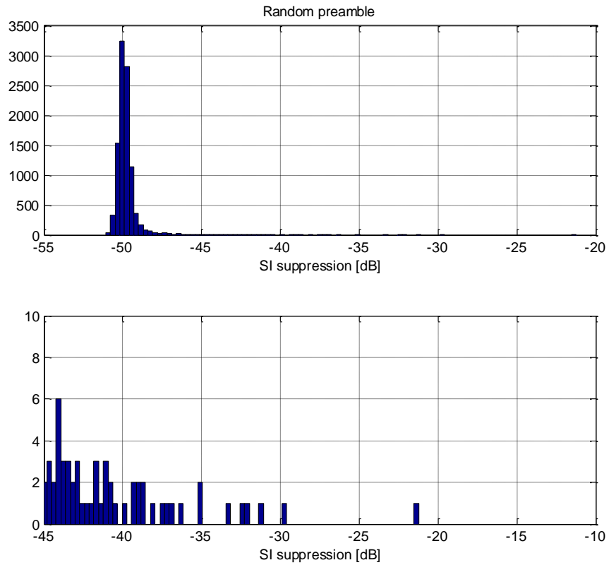
Fig. 2.11. Hammerstein based self-interference cancellation with random preamble, 5th order nonlinearity, OBO=6, INR=50 dB.
