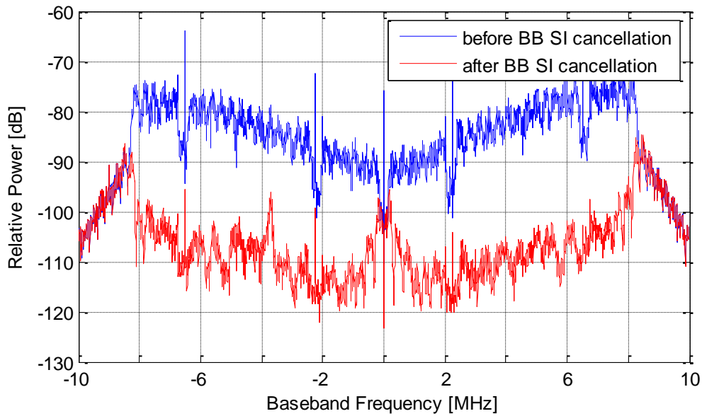
Fig.5.8. Self-interference spectrum before and after self-interference cancellation using the LMS algorithm for self-interference channel estimation with time-domain cancellation.
