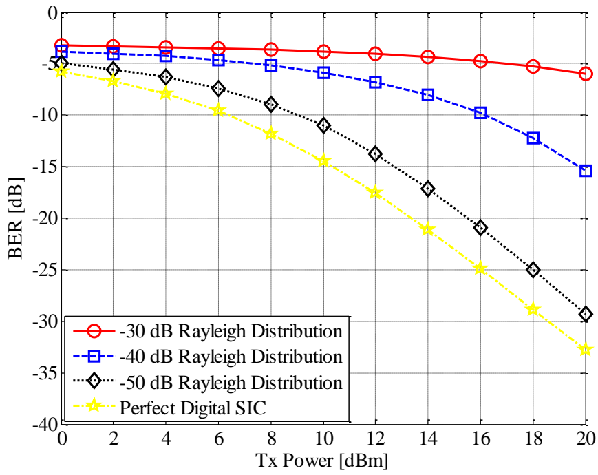
Fig. 3.6 full-duplex SC-FDMA system BER performance for different residual self-interference (Rayleigh Distribution) powers.
