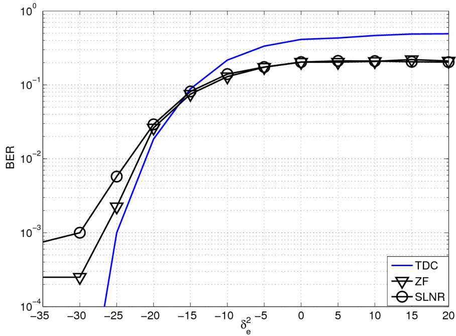
Figure 4.4. Impact of the self-interference channel estimation error on the BER performance of the full-duplex MIMO system using digital self-interference cancellation, ZF or SLNR-based precoding, where M_i = 4, N_i = 2, N_j = 2, \sqrt{\eta_i} = 20 dB, SNR = 10 dB.
