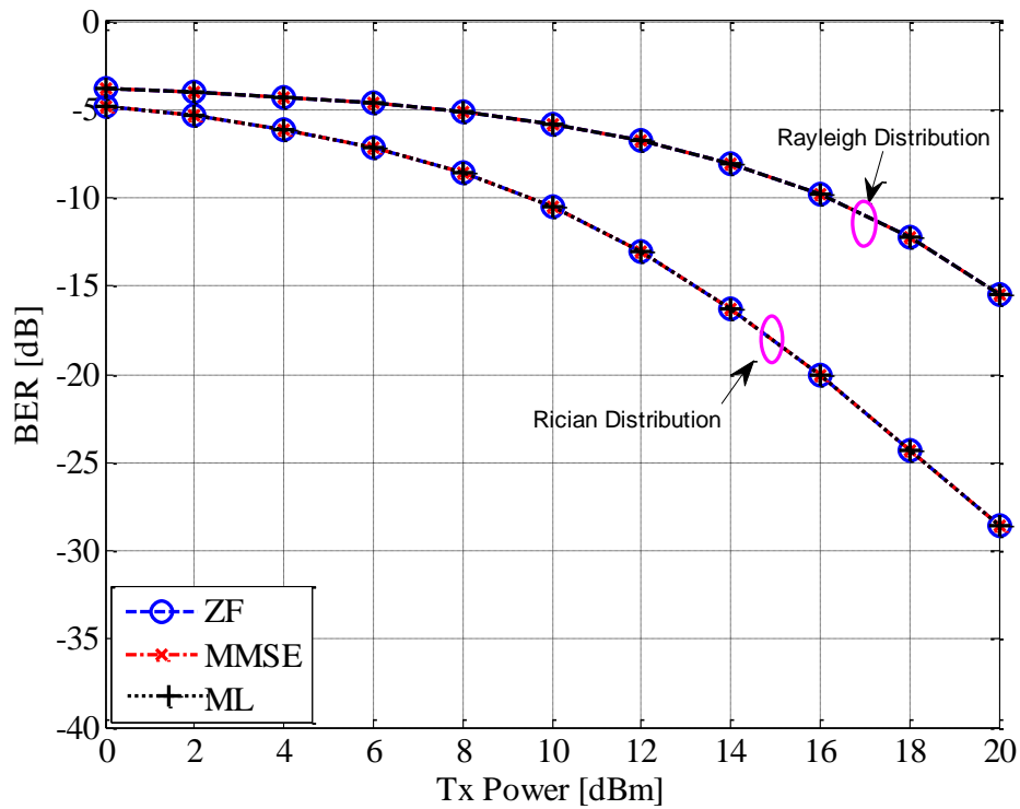
Fig. 3.8 The comparison BER performance between the different detection schemes with the Rayleigh and Rician distributed residual self-interference in SC-FDMA system.
