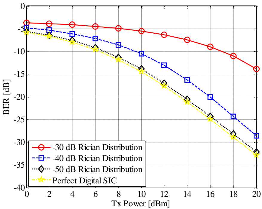
Fig. 3.7 full-duplex SC-FDMA system BER performance for different residual self-interference (Rician Distribution) powers.
