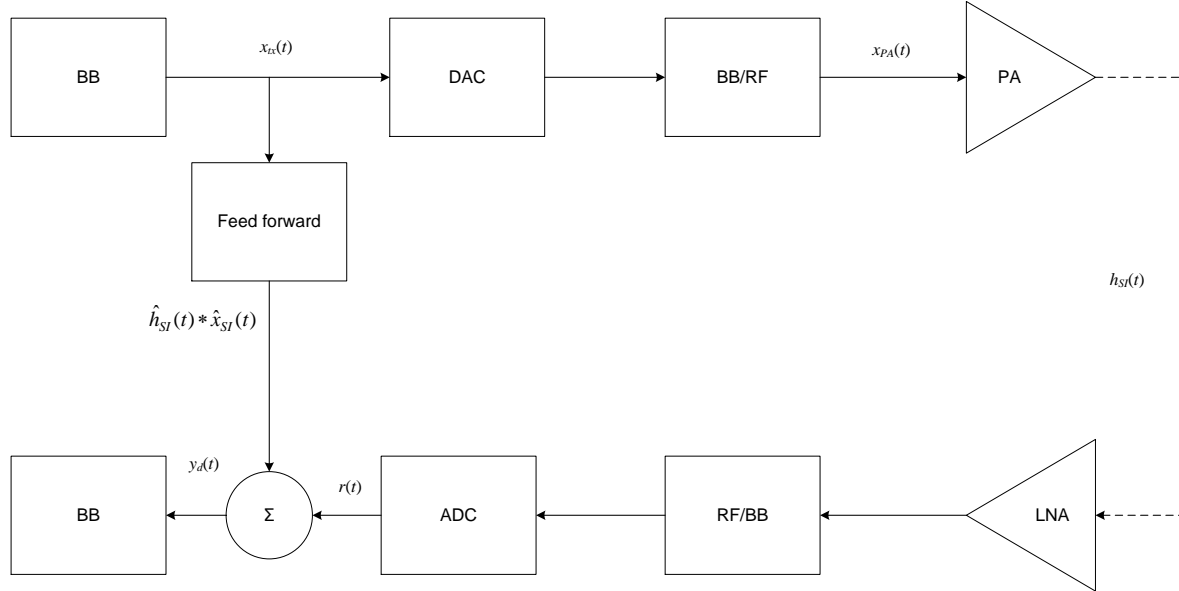
Fig. 2.1. Baseband self-interference cancellation in full-duplex transceiver.
