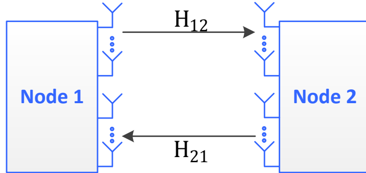
Figure 4.2. Block diagram of the full-duplex MIMO system with perfect self-interference cancellation, which works like a half-duplex system.
