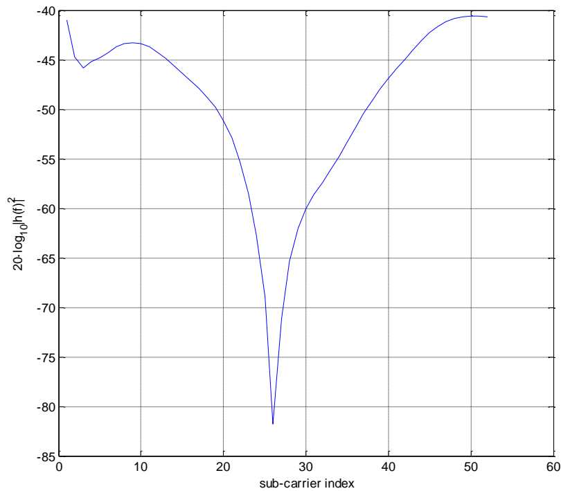
Fig. 2.5. Frequency response of the measured self-interference channel.
