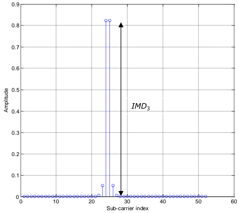
Fig. 2.4. Power amplifier two-tone test.
