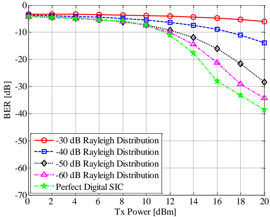
Fig. 3.3 full-duplex OFDMA BER performance for different residual self-interference where residual self-interference is assumed random variable with Rayleigh distribution.
