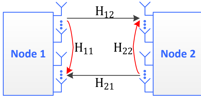
Figure 4.1. Block diagram of a full-duplex MIMO system.
