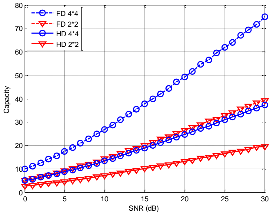
Figure 4.8. Capacity of full-duplex point-to-point MIMO system with perfect self-interference cancellation and those of the half-duplex MIMO system.
