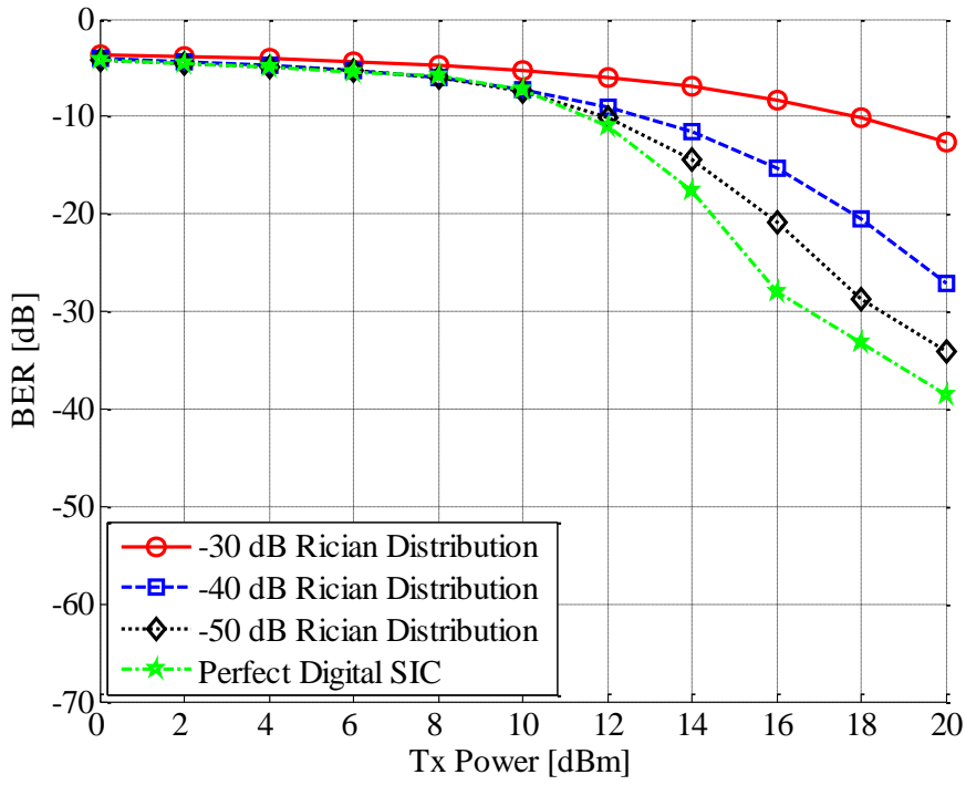
Fig. 3.4 full-duplex OFDMA BER performance for different residual self-interference where residual self-interference is random variable with Rice distribution.
