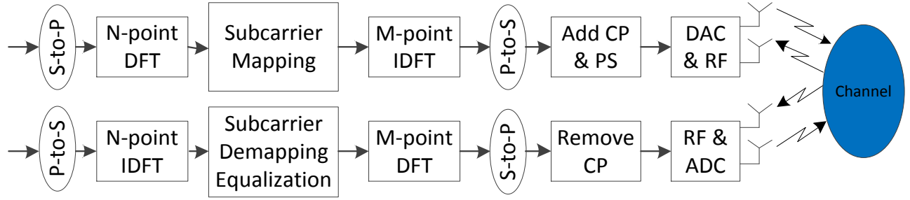
Figure 3.2. System model of SC-FDMA for full-duplex systems.
