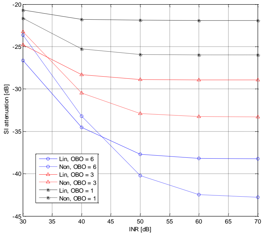
Fig.2.7. Performances of linear and two-step methods self-interference cancellation for a frequency flat self-interference channel.
