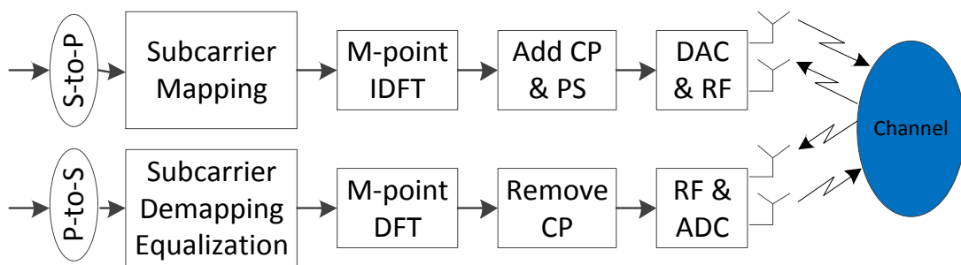
Figure 3.1. System model for OFDMA for full-duplex system.
