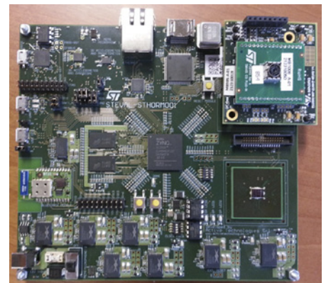
P2012/STHORM evaluation board
