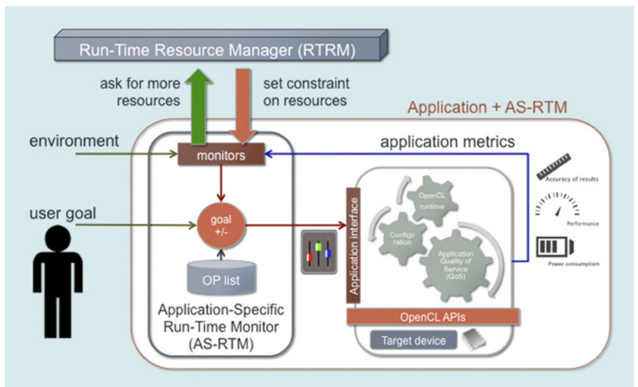
Application adaptivity through AS-RTM and RTRM
