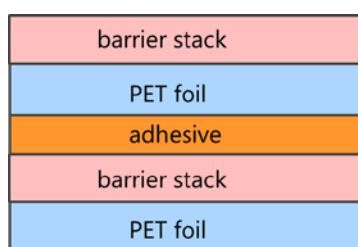
Figure 3 Barrier stack laminate optimized in TREASORES. Electrode deposition is subsequently carried out on the top barrier stack.
