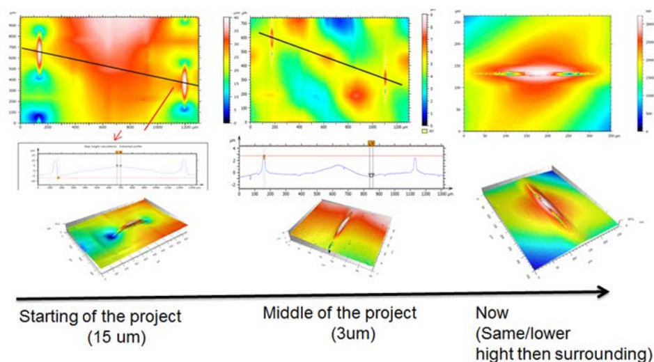
Figure 5 Reduction of surface waviness of fabric electrodes during project progress.
