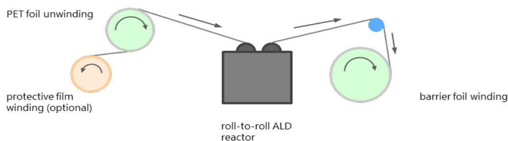
Figure 4 Schematic drawing of the inline roll-to-roll fabrication equipment developed in TREASURES.
