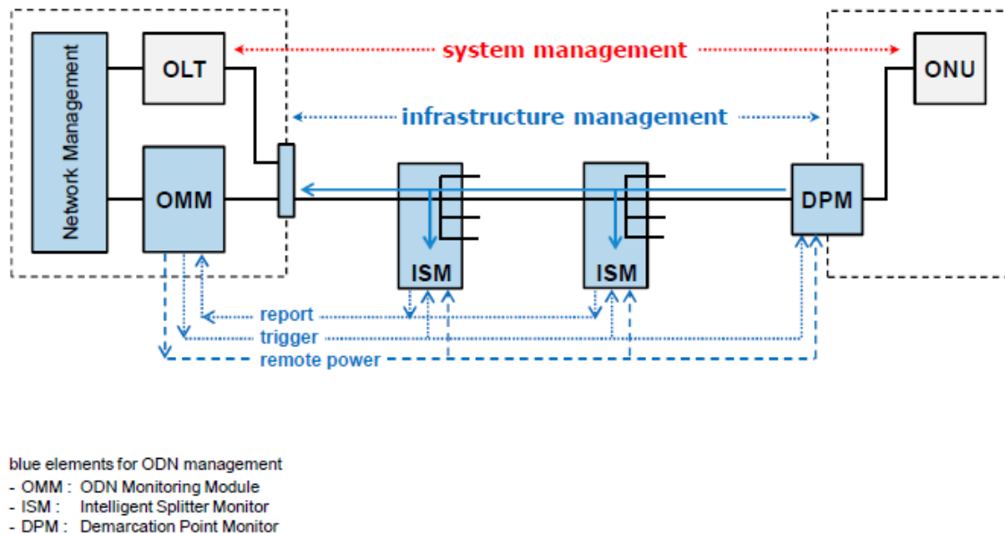
Fig. 4. A near term example of a managed infrastructure for FTTx. (Courtesy of Alcatel-Lucent)
