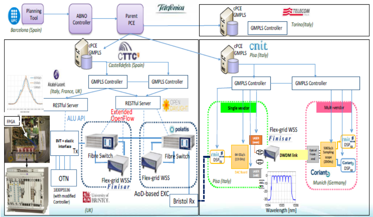
Fig. 2. Pan-european test-bed implemented within European FP7 project IDEALIST. (Courtesy of IDEALIST project).
