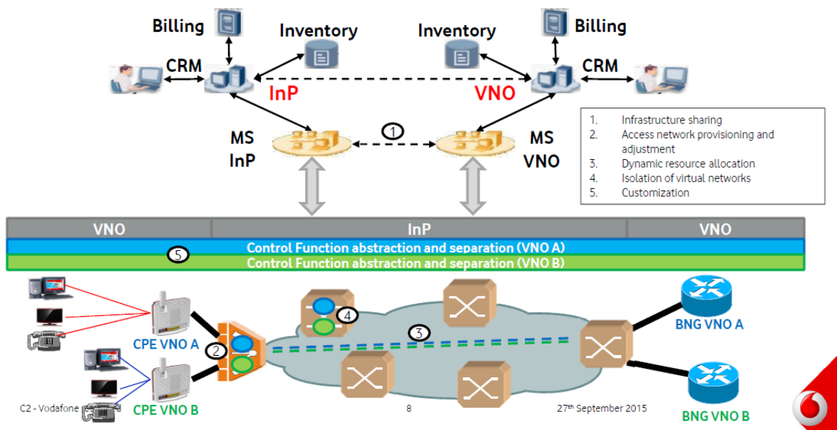
Fig. 3. End-to-end architecture of Fixed Access Network Sharing scenario. (Courtesy of Vodafone)
