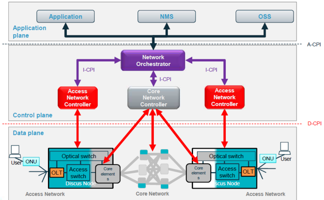
Fig. 7. DISCUS SDN/NFV control plane architecture.
