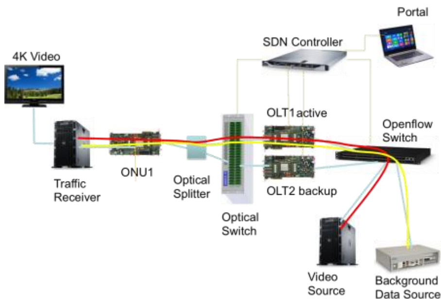
Fig. 8. Schematic of portable DISCUS Demo shown at ECOC Exhibition 2015.
