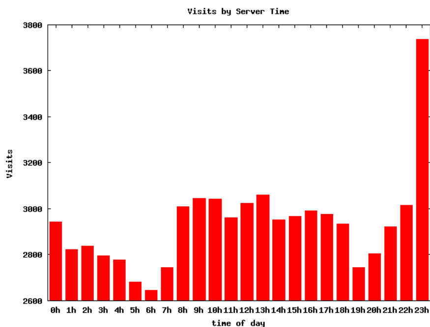
Figure 2.1: Visits by server time
