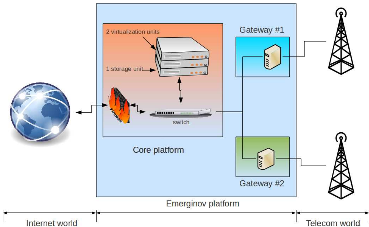
Illustration 1: Organic architecture
