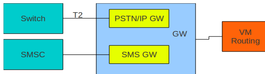
Illustration 4: Gateway description
