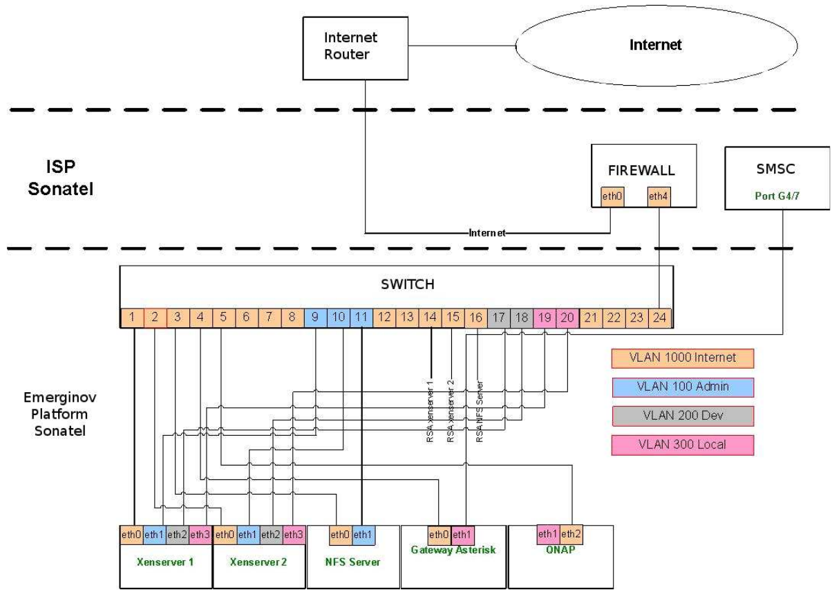
Illustration 3: Technical architecture
