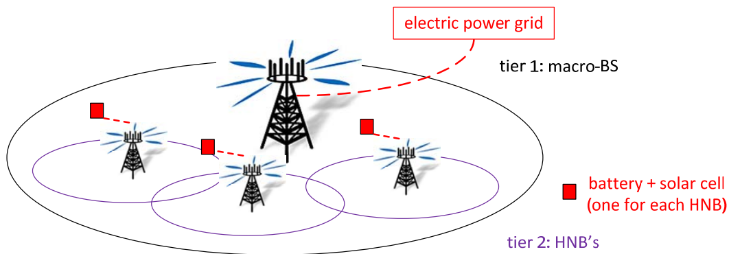
Figure 1. Scenario based on a 2-tier network. Tier 1: one macro-BS connected to the electrical power grid, tier 2: several HNBs placed generally at different locations, each one with its own battery and solar cell. The coverage areas of the HNBs overlap with the coverage area of the macro-BS.
