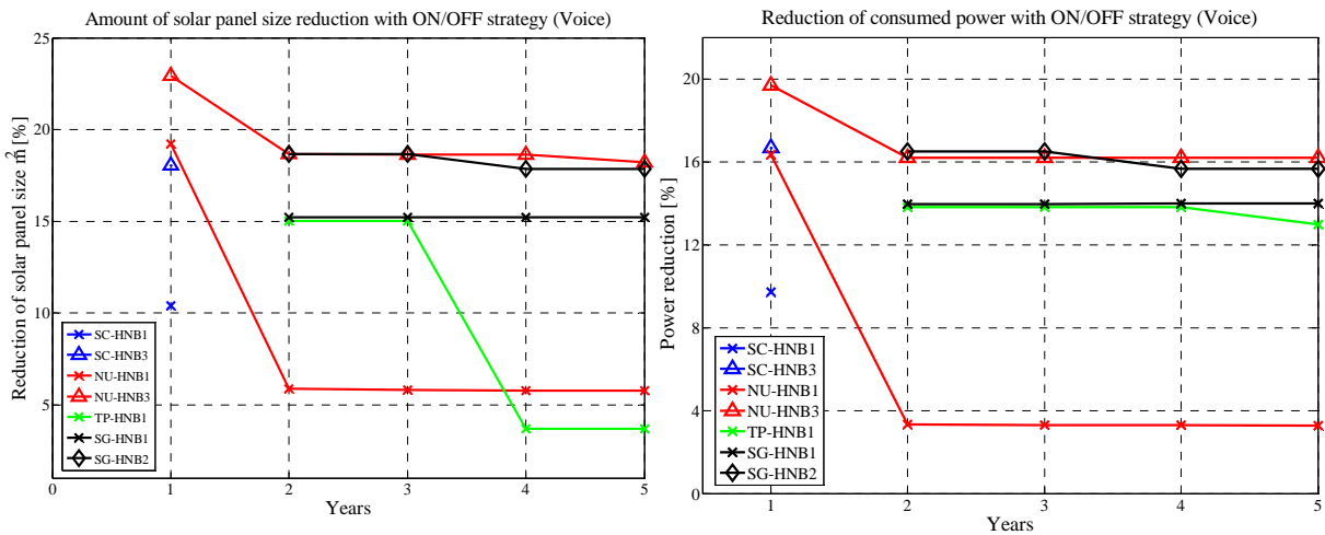
Figure 6. Left figure: amount of solar panel size reduction after on-off strategy. Right figure: amount of power reduction after on-off strategy. Results are given in percentage terms, where they are being
