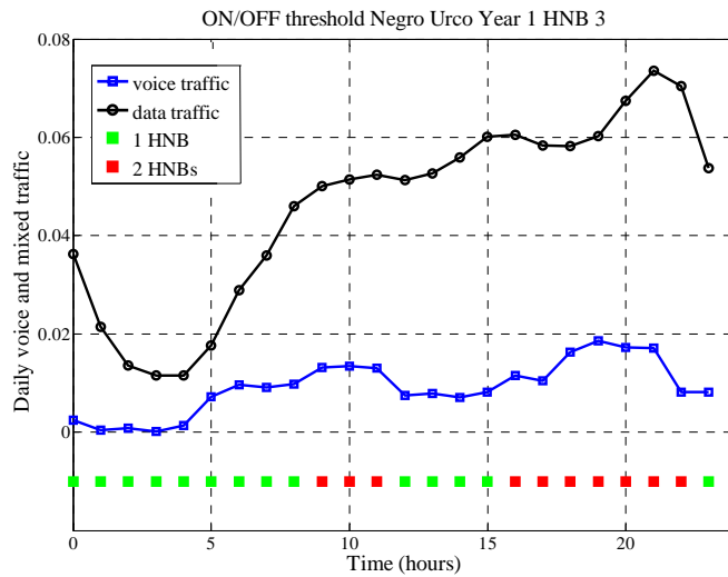
Figure 8. Daily traffic evolution and on-off strategy
