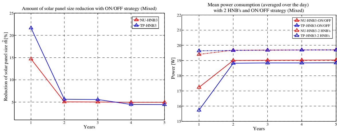
Figure 9. Left figure: amount of solar panel size reduction after on-off strategy. Right figure: amount of power consumed by scenario with 2 HNBs active and after on-off strategy
