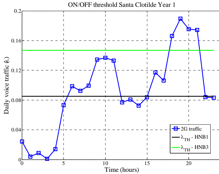
Figure 5. Daily traffic evolution with lambda threshold depicted
