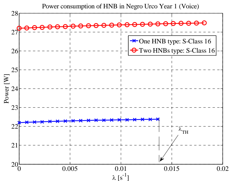
Figure 4. Computation of lambda threshold for a single type of traffic
