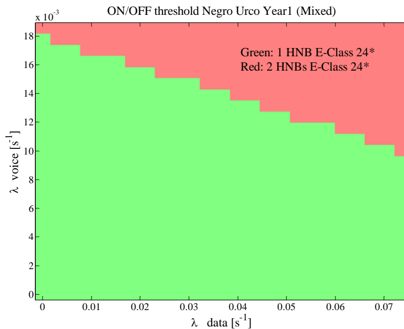
Figure 7. Computation of lambda threshold for two types of simultaneous traffic
