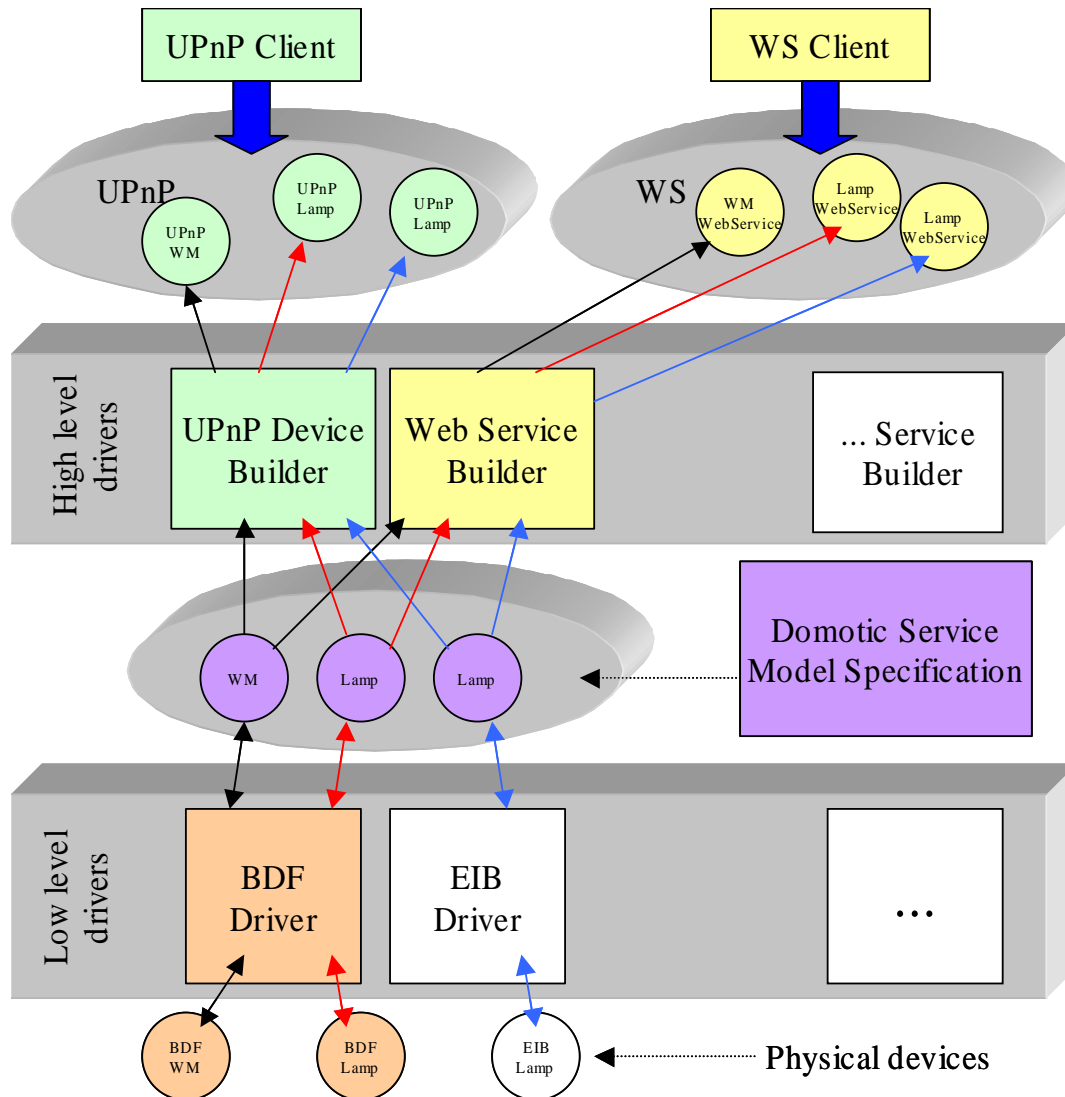
Figure 4-1: The Amigo Domotic Infrastructure
