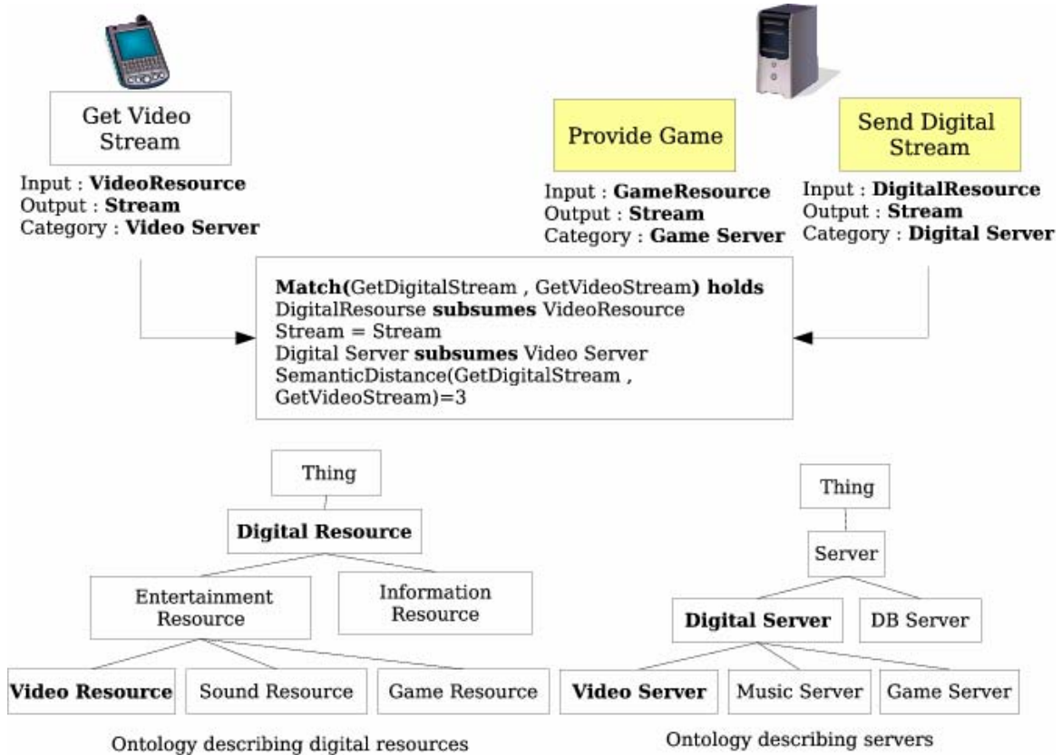
Figure 4-5 Describing and matching capabilities of services
