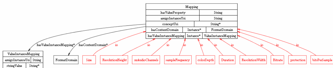
Figure 3-5: The Mapping ontology
