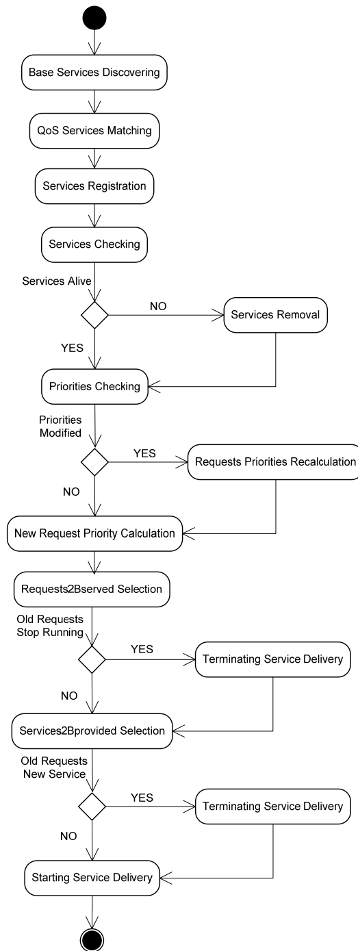
Figure 4-12: The Service Selection process state diagram for outdoor services
