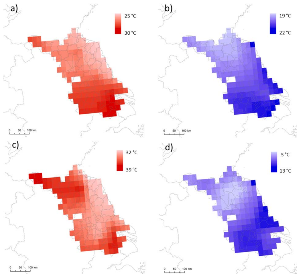
Figure 5 Daily maximum (a) and minimum (b) temperature averaged out from June to October 2006. Maximum value reached by daily maximum temperature (c) and minimum value reached by daily minimum temperature (d) from June to October 2006.
