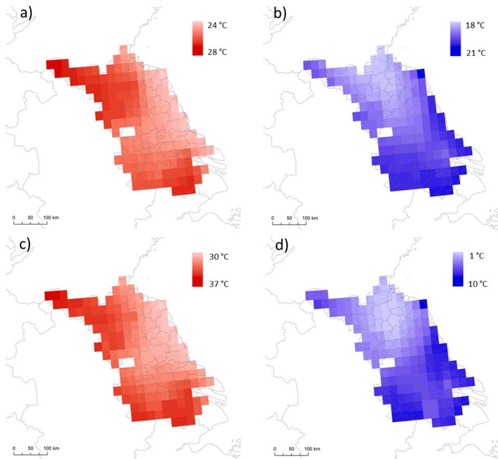
Figure 4 Daily maximum (a) and minimum (b) temperature averaged out from June to October 1999. Maximum value reached by daily maximum temperature (c) and minimum value reached by daily minimum temperature (d) from June to October 1999.
