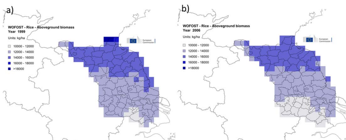
Figure 9 Maximum value of aboveground biomass simulated by WOFOST in: a) 1999 growing season; b) 2006 growing season. Grid cell resolution is about 25×25 km
