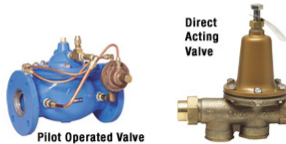
Figure 13 Direct Acting Valve and Pilot Operated Valve for reducing pressure in a water distribution network (www.watts.com)
