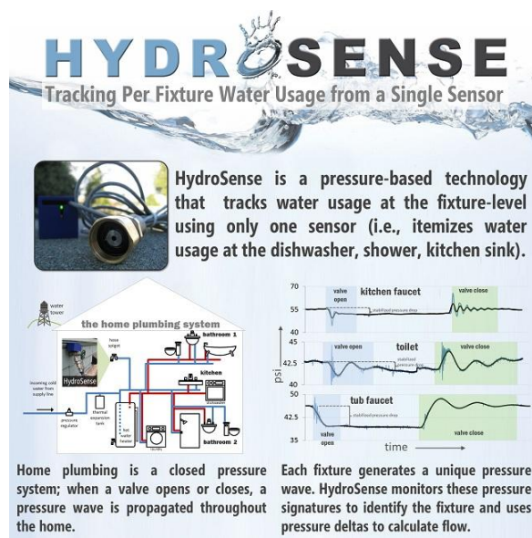
Figure 5: HydroSense 24 technology
