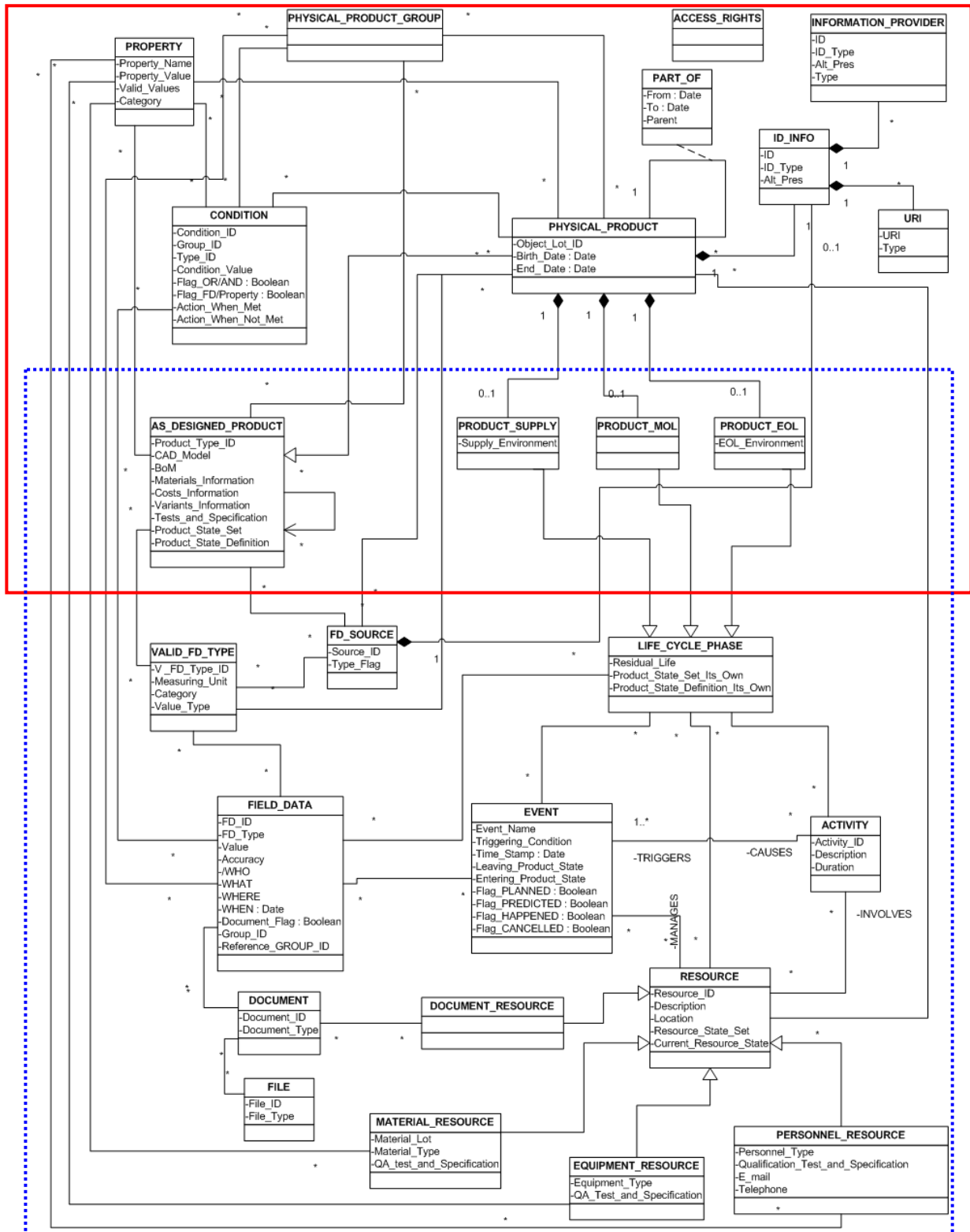
Figure 10: Complete schema of the semantic object model
