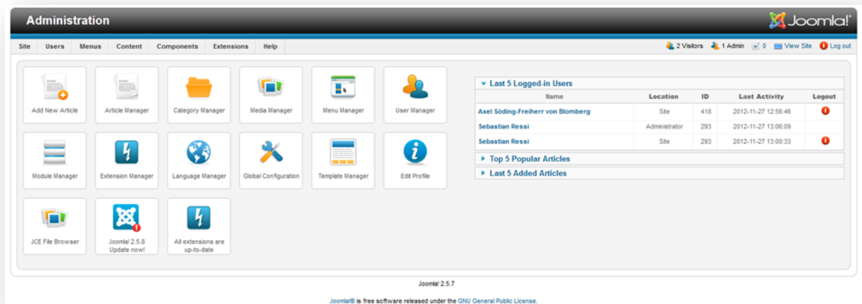
Figure 4: Backend
