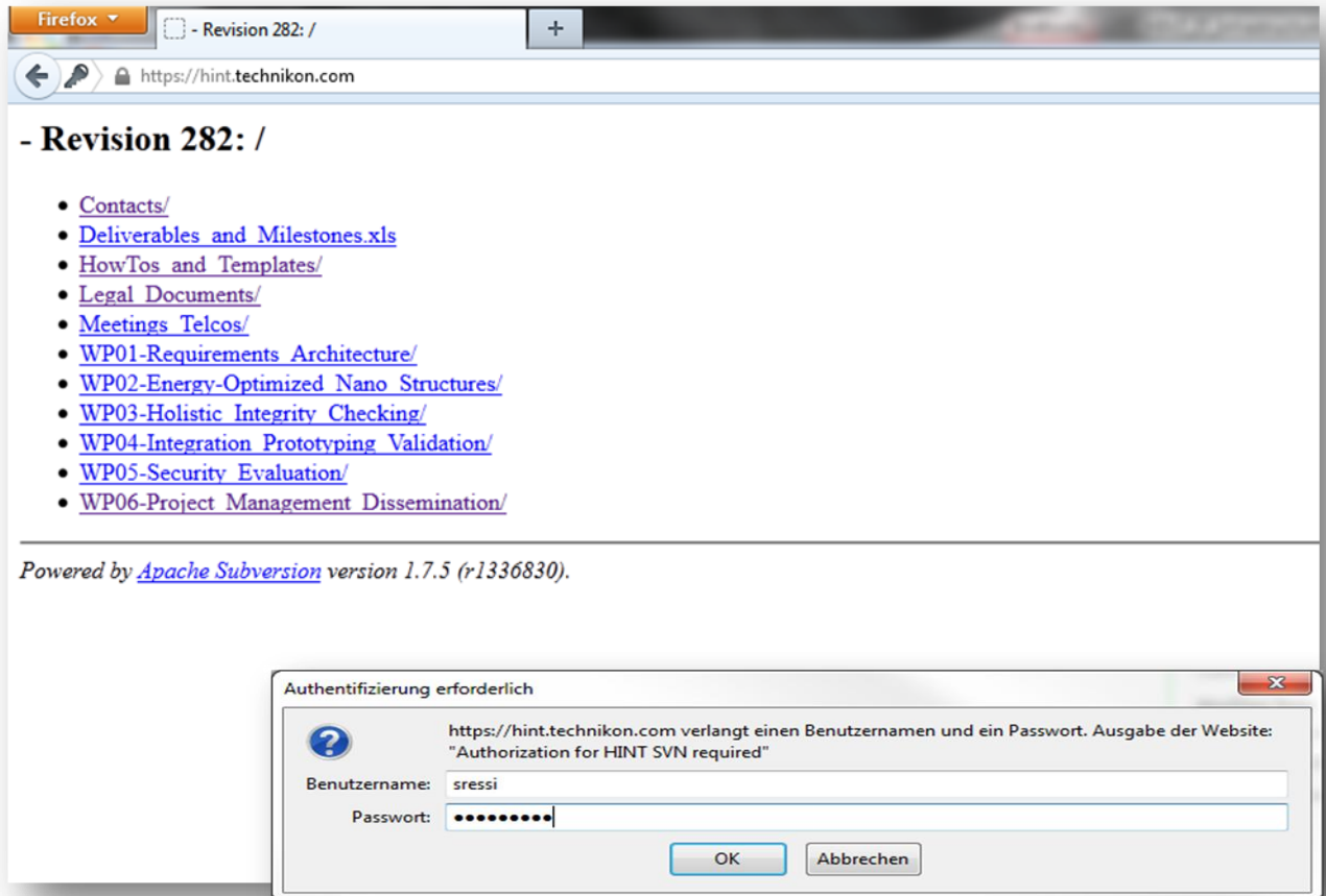
Figure 13: Browser access
