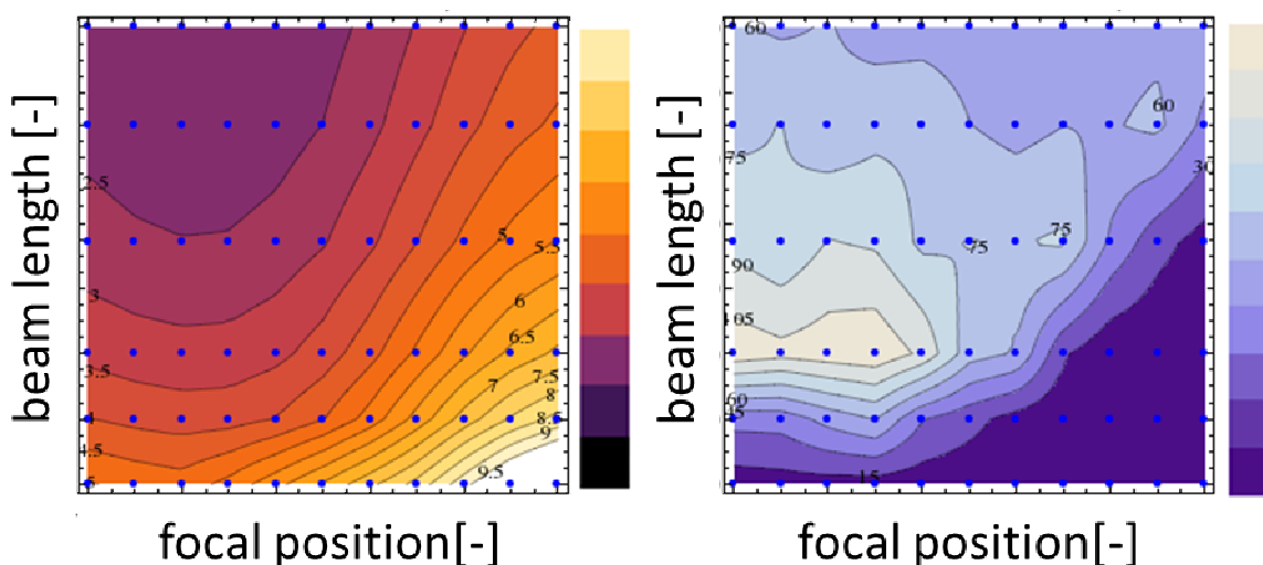
Figure 10: Inclination (left, 0-10°) of the cutting front and roughness (right, 0-150 \mu\text{m} ) of the resulting cut surface as functions of beam length at focus parallel to the cutting direction and its focal position. By visual exploration of the Process Maps generated by the Meta-Model of sheet metal cutting the concept of elliptical beam shaping is refined.
