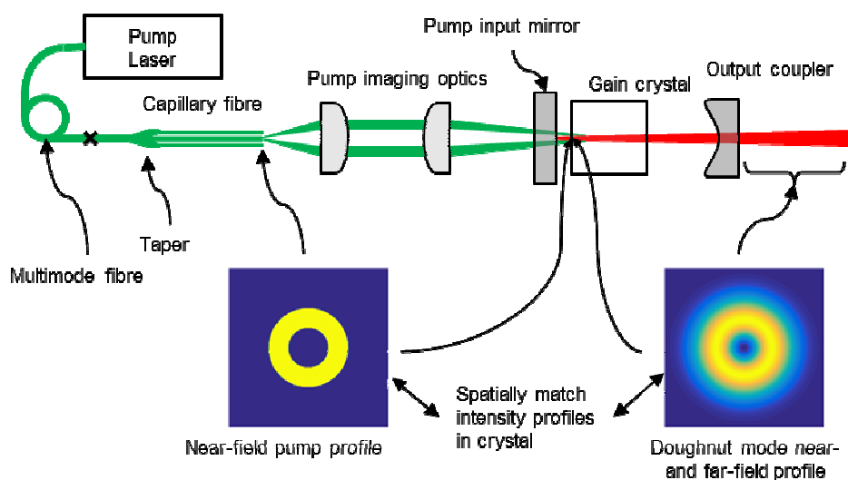
Figure 9: Schematic of ORC hybrid laser design
