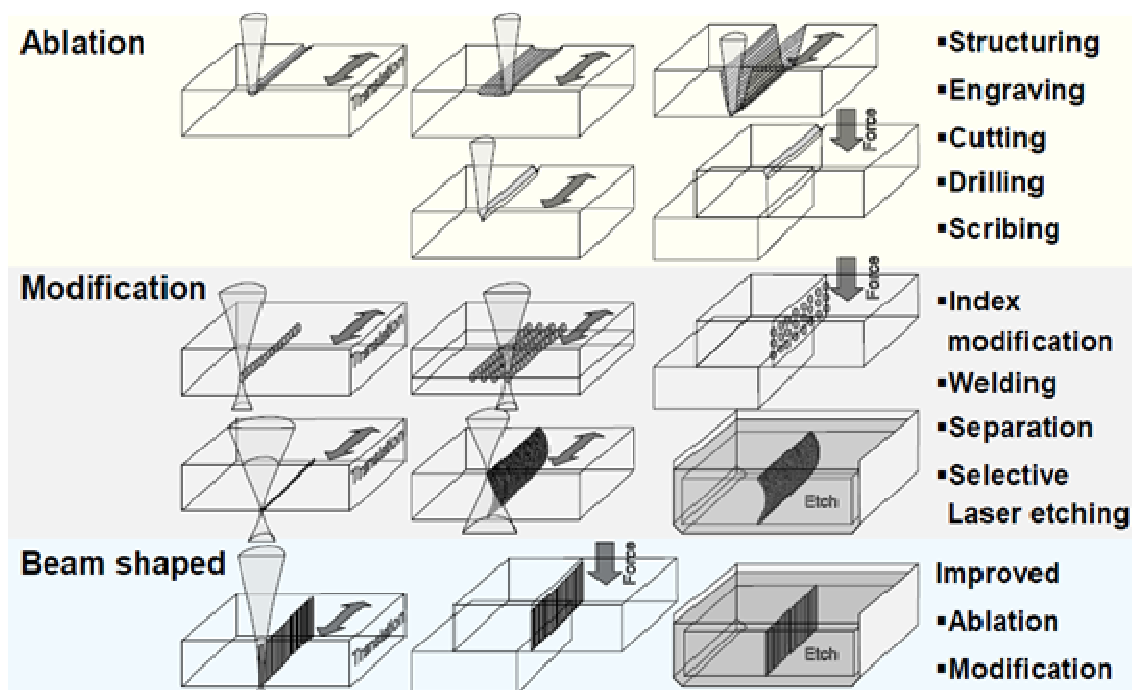
Figure 16: Schematic of different glass cutting methods
