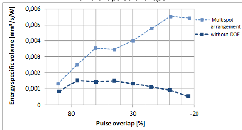
Figure 20: Graph showing the energy specific volume of processes with and without optimised multi-spot arrangement at different pulse overlaps.
