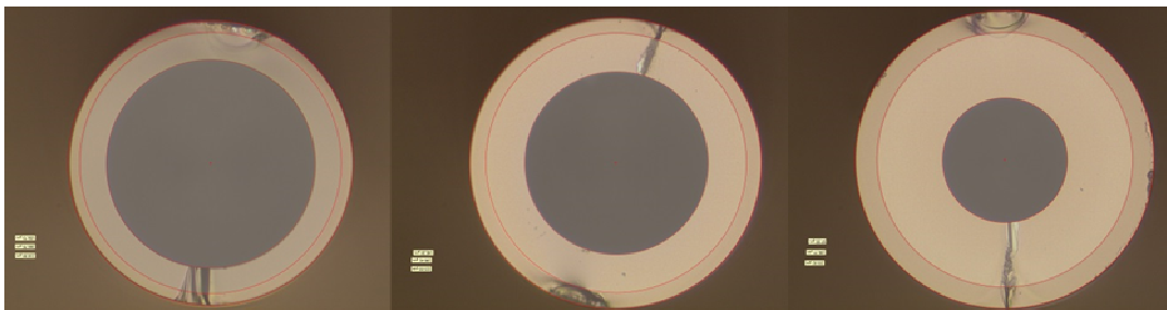
Figure 2: Cleaved capillary fibres with different aspect ratios
