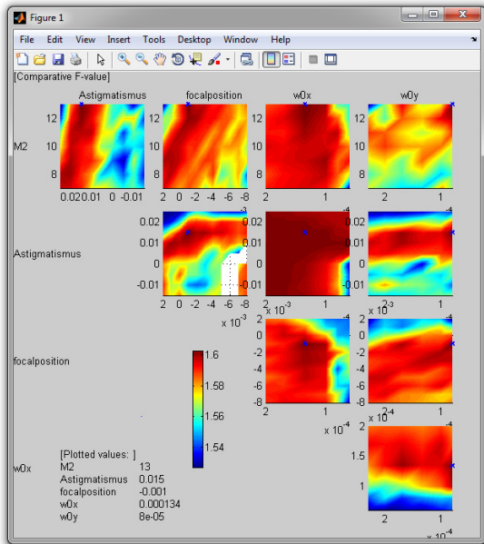
Figure 14: Example of optimisation results (roughness variation across part of the parameter space) from the physical model for a specific laser cutting case and system
