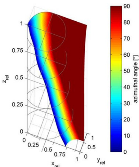
Figure 23: 3D model of cutting kerf
