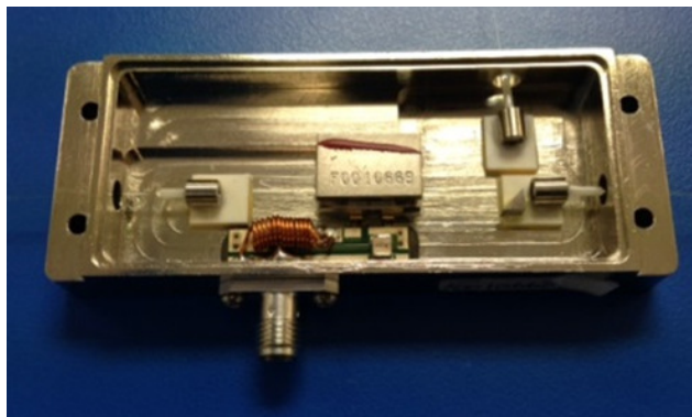
Figure 4: 3-port acousto-optic fibre switch
