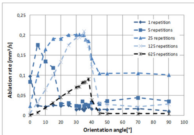
Figure 18: Ablation rate of process with line arrangement at different angles relative to the feed rate direction.
