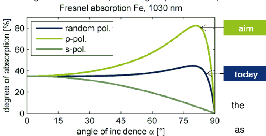
Figure 22: Absorption diagram for solid state lasers
