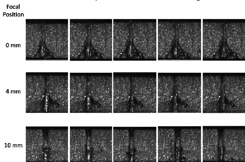
Figure 12: Time series with 1.5 ms interval for three different focal positions
