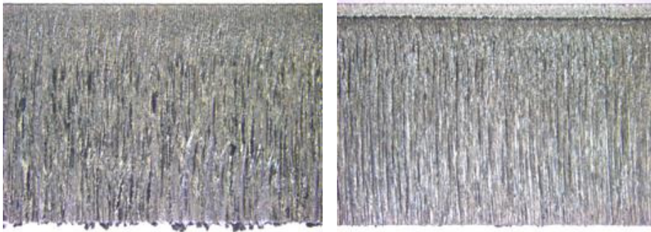
Figure 24: Cutting results in 15 mm stainless steel. Left: State-of-the-art with random polarisation showing dross at the bottom of the workpiece and rough surface finish Right: optimised polarisation showing no dross, improved surface quality: and performed at twice the feed rate!
