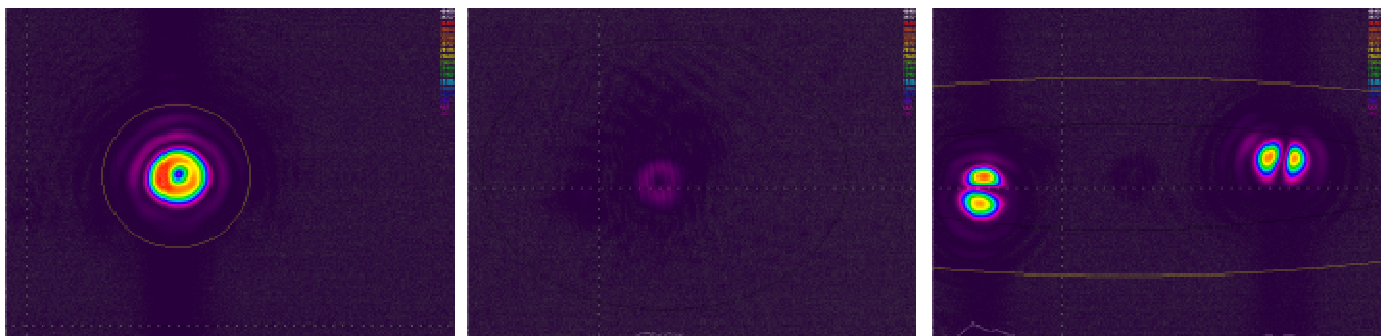
Figure 3: Left: Isolator input beam; Centre: Residual (unisolated beam). Right: Isolated beams showing decomposition of radially and azimuthally polarised LG01 modes into orthogonally polarised TEM_{10} and TEM_{01} modes.
