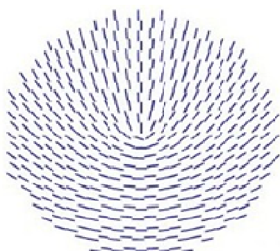
Figure 7: A schematic showing the orientation of nano-gratings in the ORC S-waveplate.
